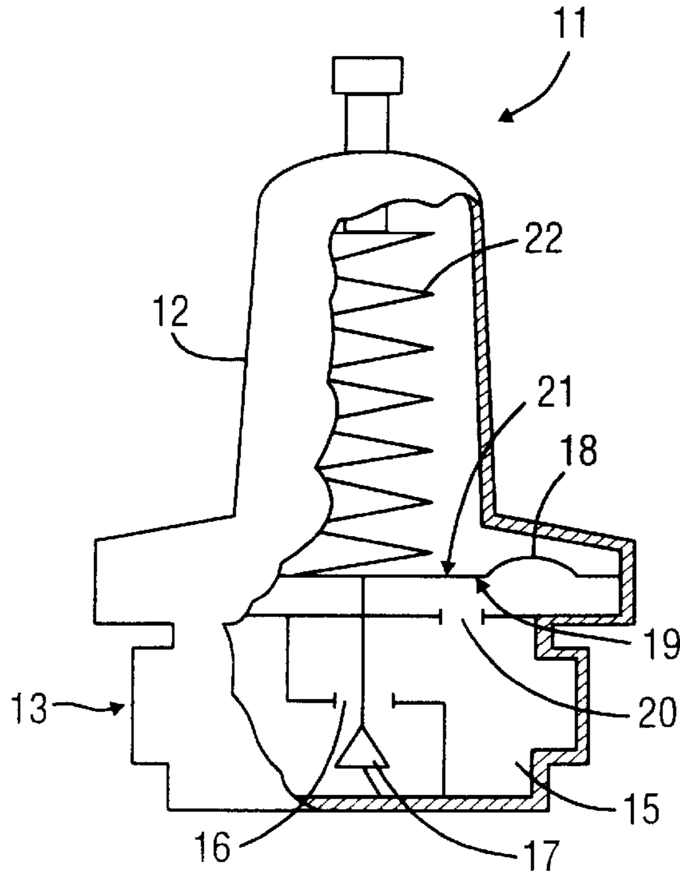
FIG. 1 (prior art)
