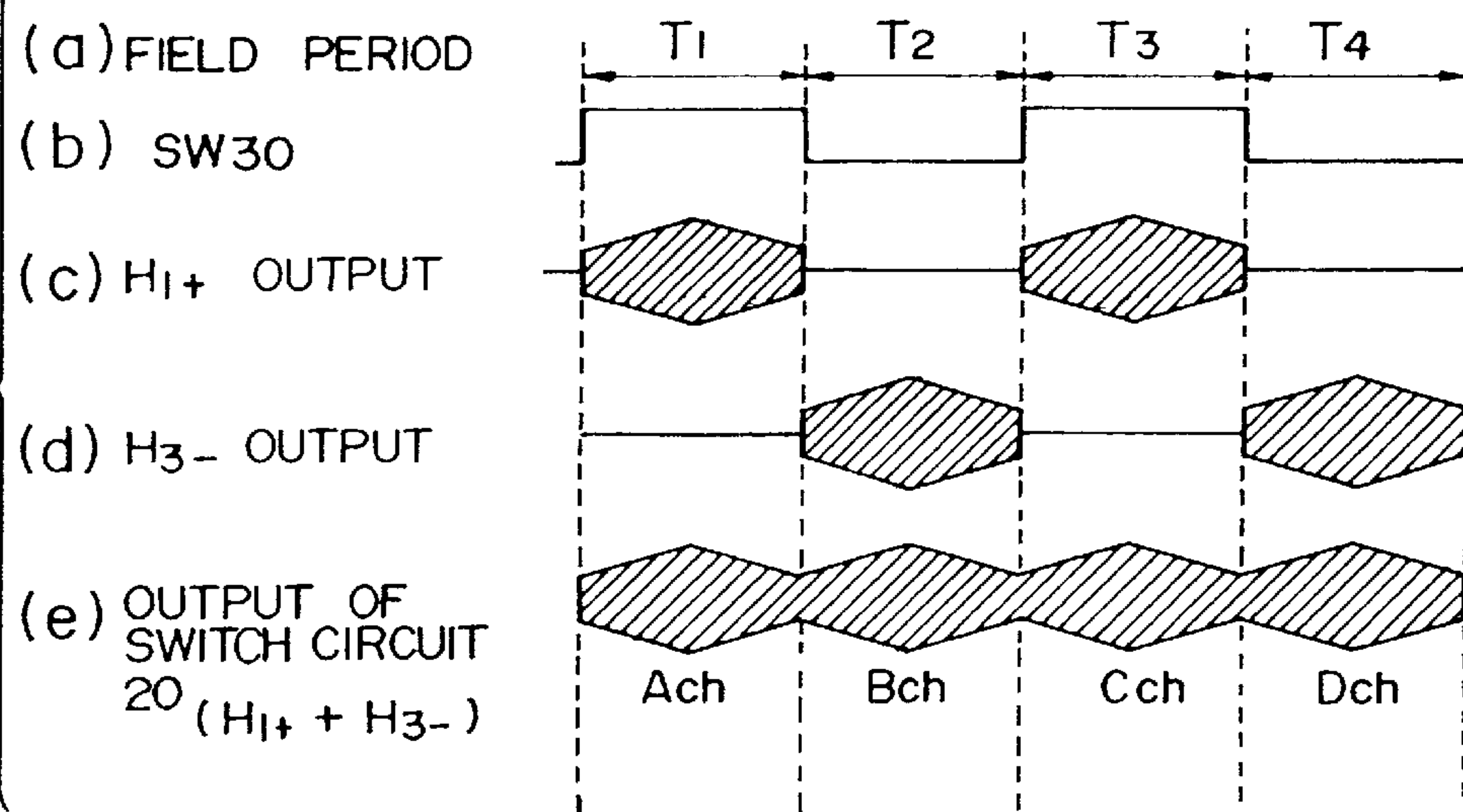
OPERATION DIAGRAM OF INTERMITTENT RECORDING AND NORMAL SPEED REPRODUCTION
