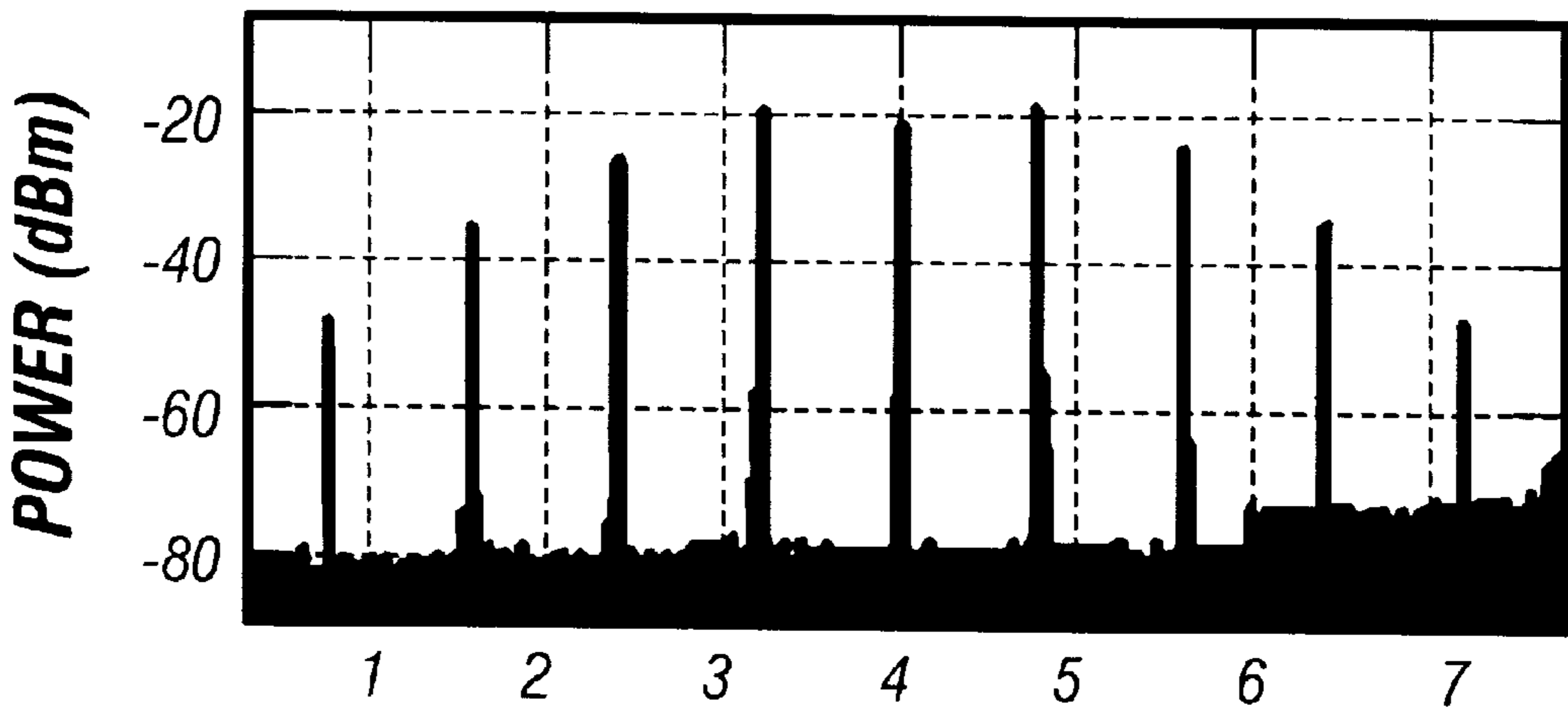
FREQUENCY (GHz) FIG. 9F
