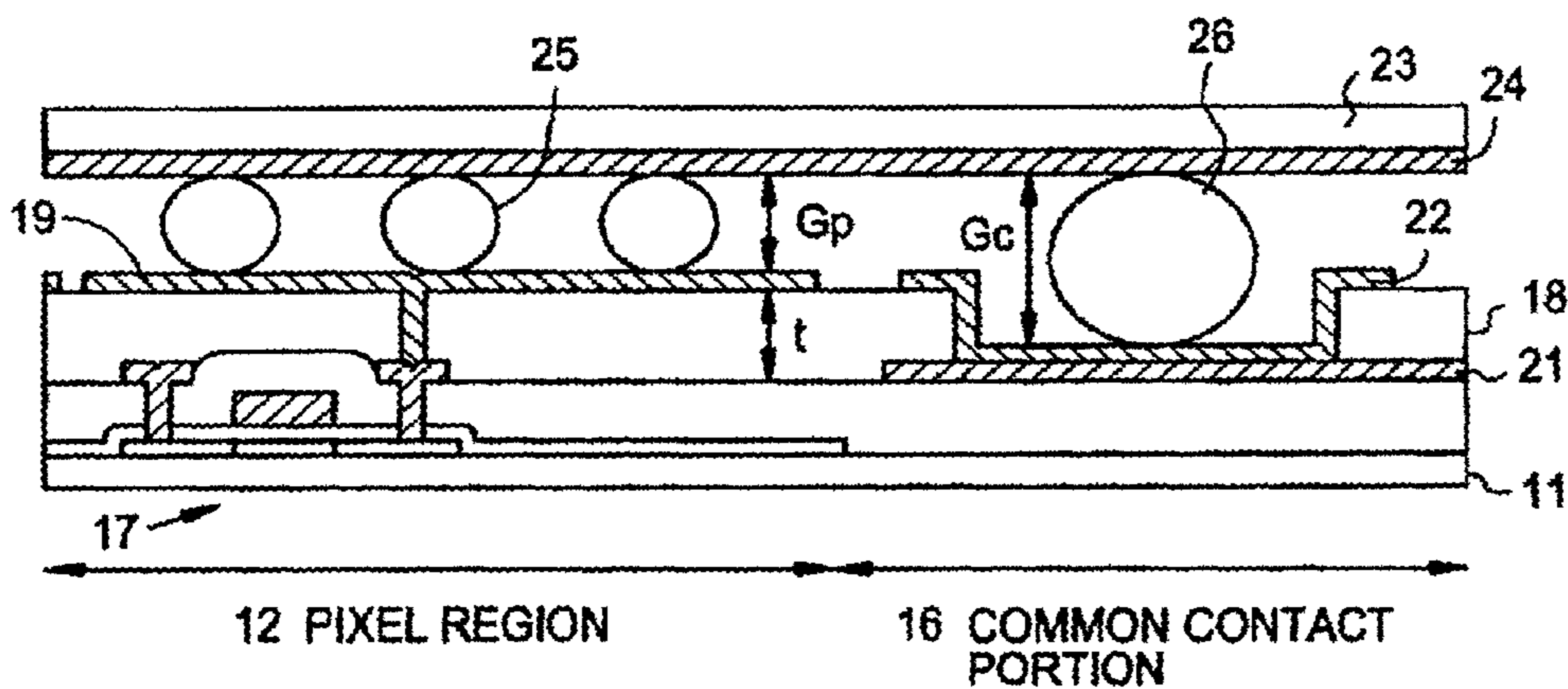
FIG.13 PRIOR ART
