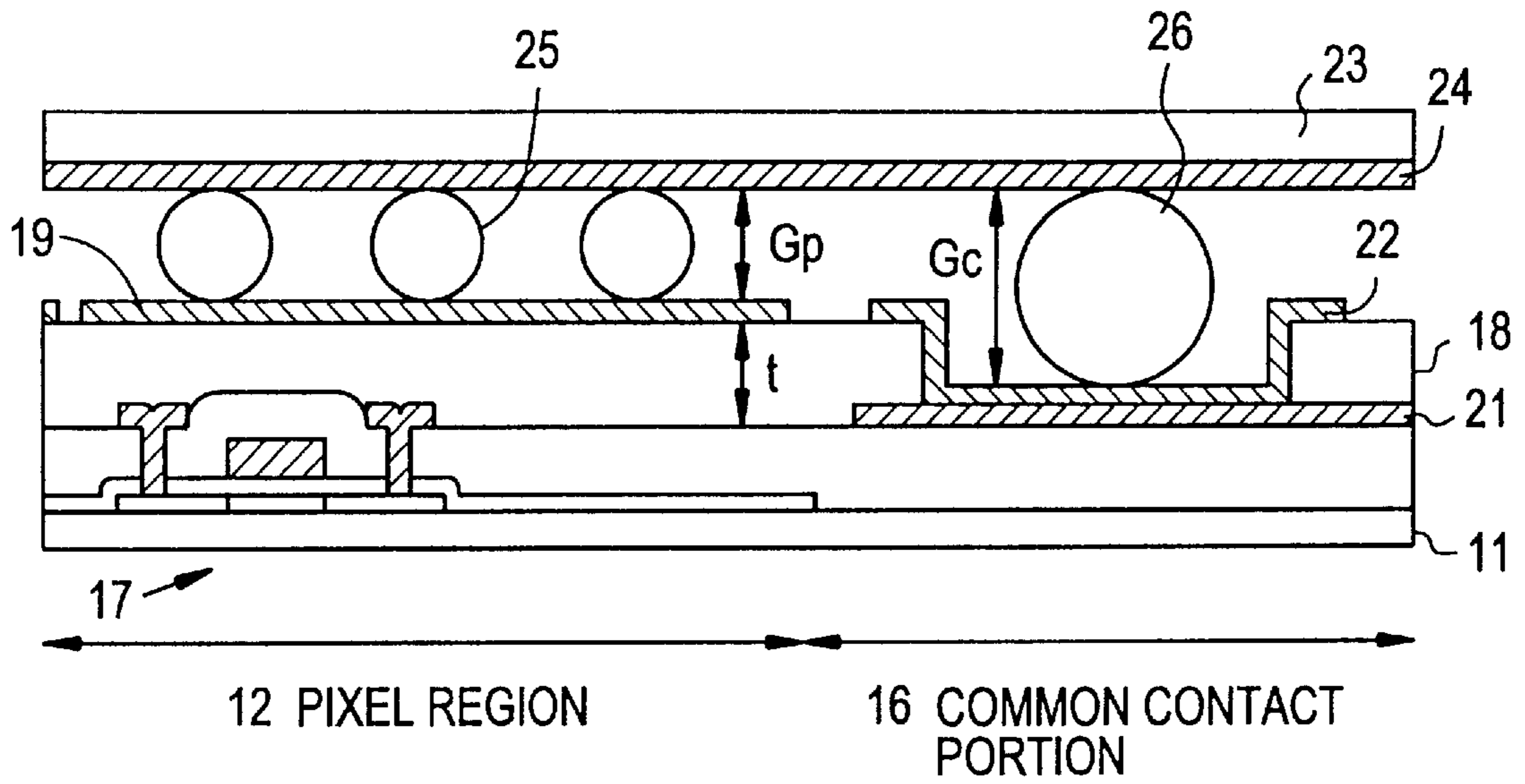
FIG. 13 PRIOR ART
