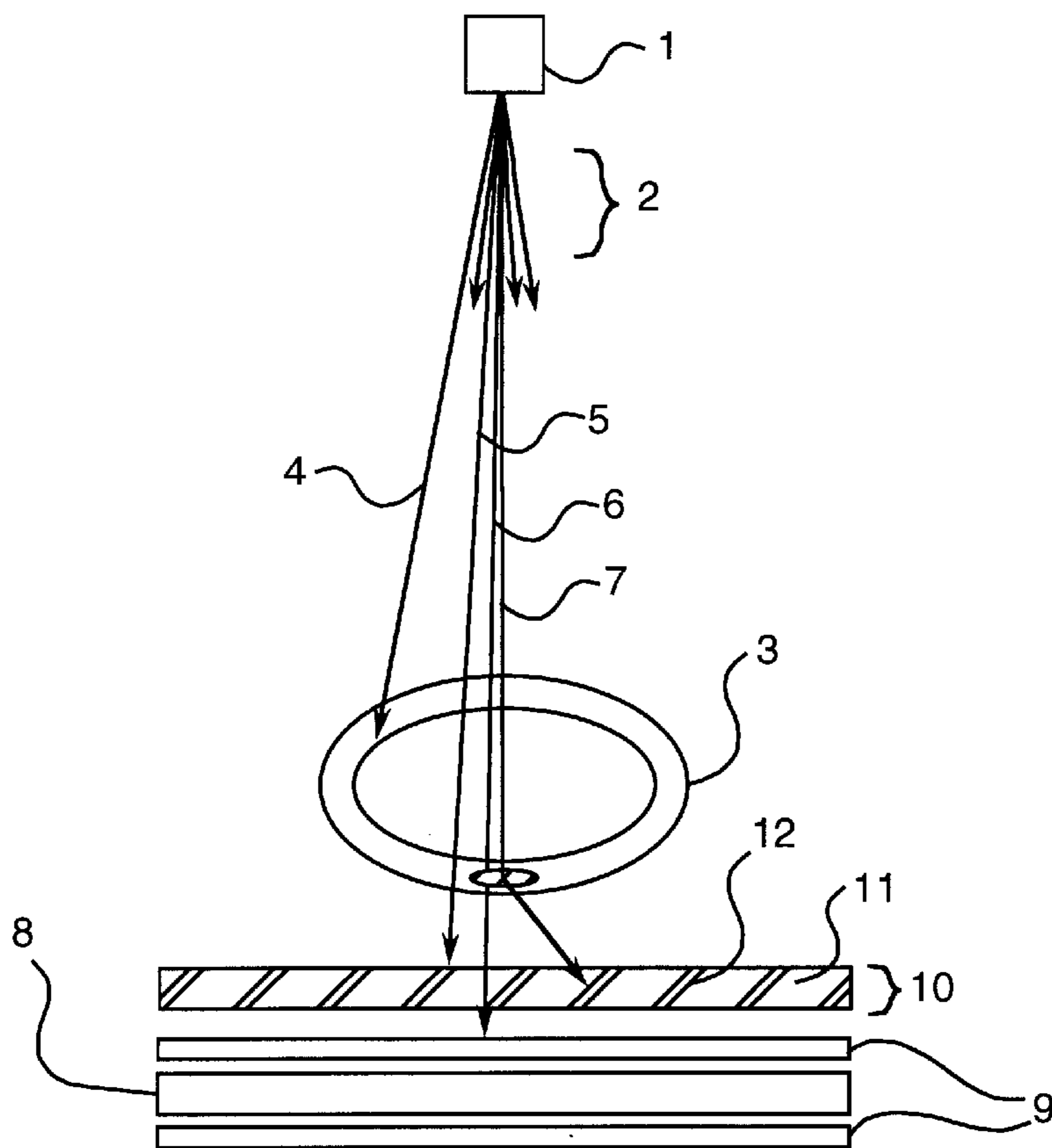
FIG. 1 (PRIOR ART)
