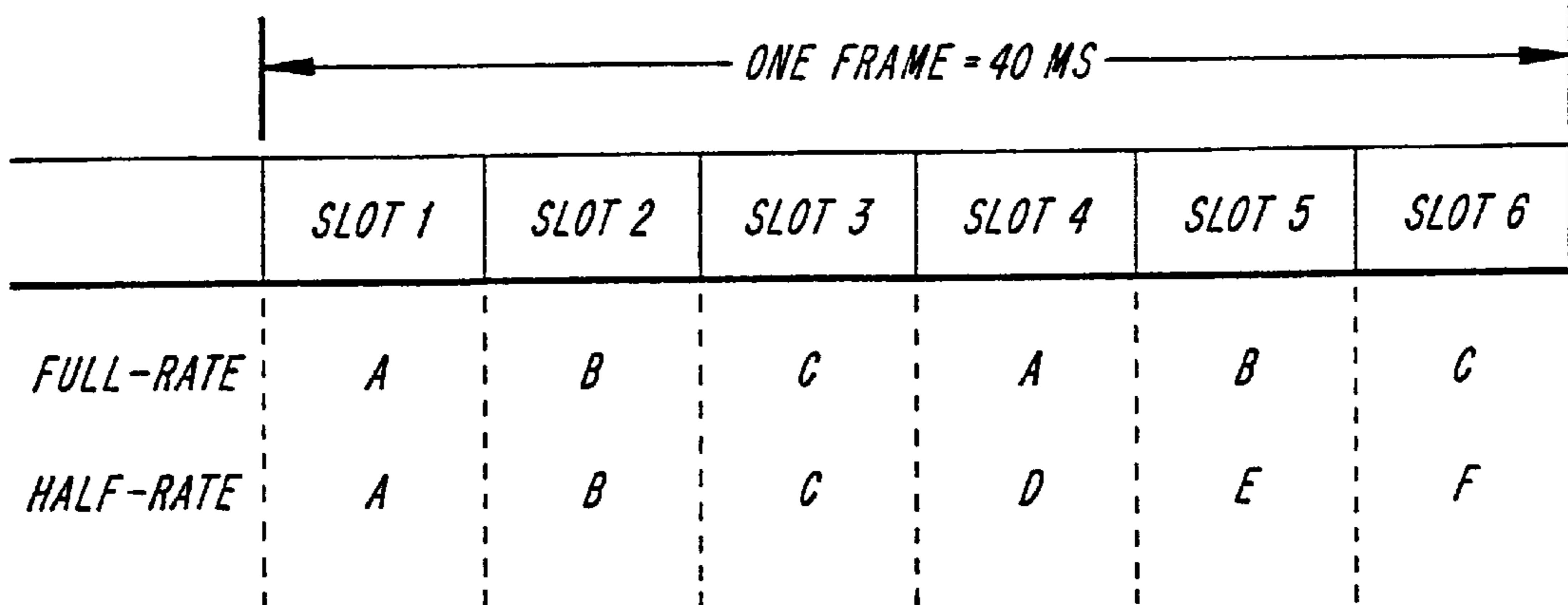
FIG. 4 PRIOR ART
