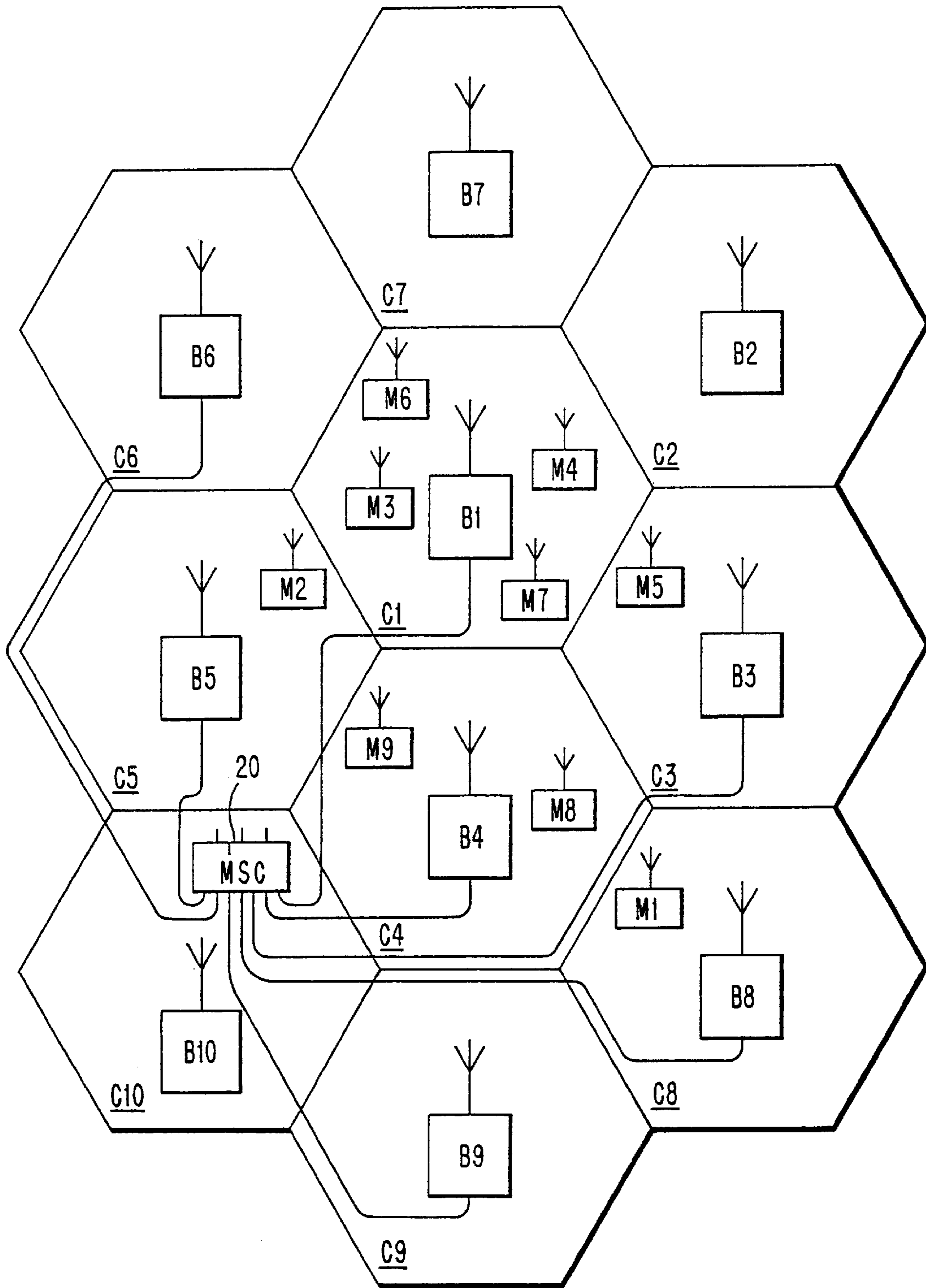
FIG. 1 PRIOR ART
