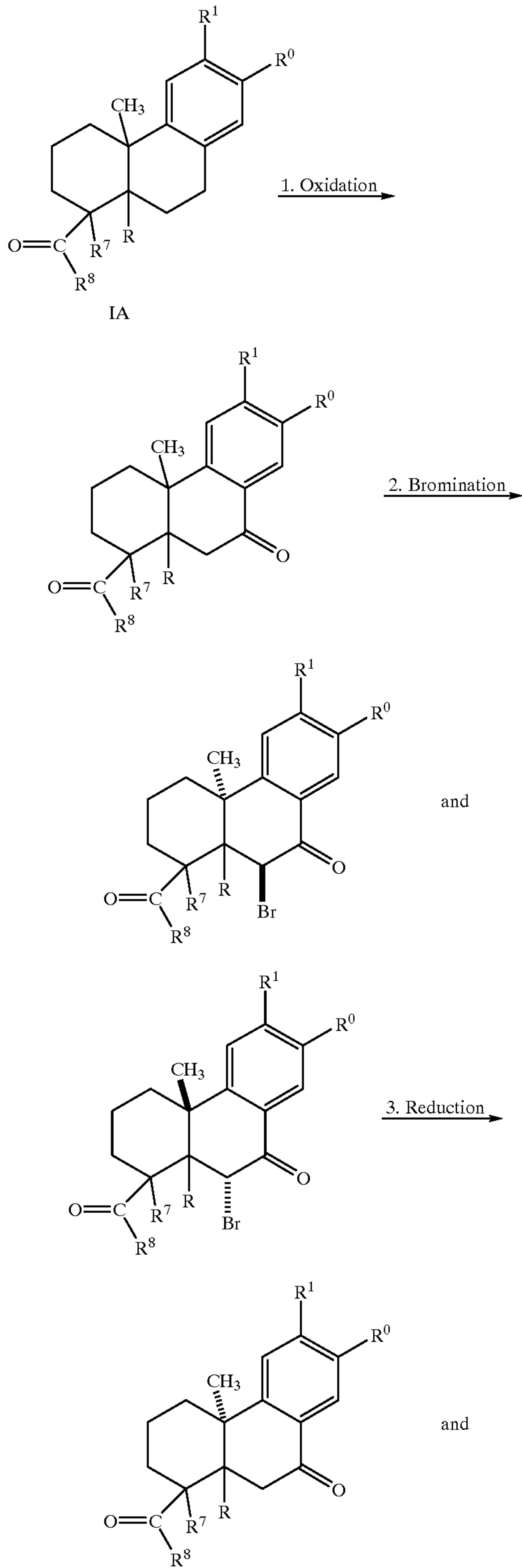
Reaction Scheme I
