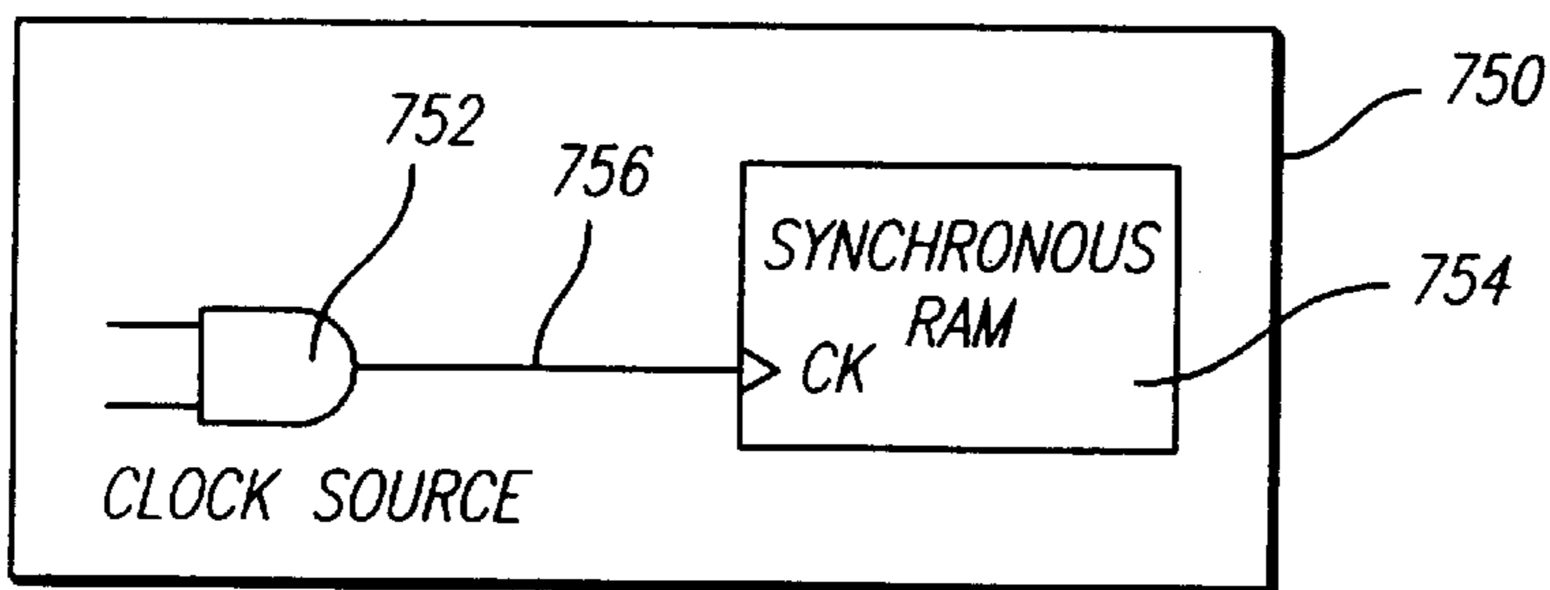
FIG. 41B CLOCK RETRIEVED THROUGH USING A CONNECTED CLOCK INPUT PIN ON A RAM
