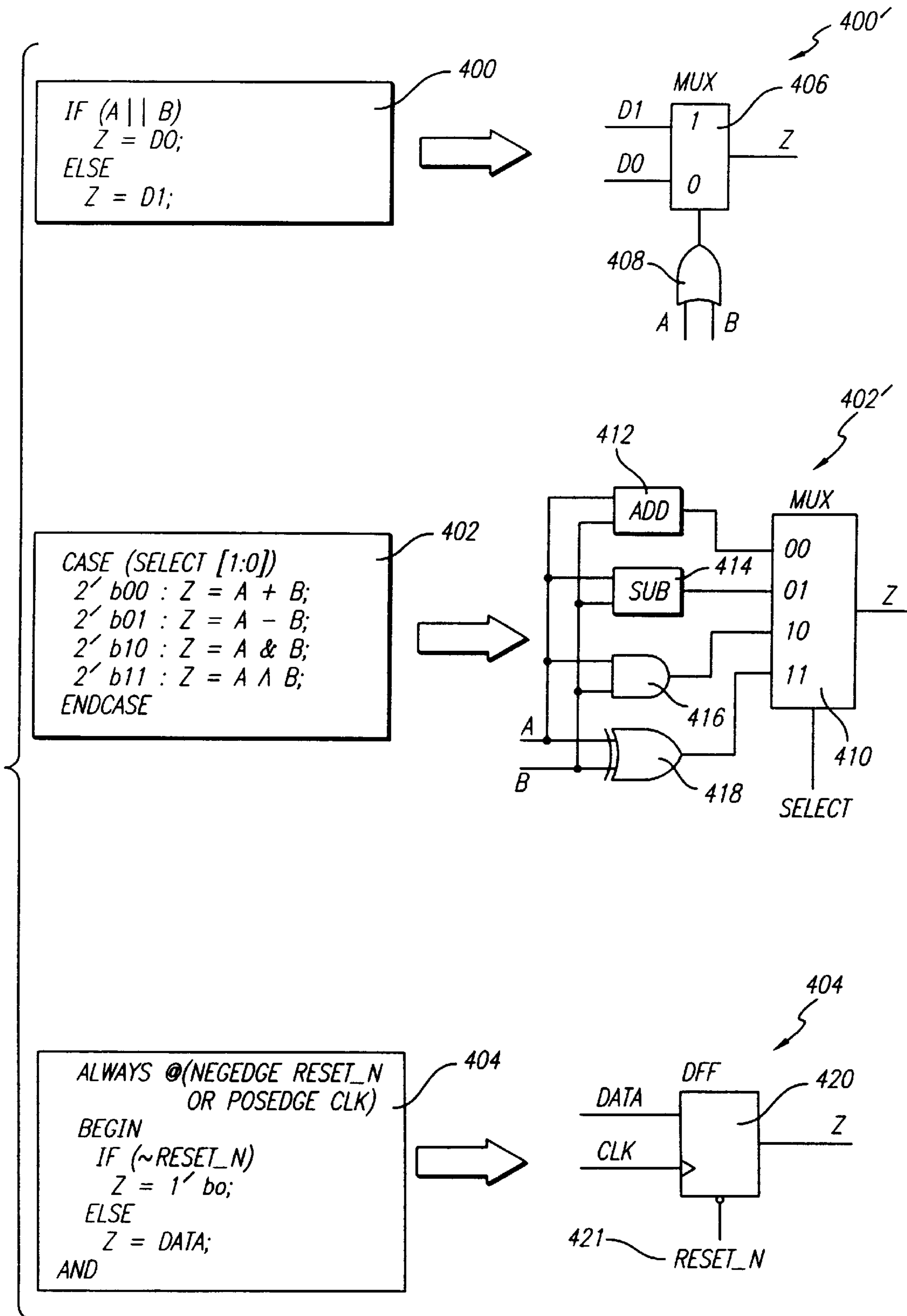
FIG. 38 EXAMPLES OF TRANSFORMS USED FOR RTL CODE TRANSLATION
