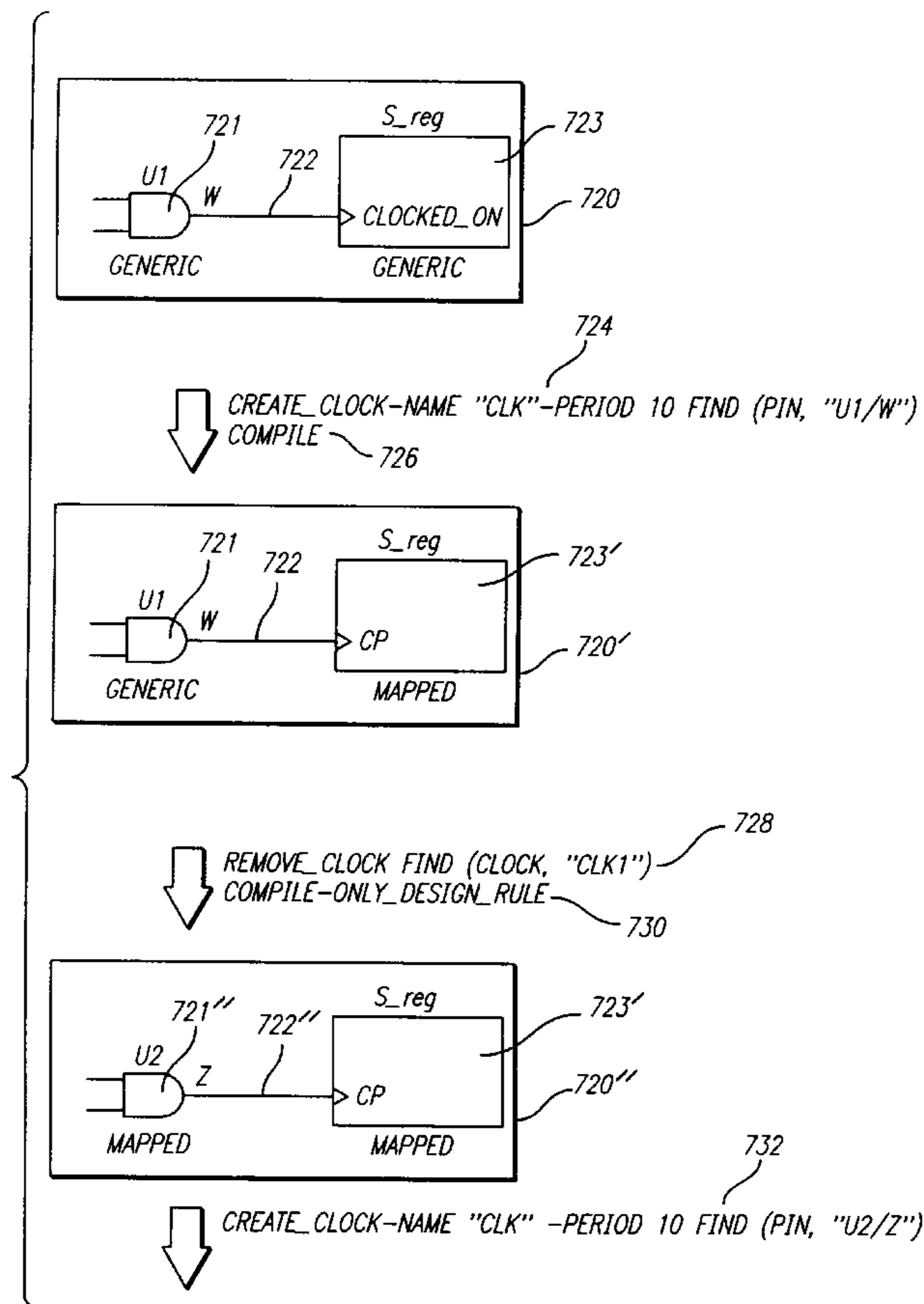
PROCESS USED TO MAP CELLS THAT CREATE INTERNAL CLOCKS.
