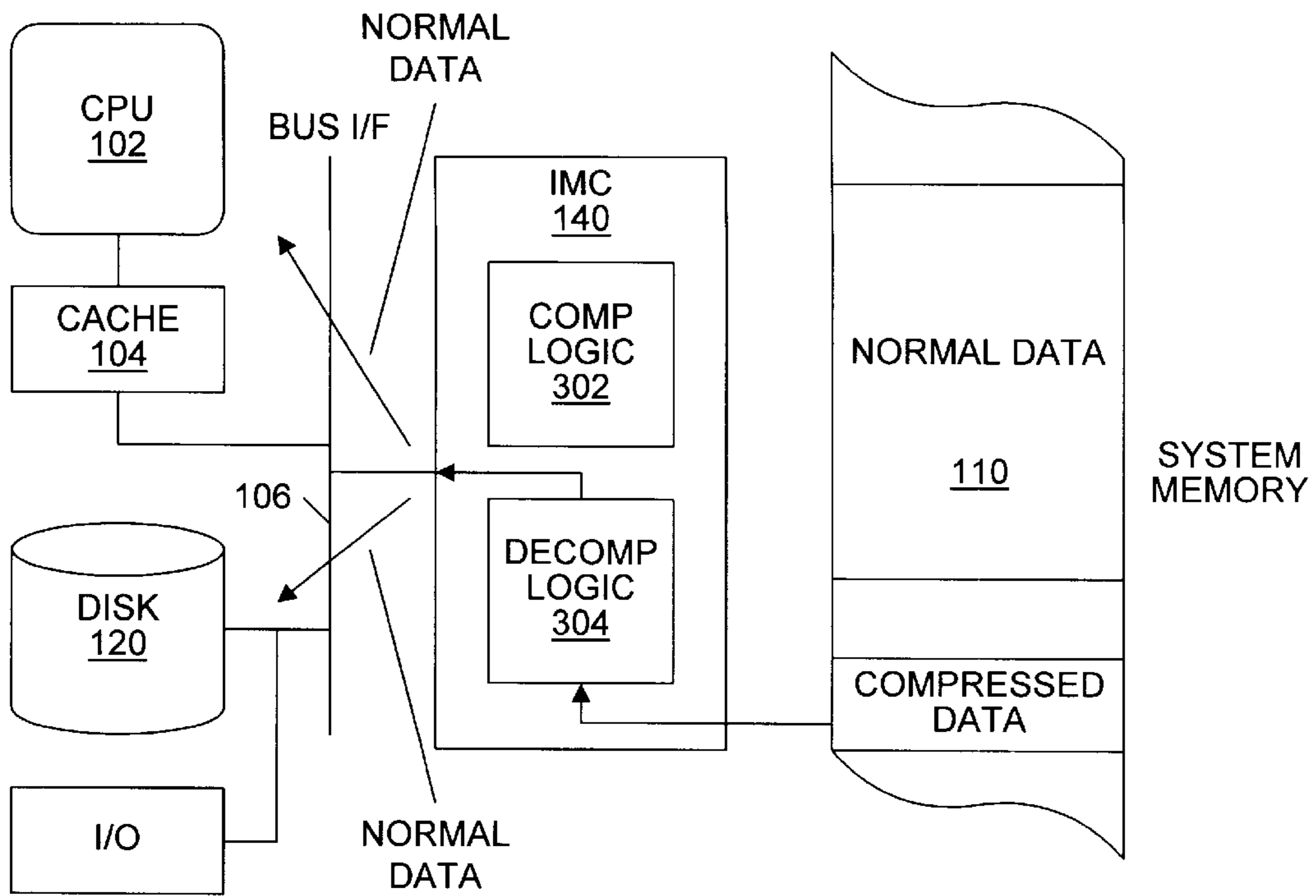
Memory decompression to CPU or Disk
