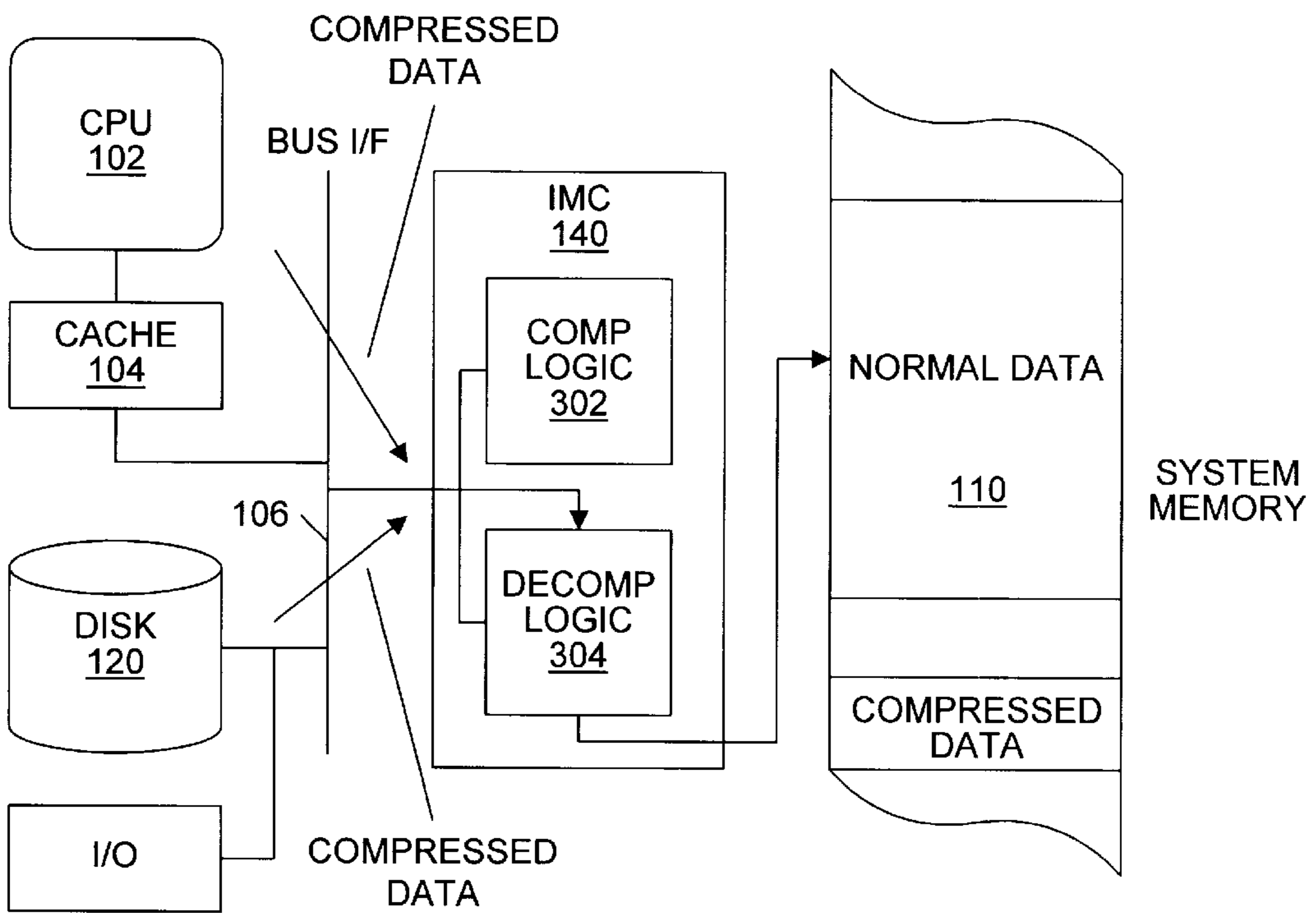
Decompression from Disk or CPU to memory
