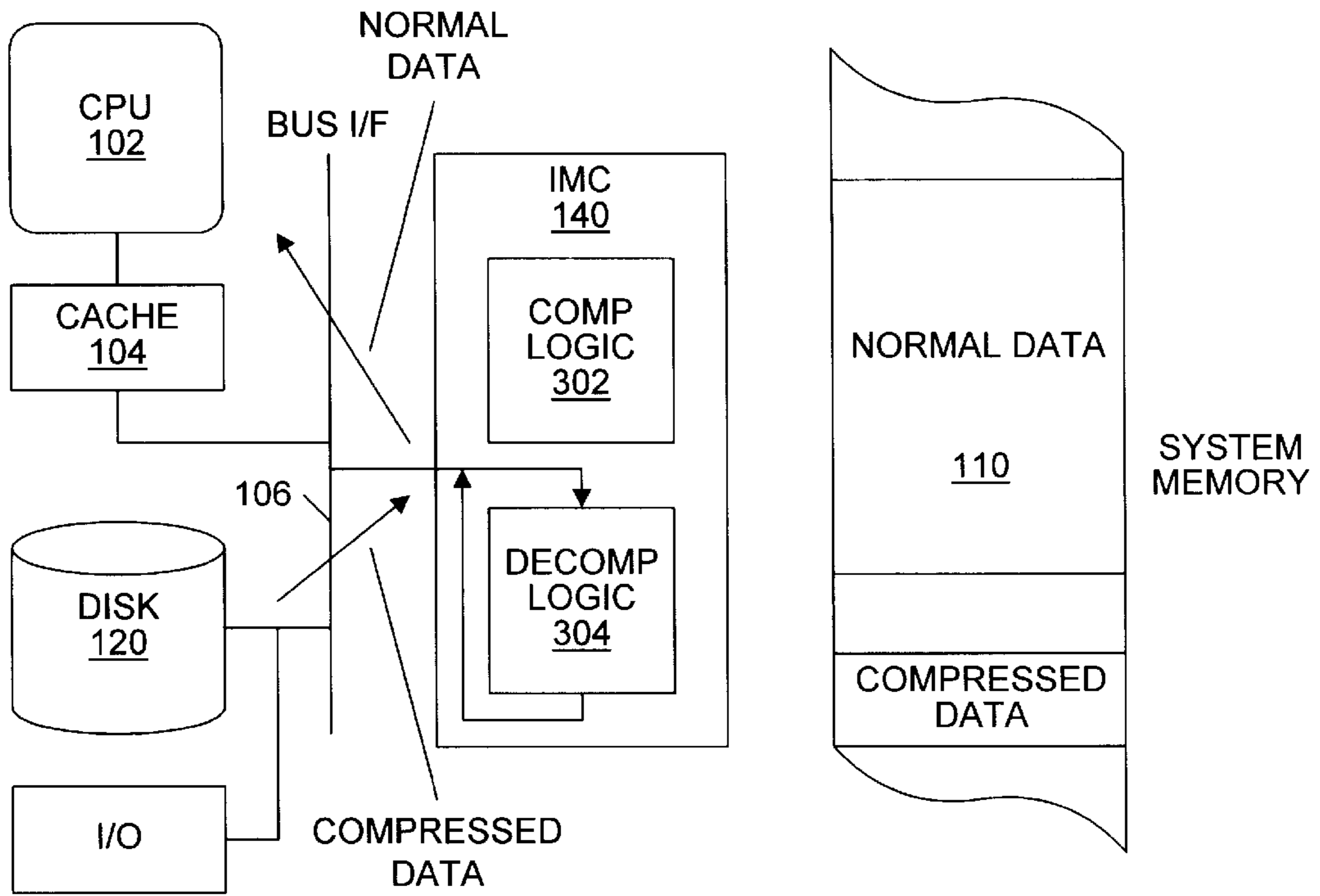
Decompression of disk to CPU
