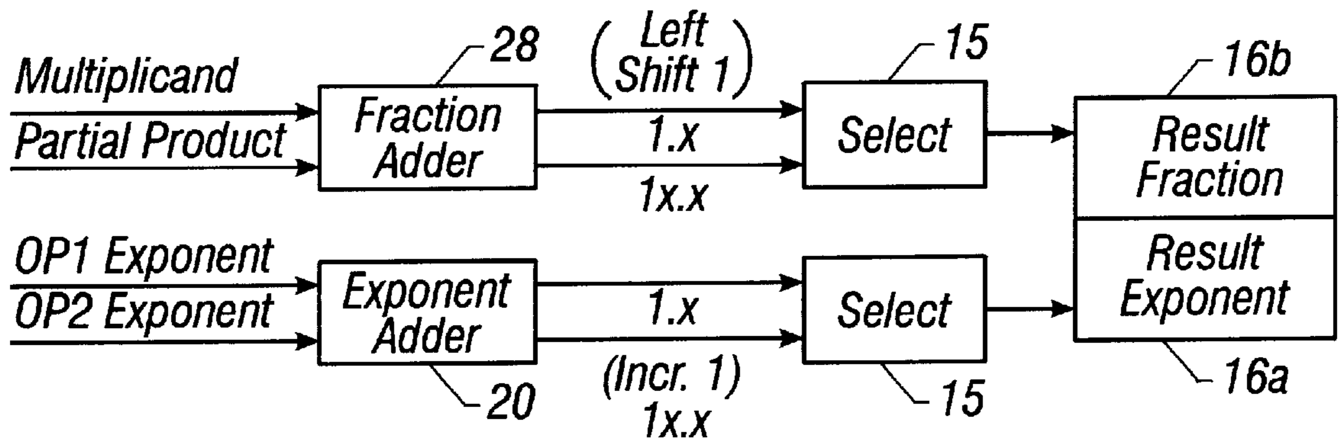
FIG. 3 (Prior Art)
