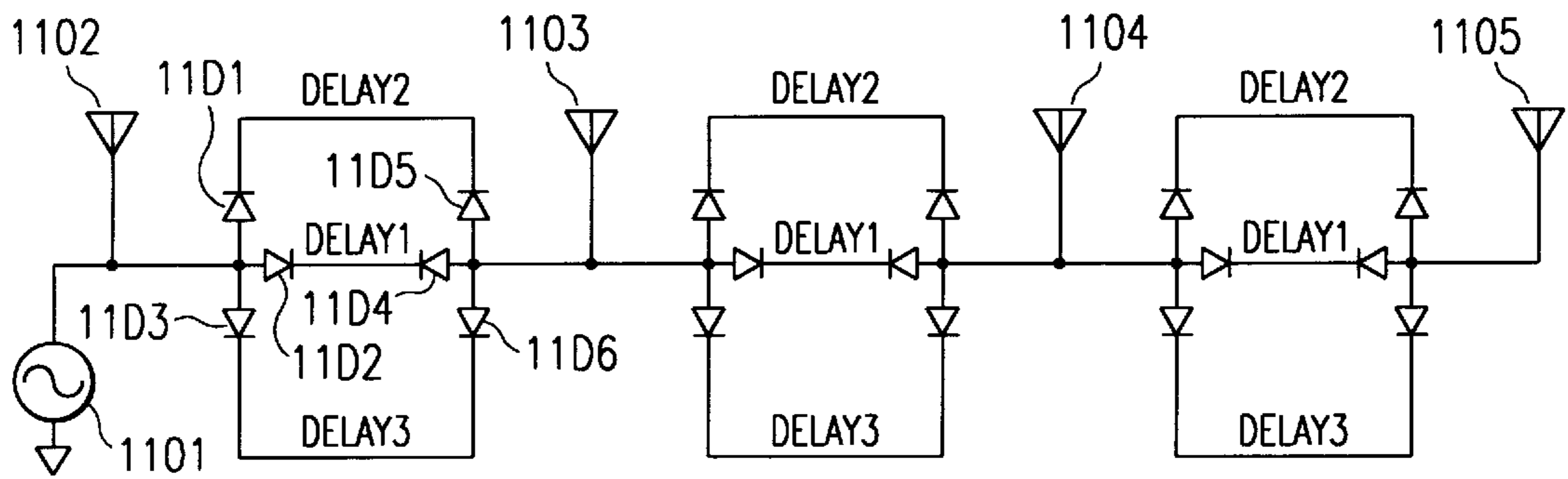
DIODE SWITCHED CIRCUIT
