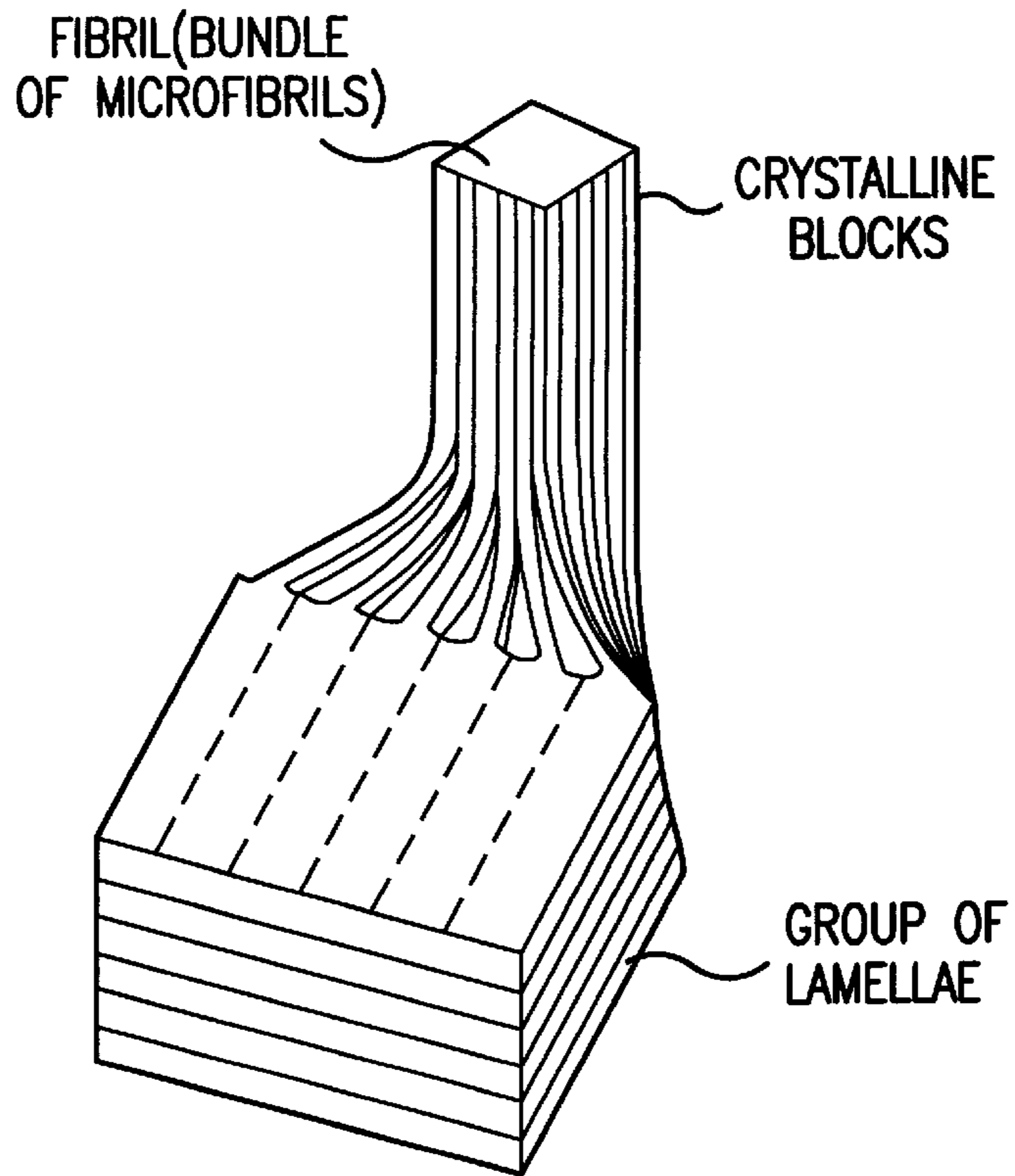
TRANSFORMATION OF LAMELLAR STRUCTURE TO FIBRILLAR STRUCTURE
