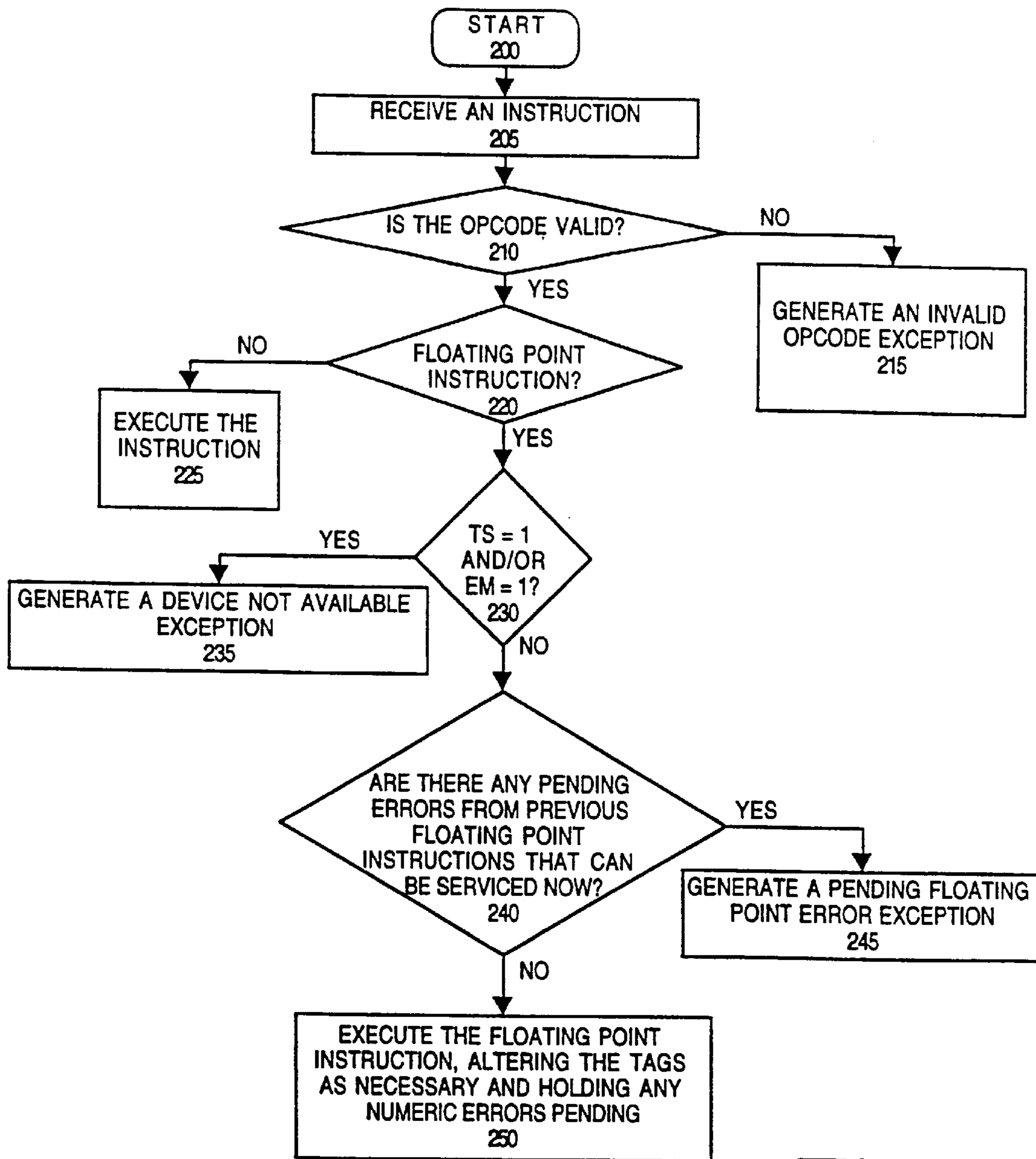
Fig. 2 (Prior Art)
