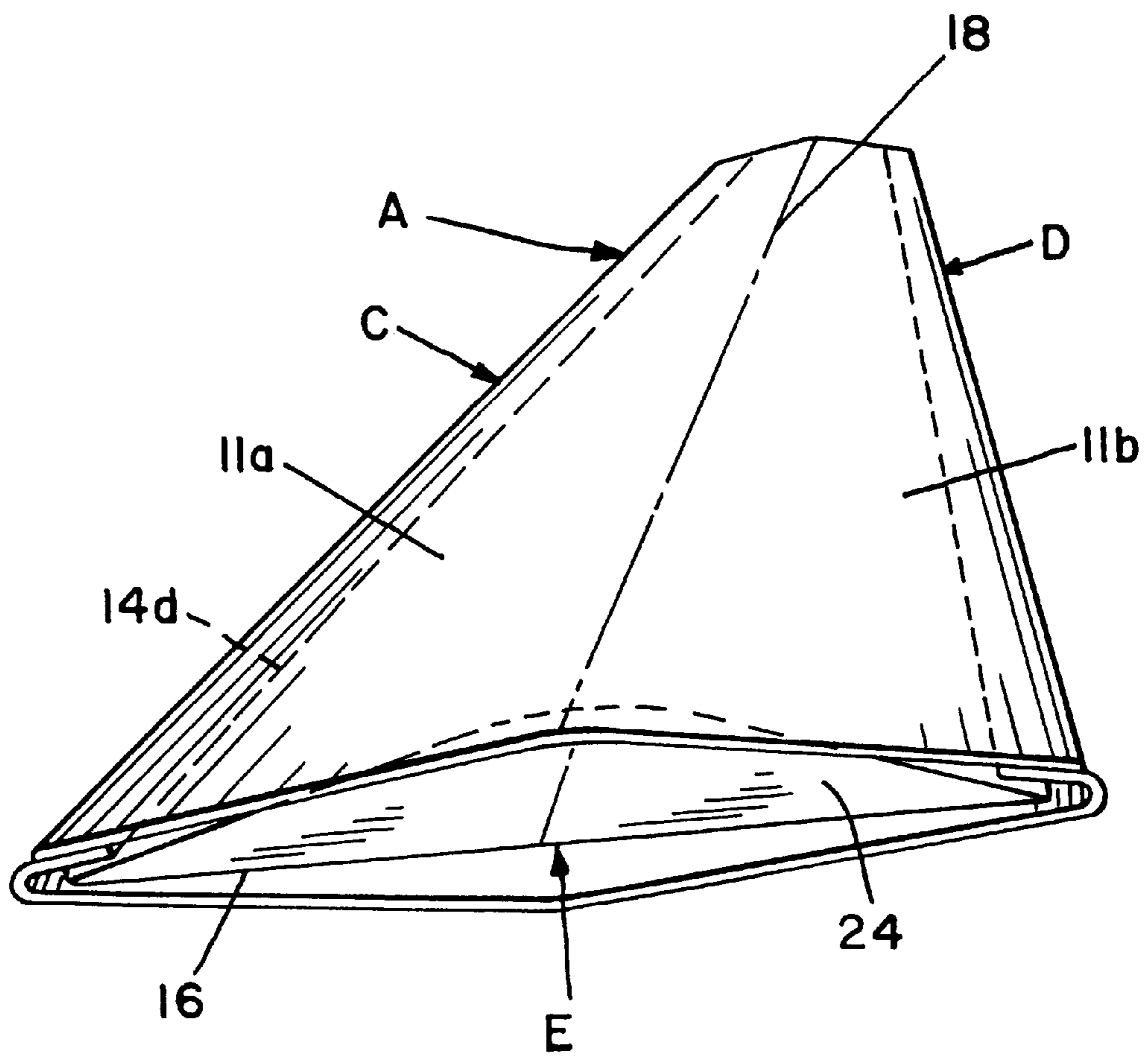
FIG. 2 PRIOR ART
