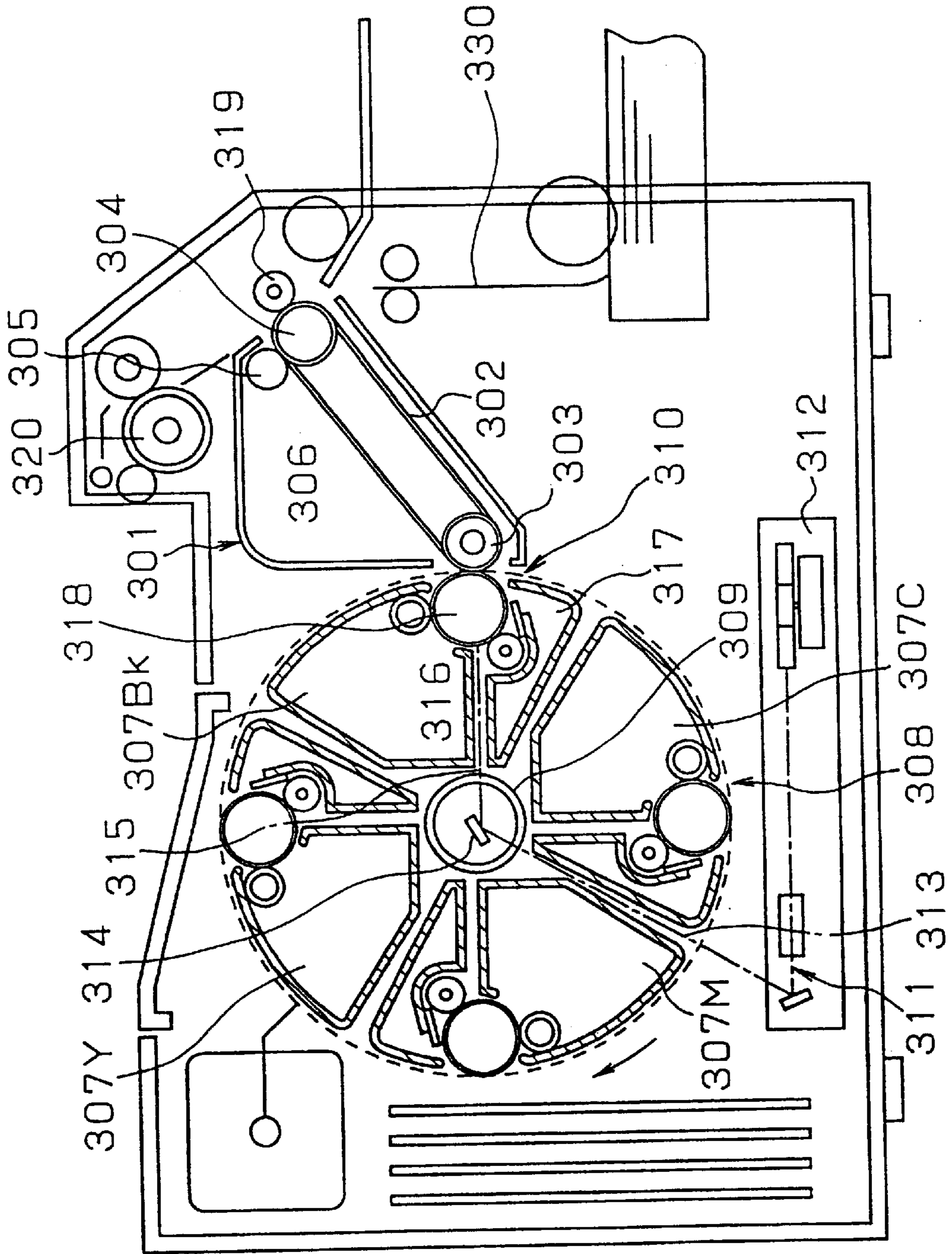
FIG. 20 (PRIOR ART)
