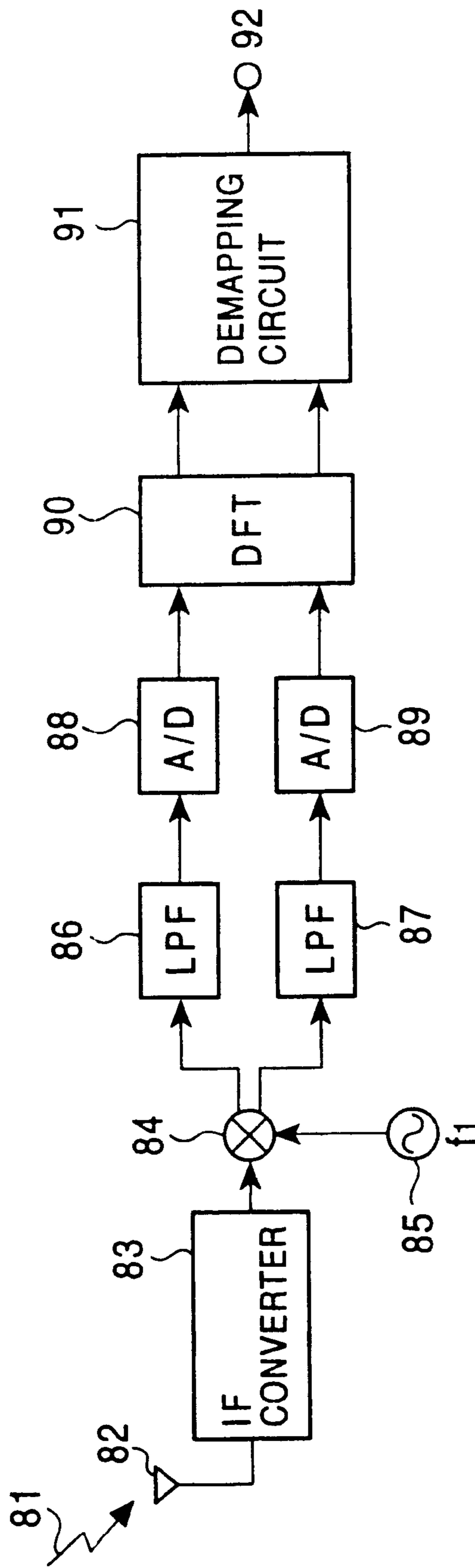
FIG. 12 (PRIOR ART)
