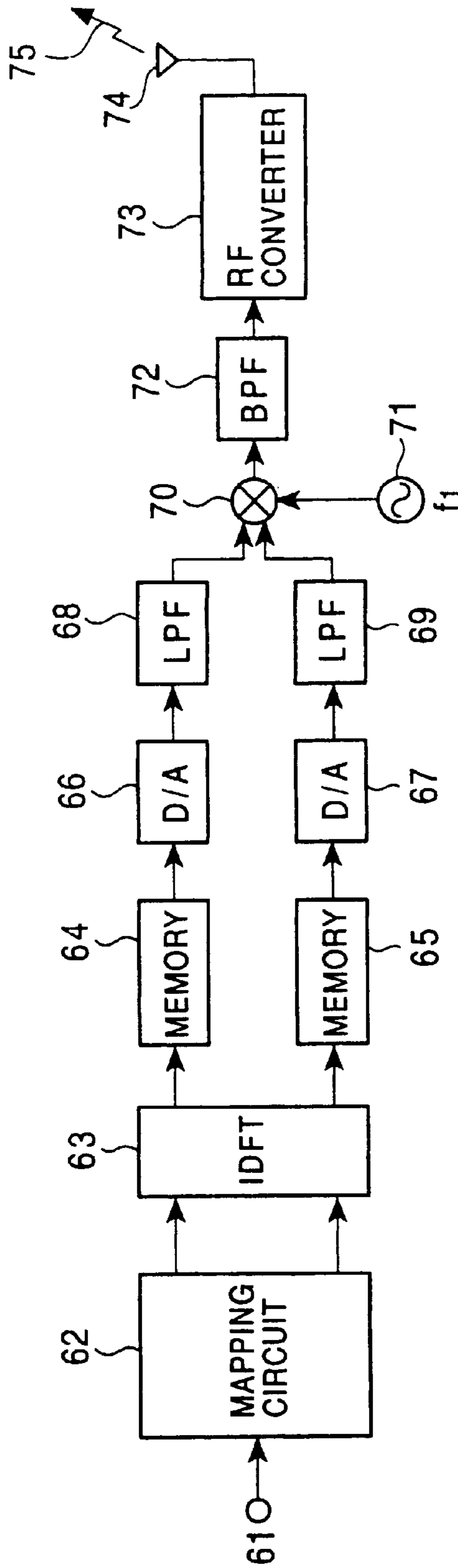
FIG. 11 (PRIOR ART)
