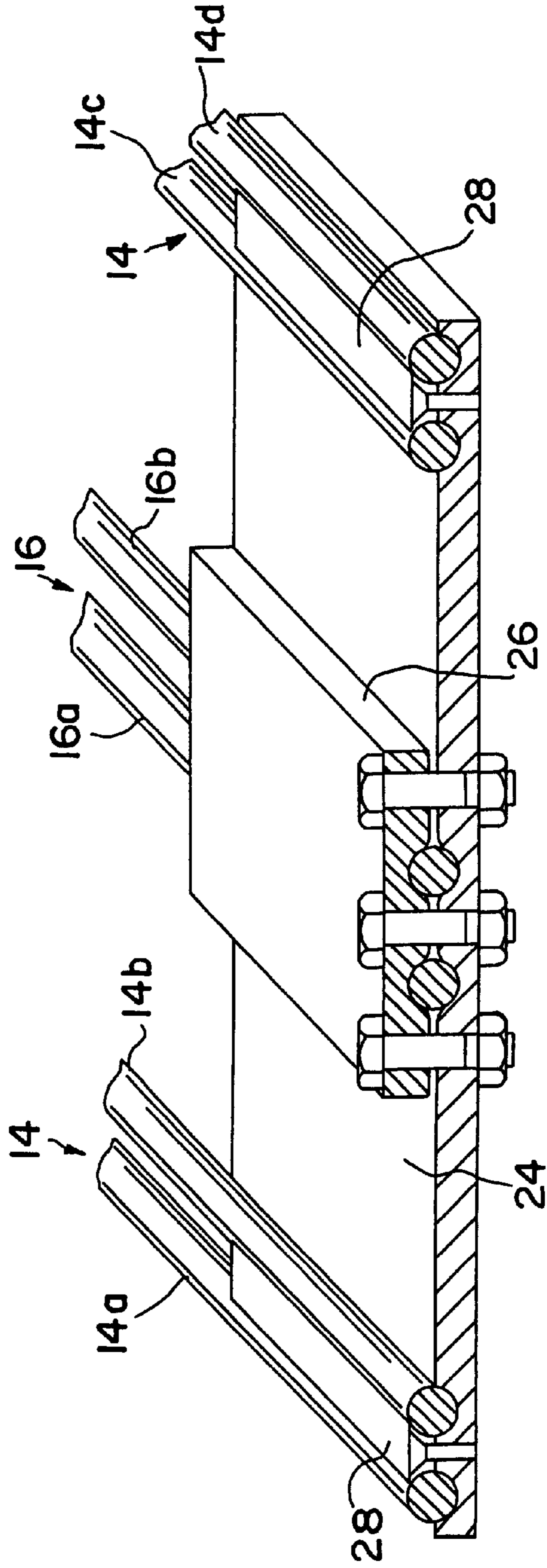
FIG. 5 PRIOR ART
