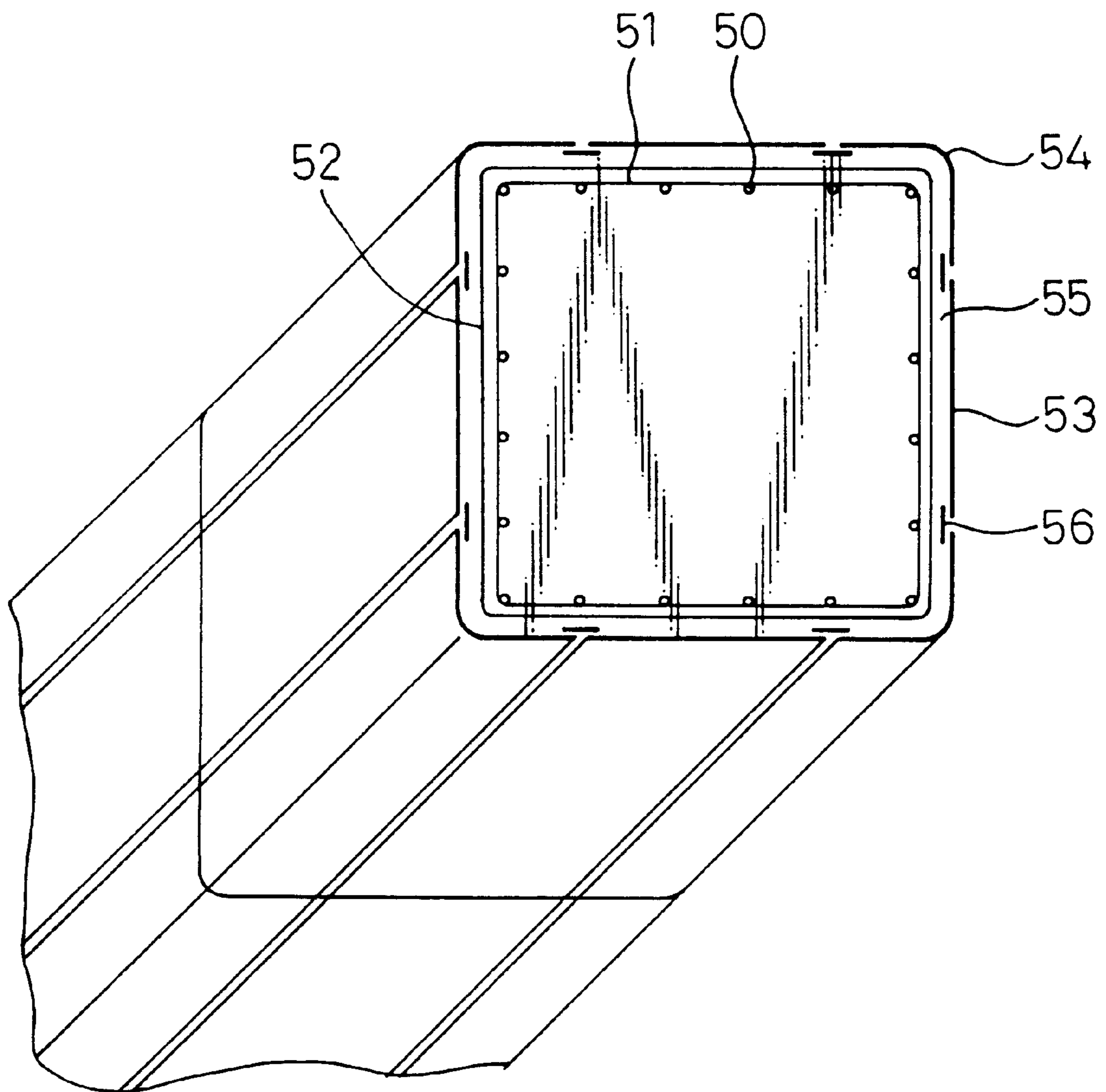
Fig. 24 PRIOR ART
