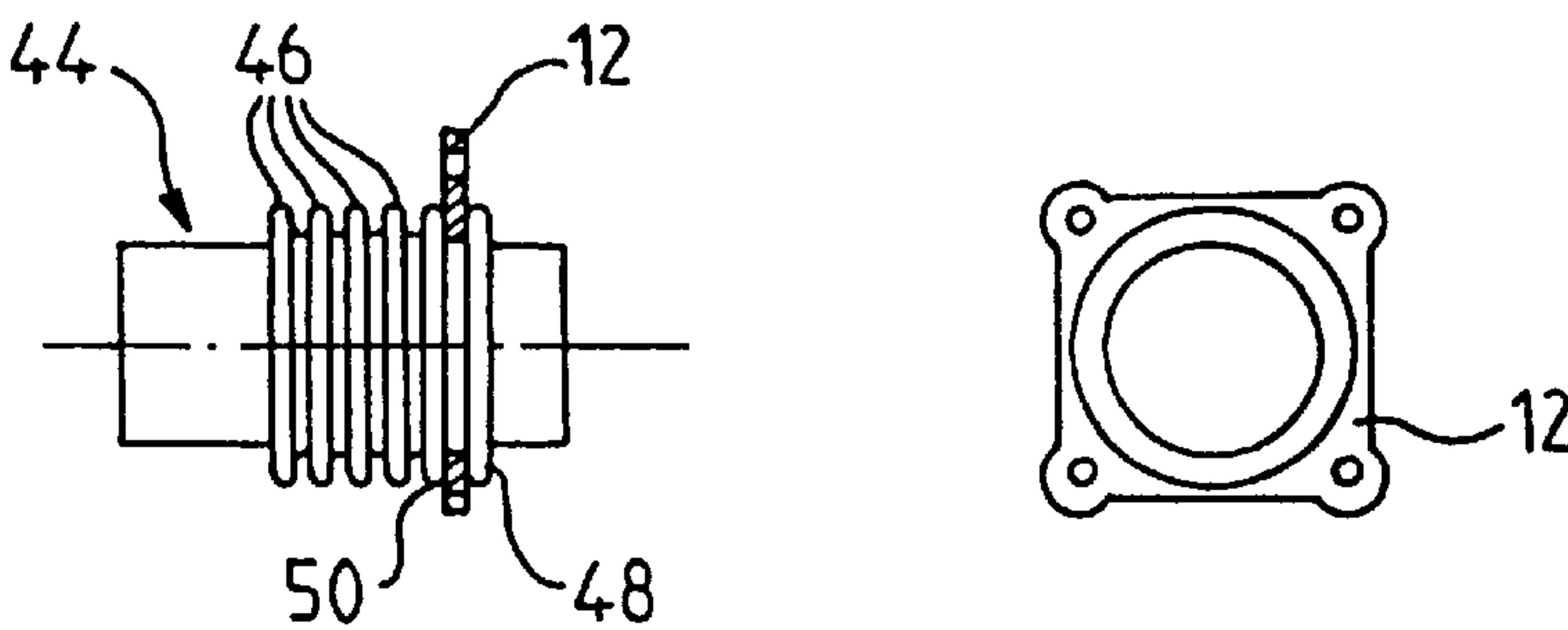
HYDROFORM FLANGE & BELLOWS 1 - UP SHOWN 3 - UP .RECOMMENDED
