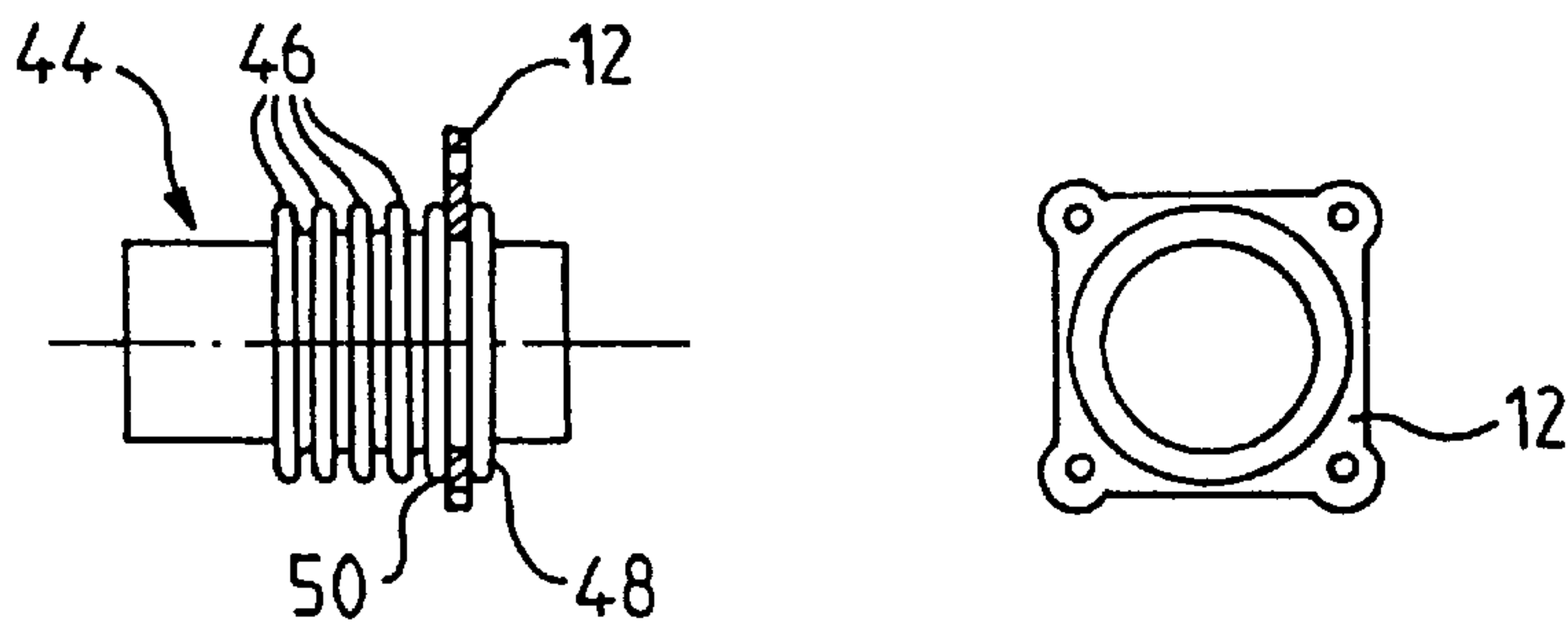
HYDROFORM FLANGE & BELLOWS
