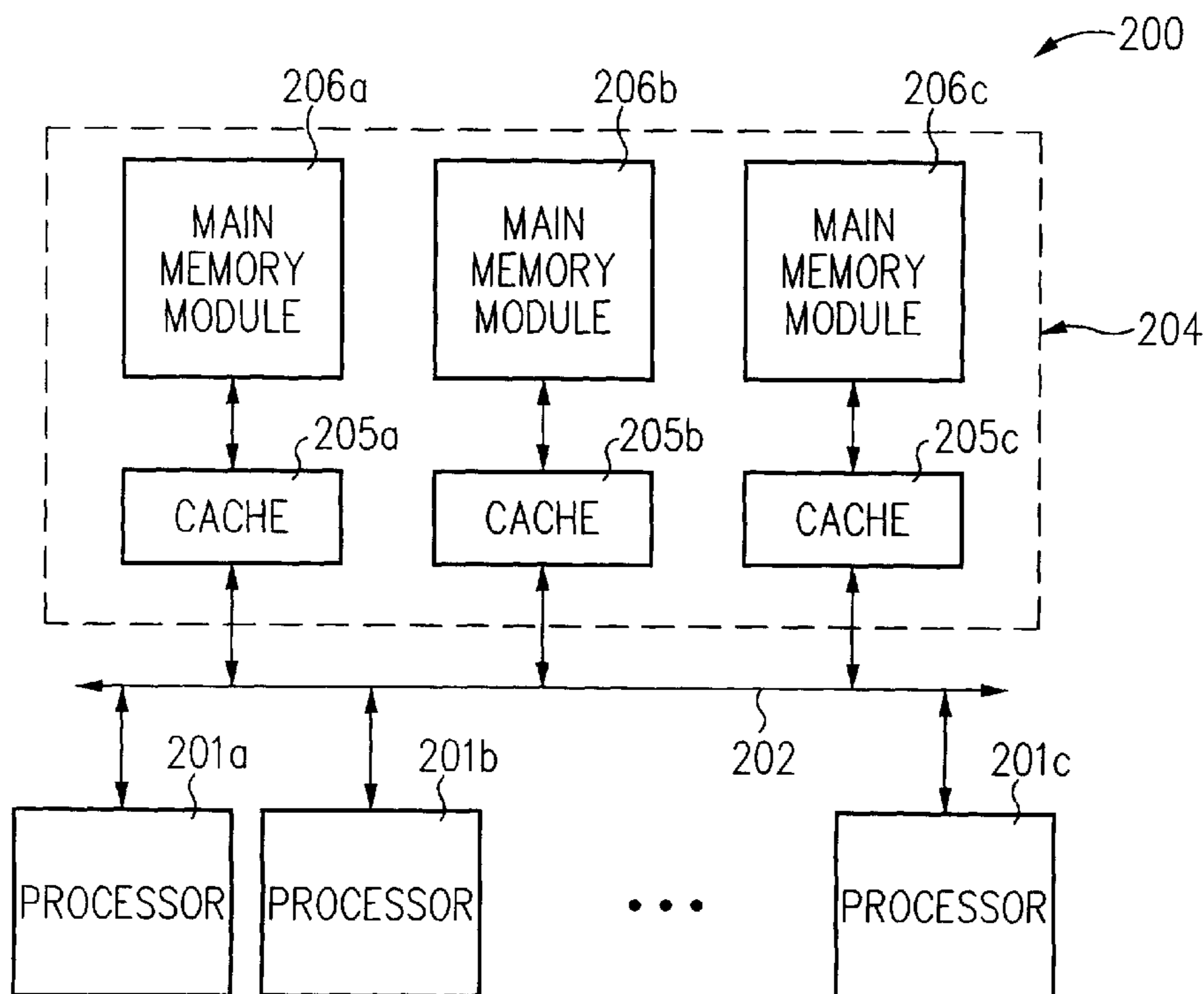
FIG. 2 (PRIOR ART)
