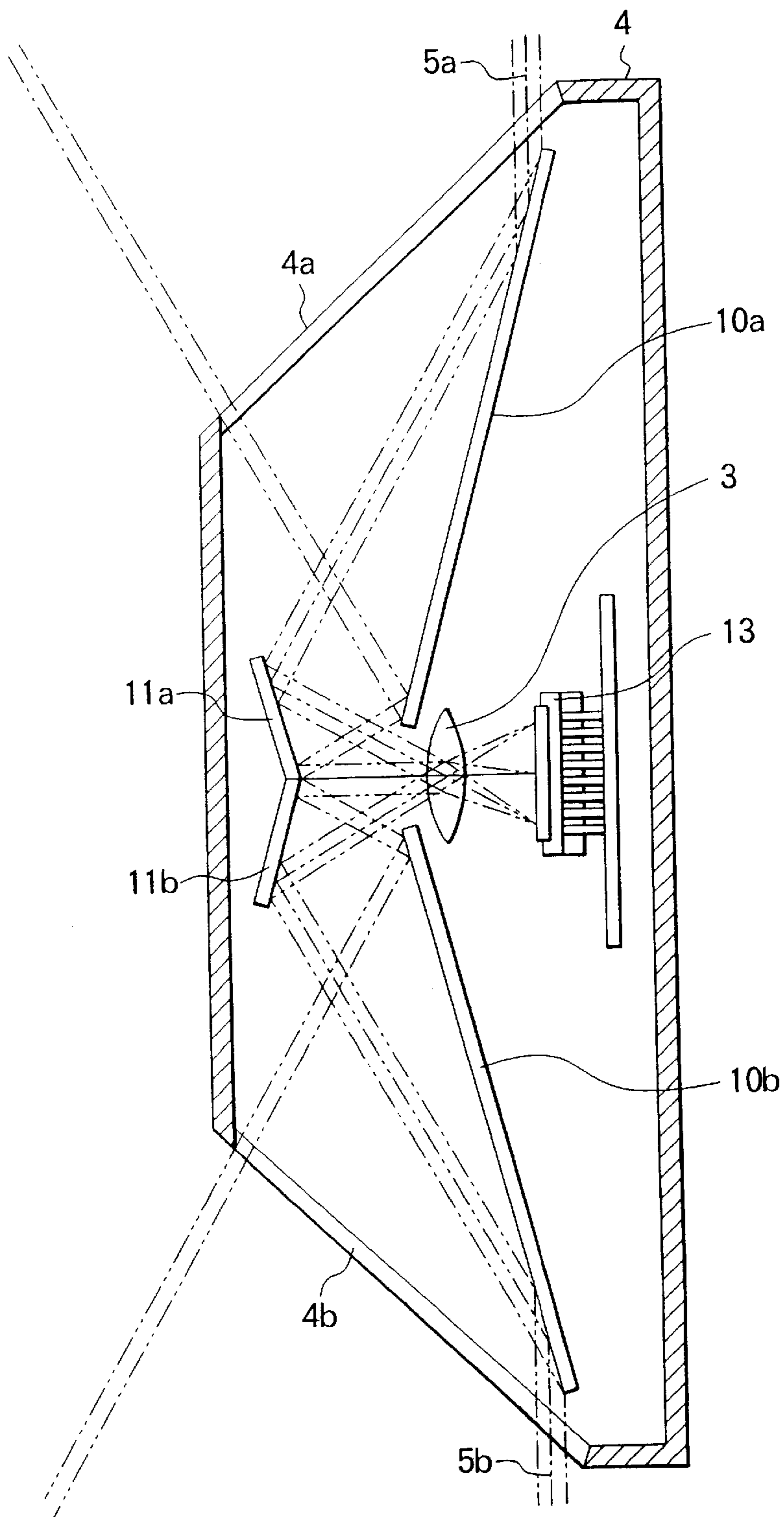
FIG. 13 PRIOR ART
