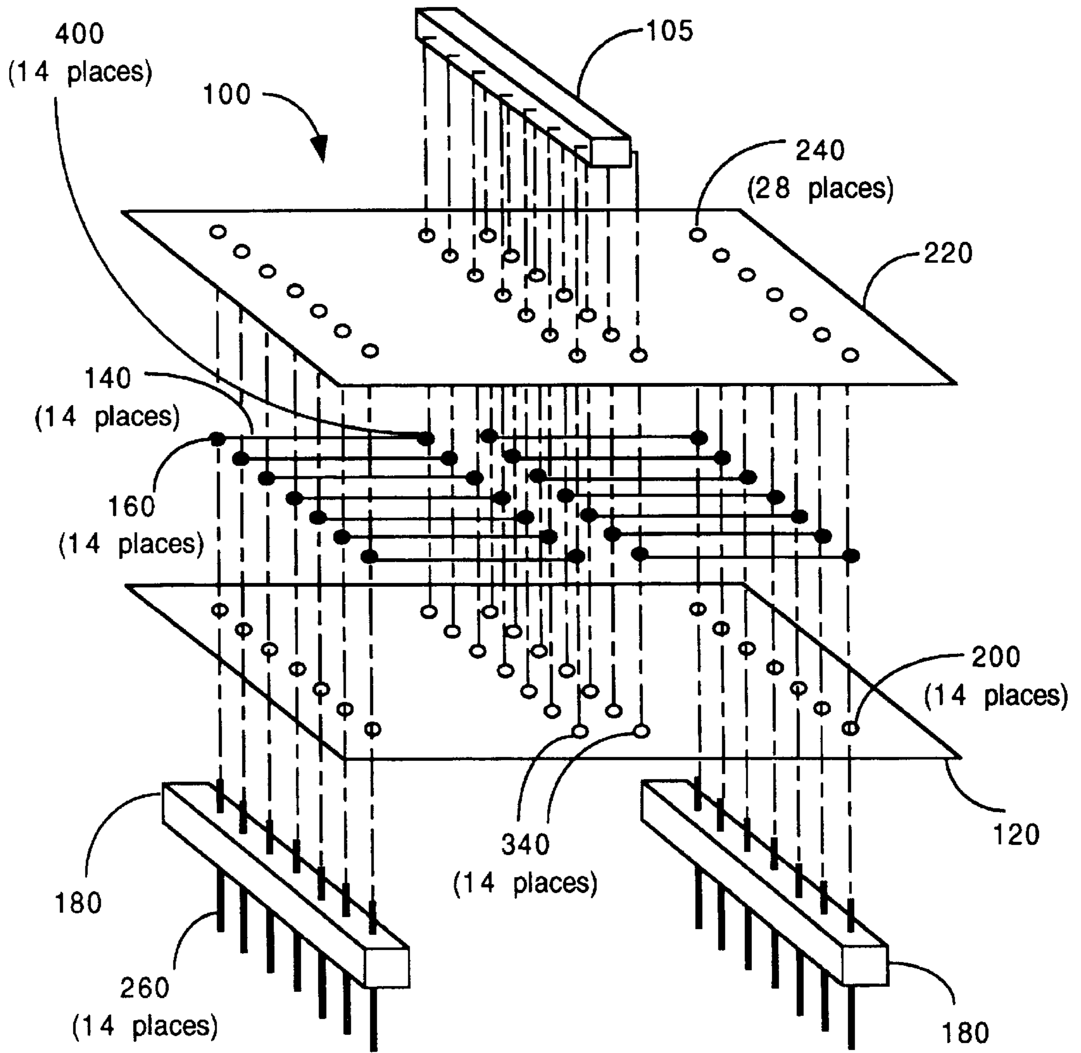
Figure 4 Exploded View - Dual-In Line Mount, Unfolded
