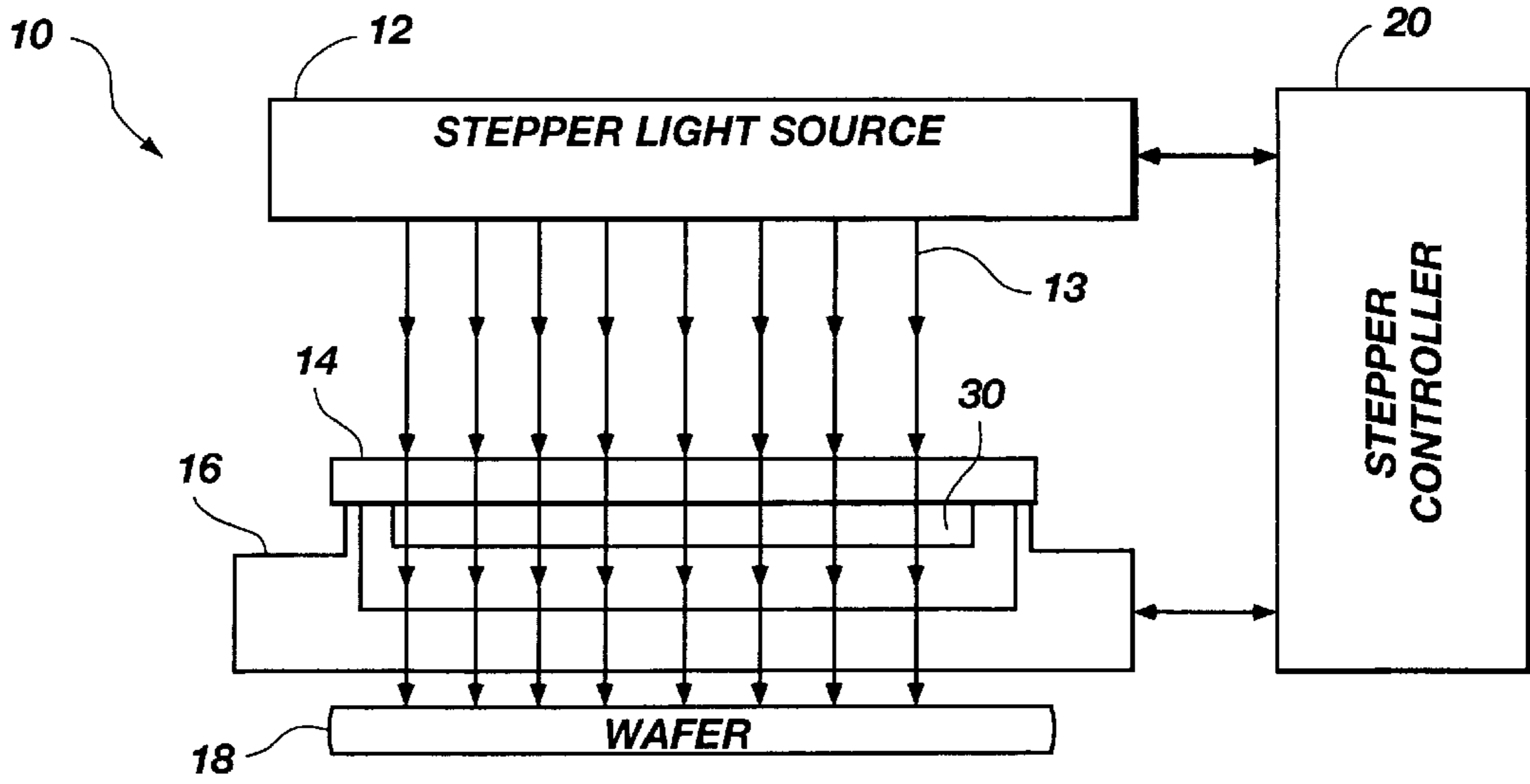
Fig. 1 (PRIOR ART)
