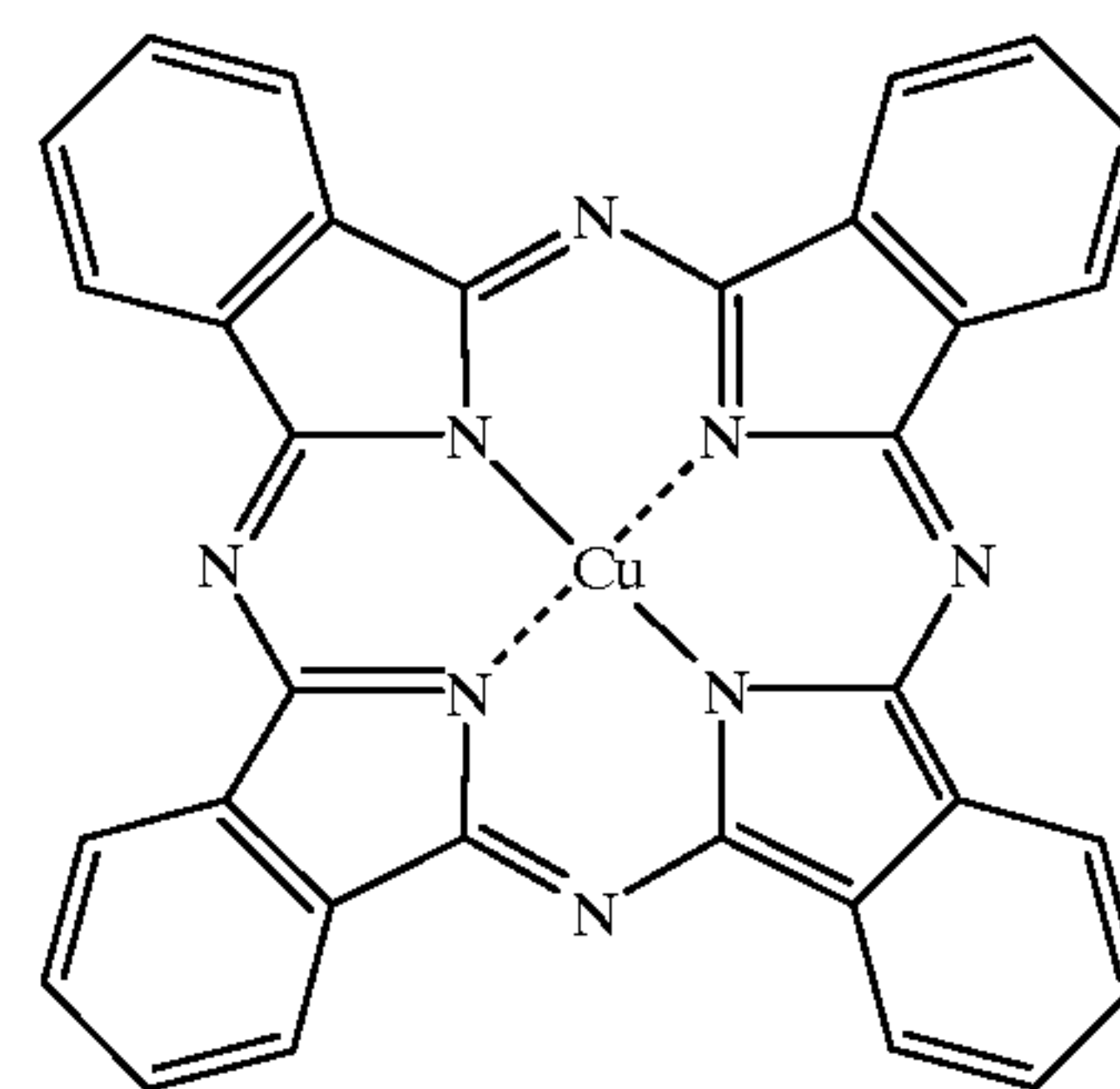
Cu-Phthalocyanine
