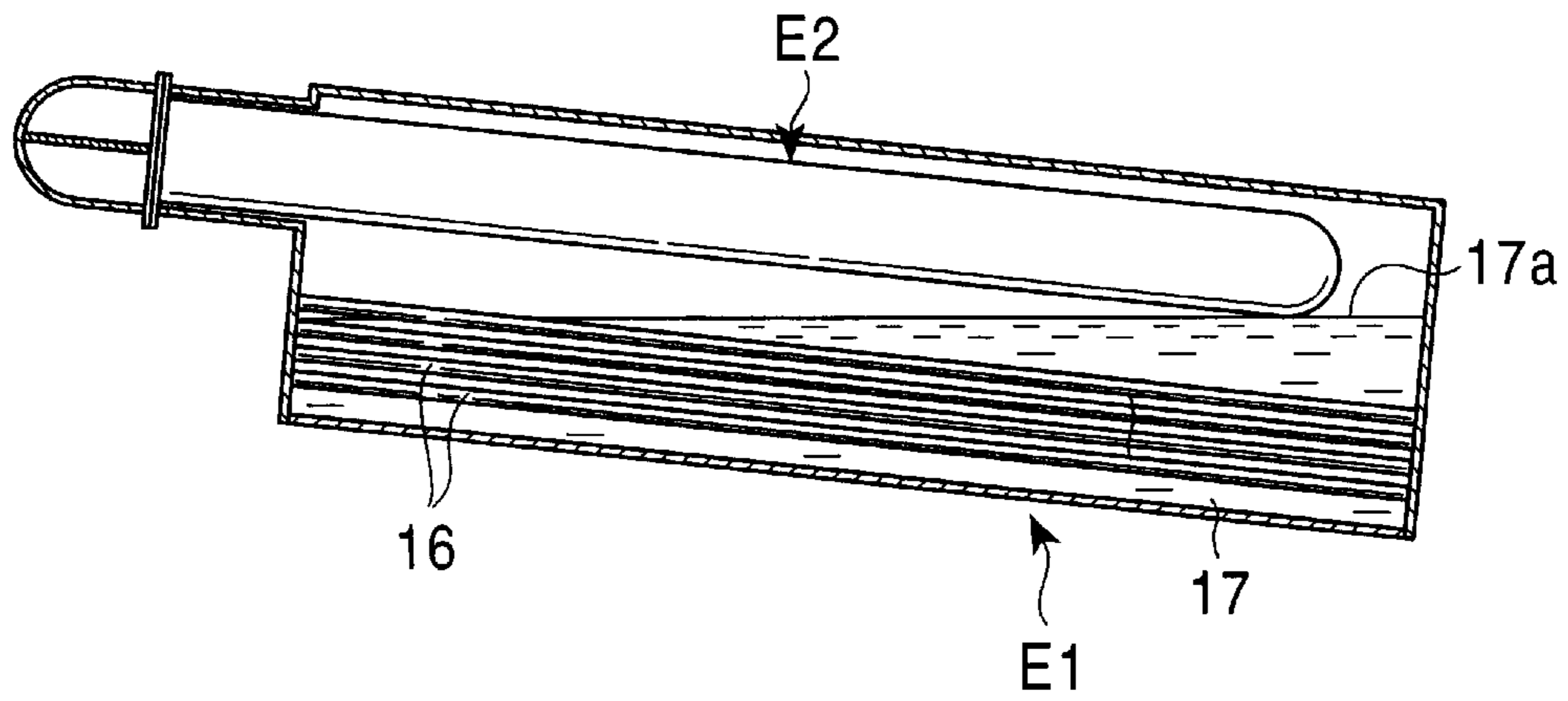
FIG. 6C PRIOR ART
