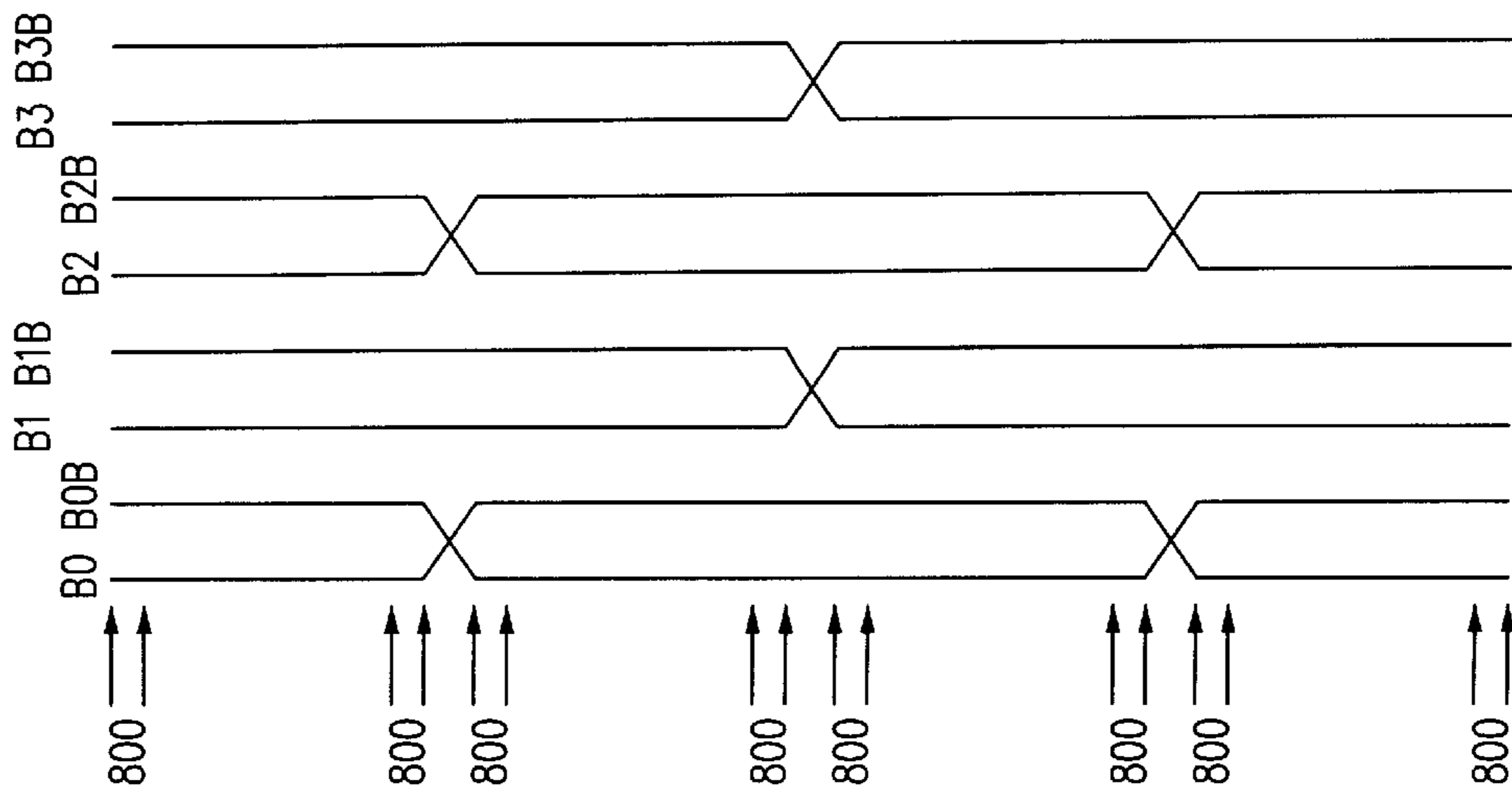
FIG. 35 (PRIOR ART)
