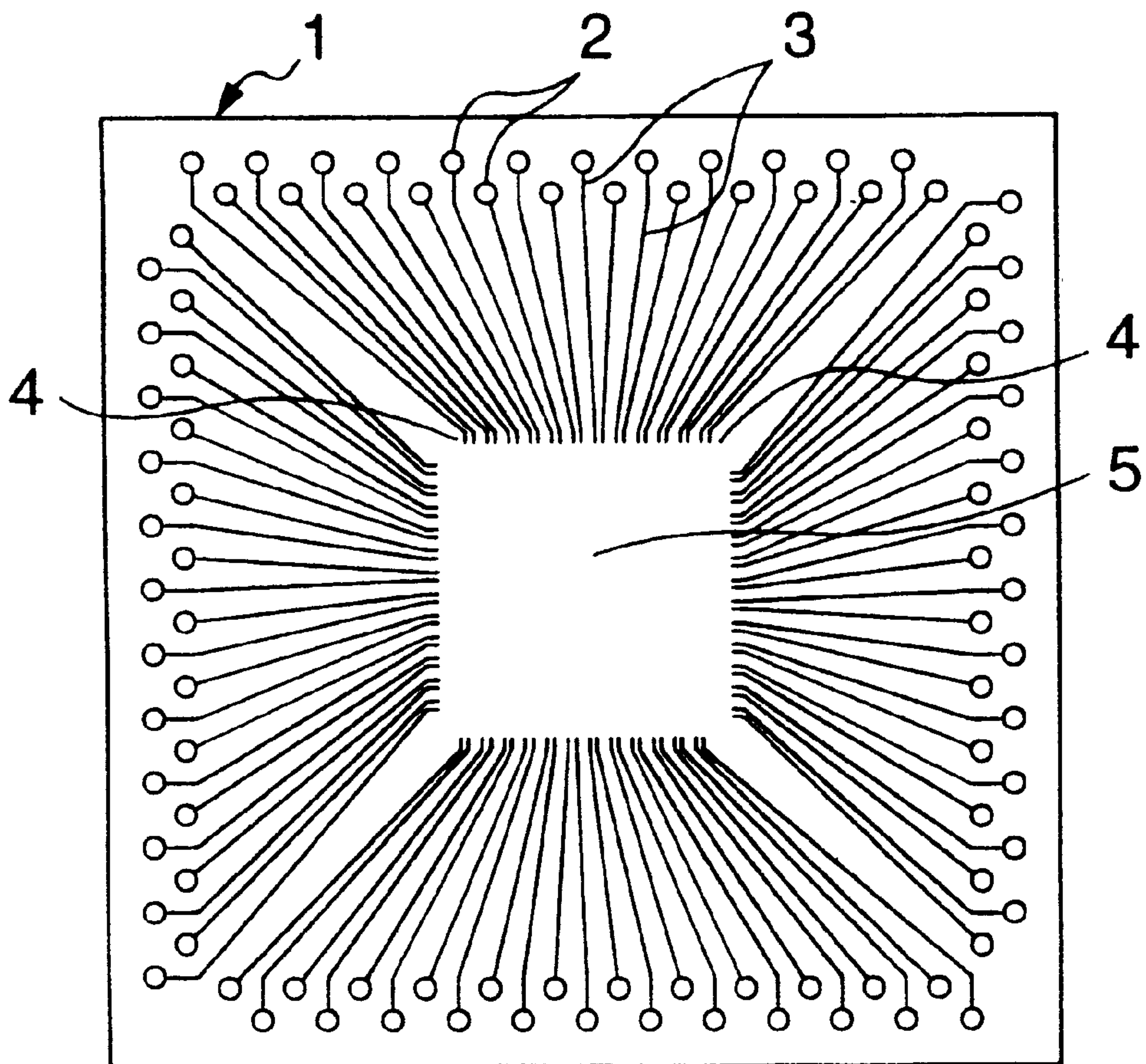
FIG. 9 PRIOR ART
