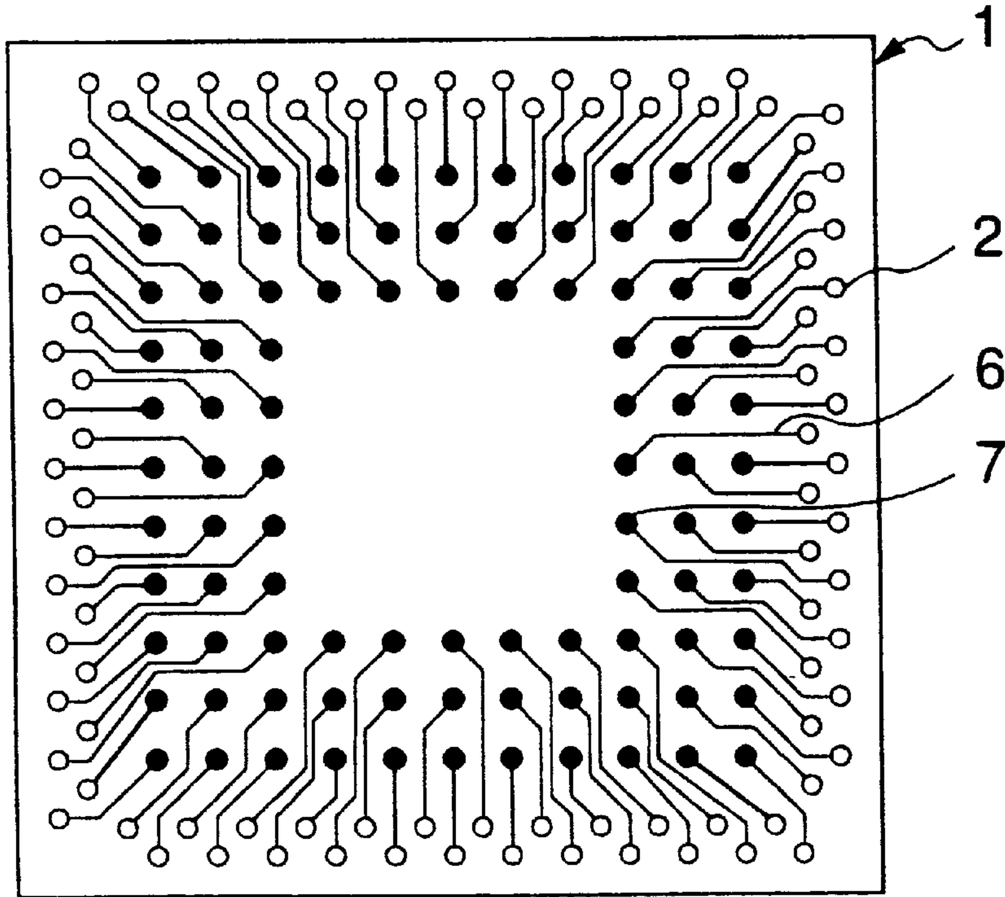
FIG. 10 PRIOR ART
