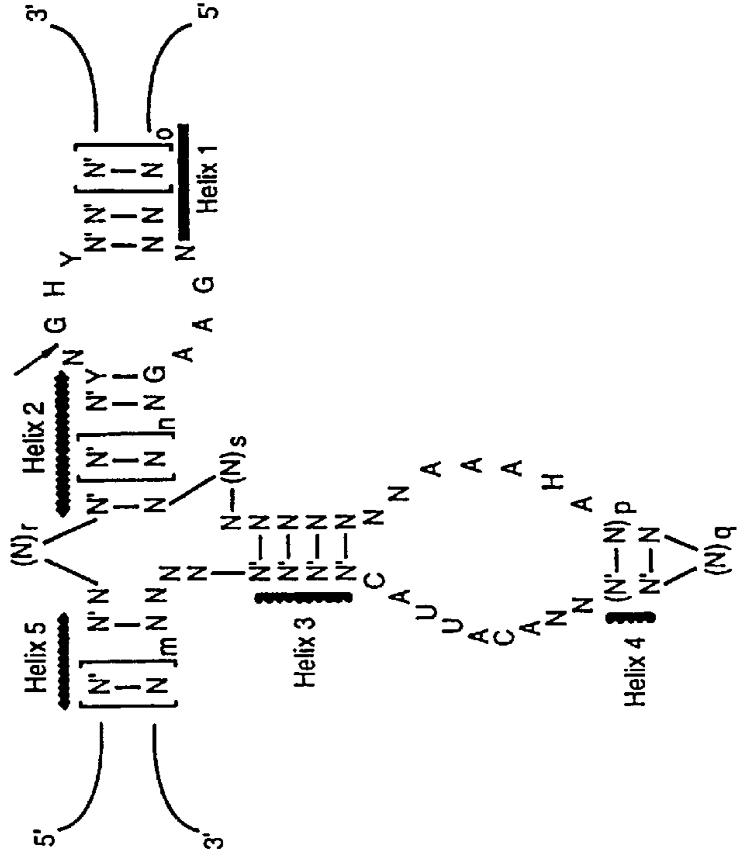
HAIRPIN RIBOZYME
