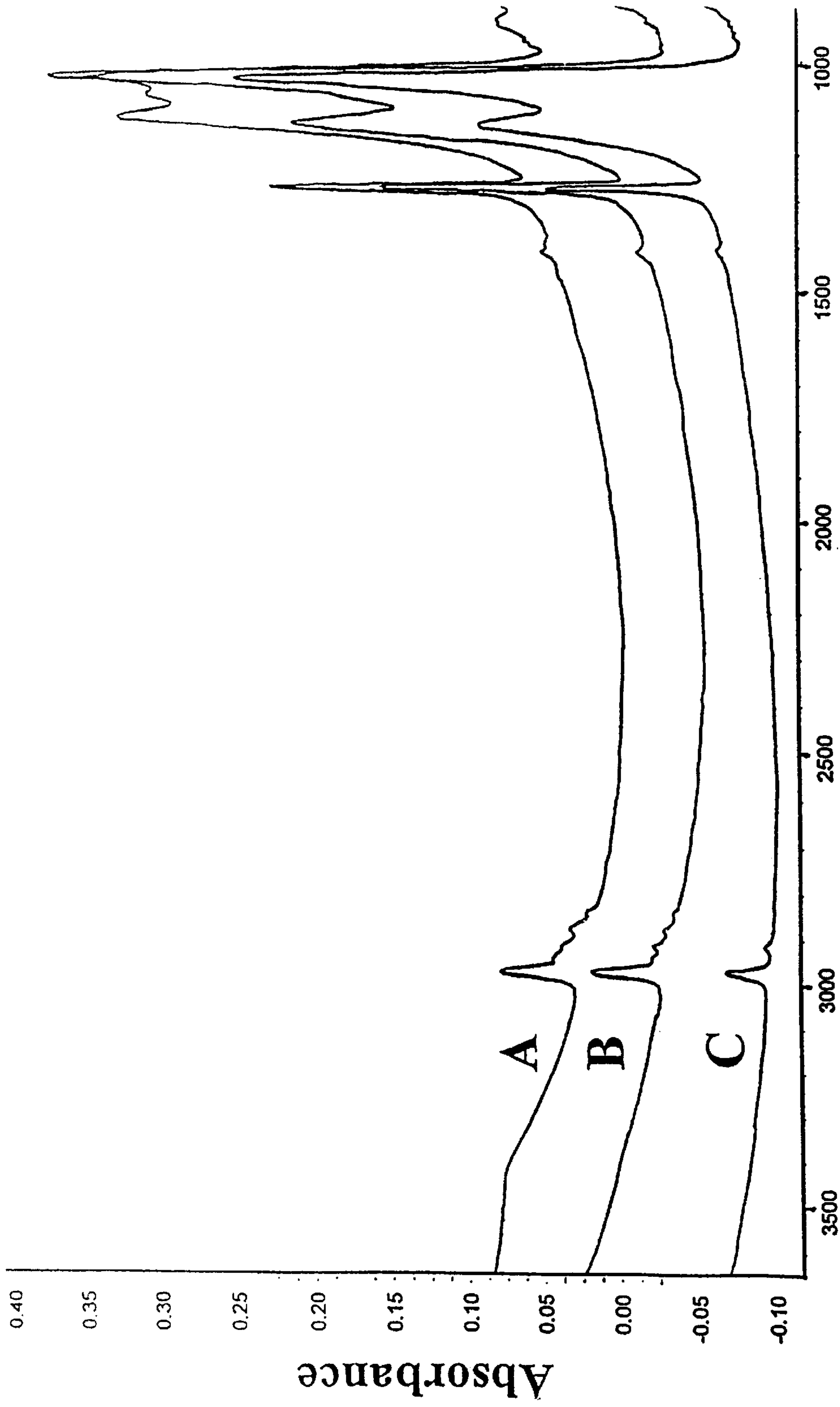
Wavenumber, cm -1
