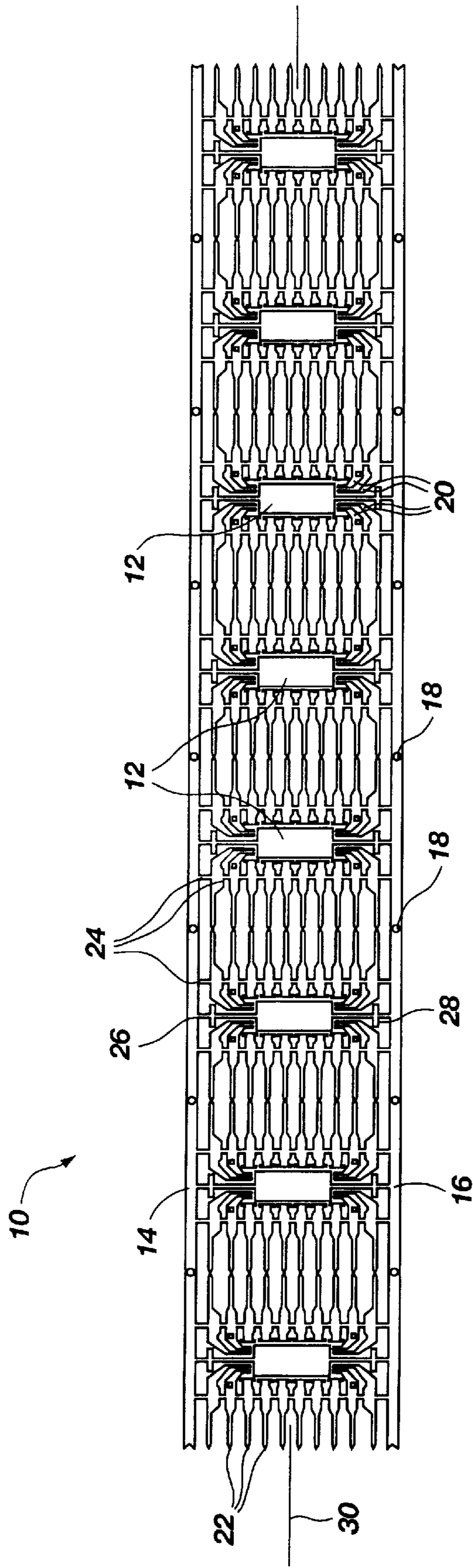
Fig. 1 (PRIOR ART)
