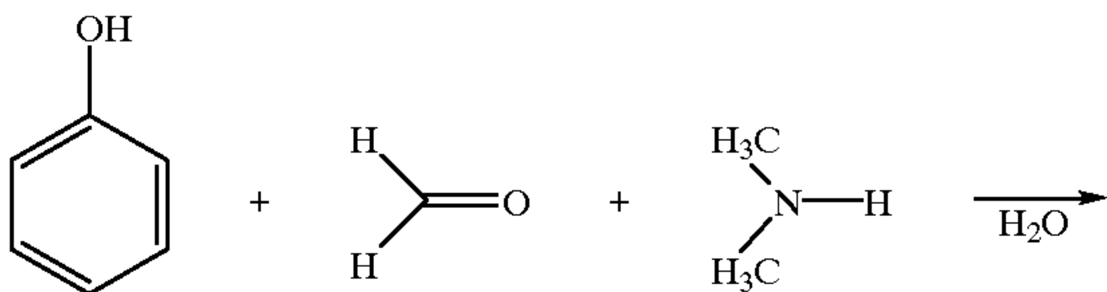
Reaction formula [1]
