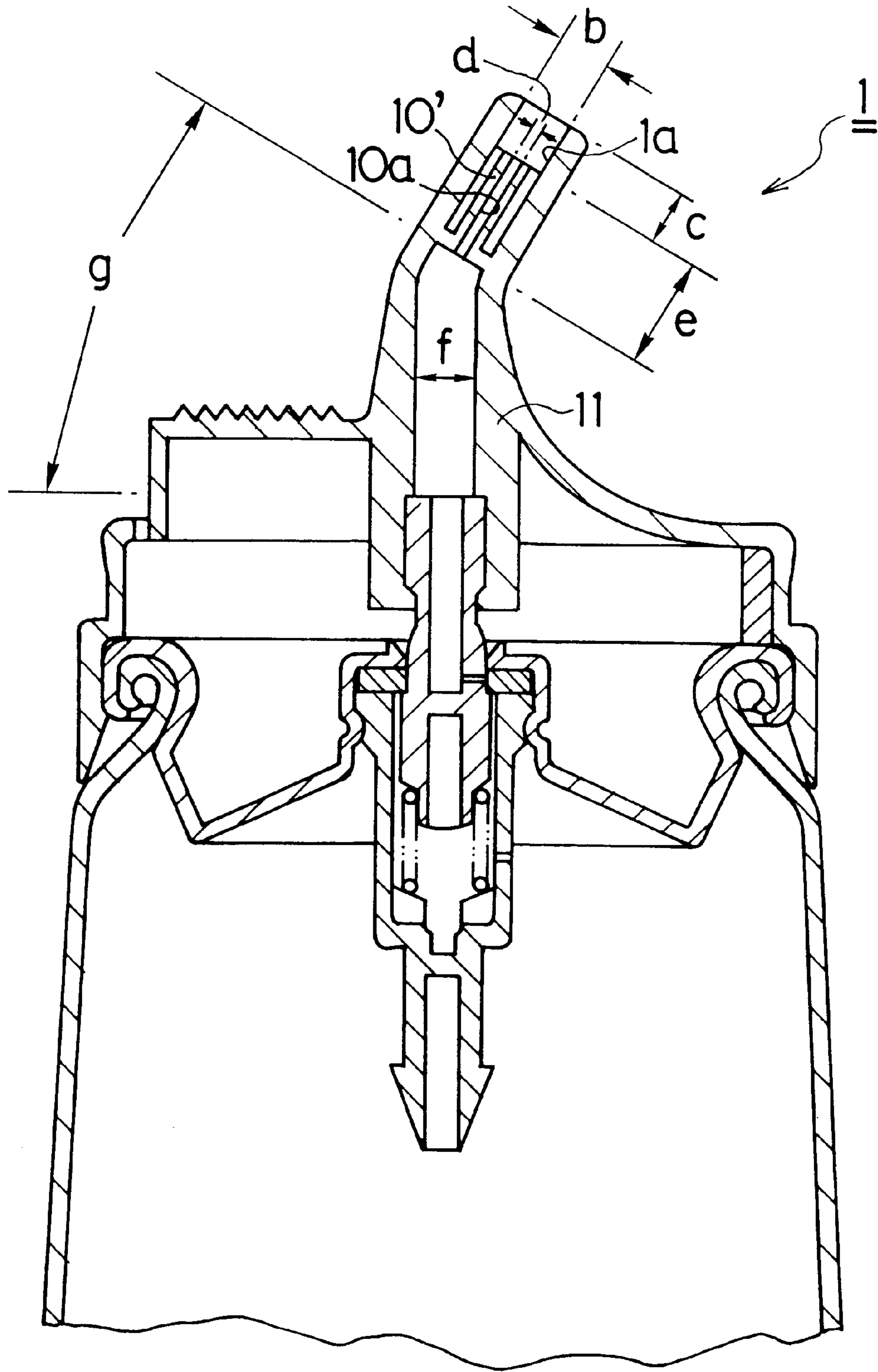
FIG. 6 (PRIOR ART)
