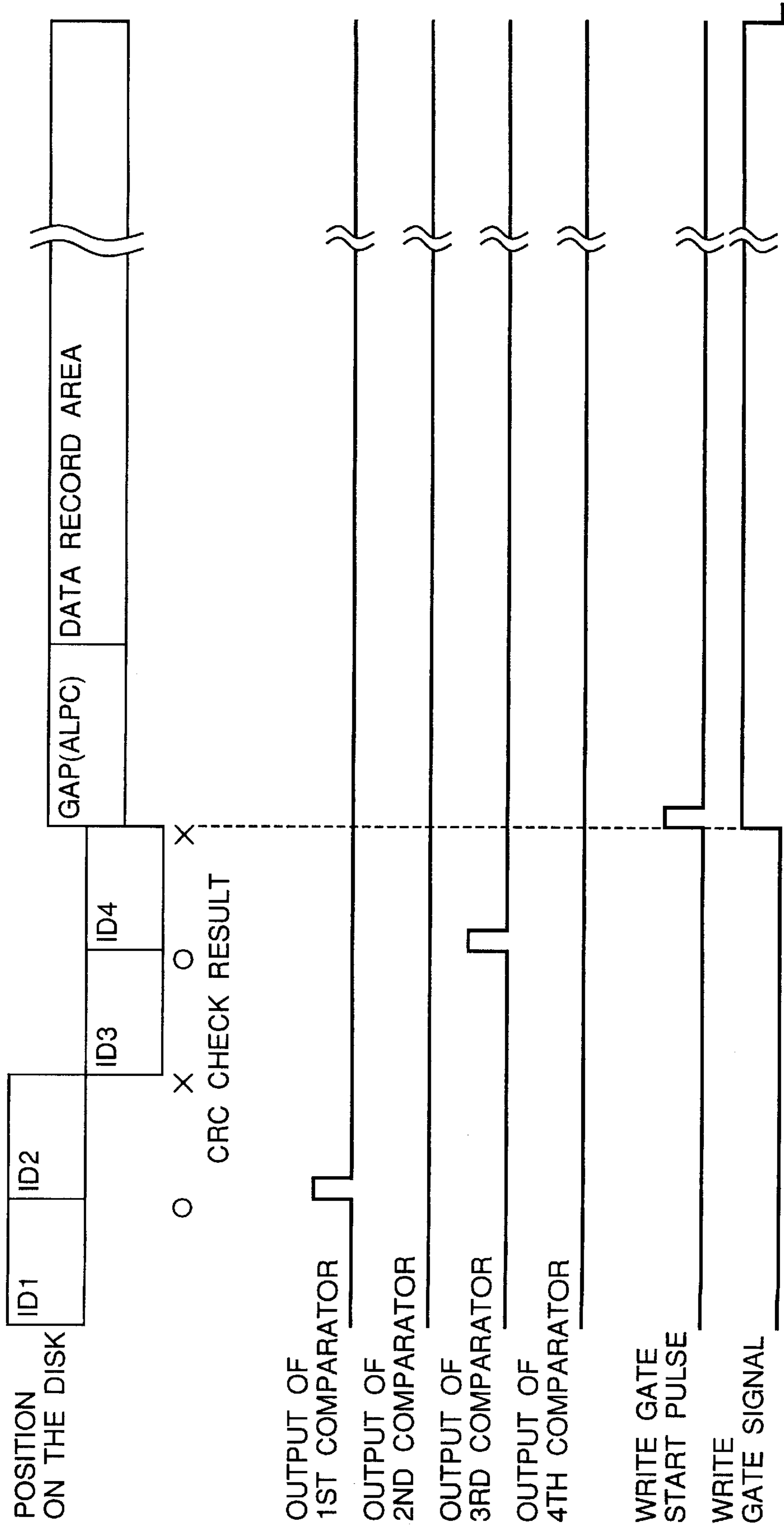
Fig.5 PRIOR ART
