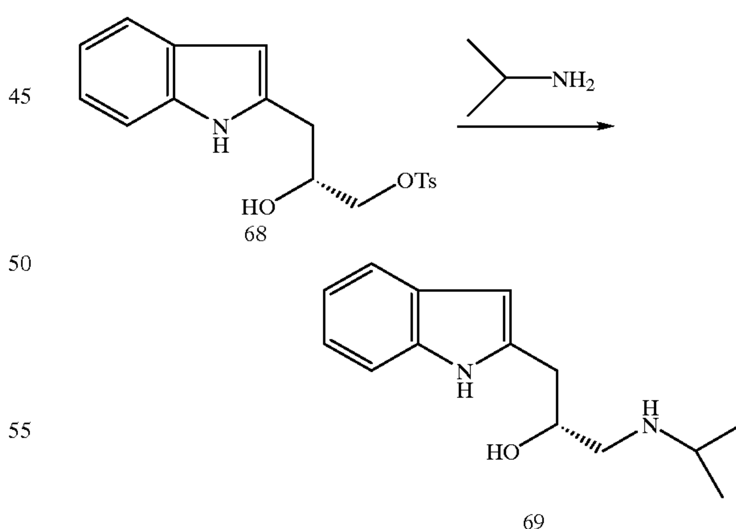
Amino compound 69
