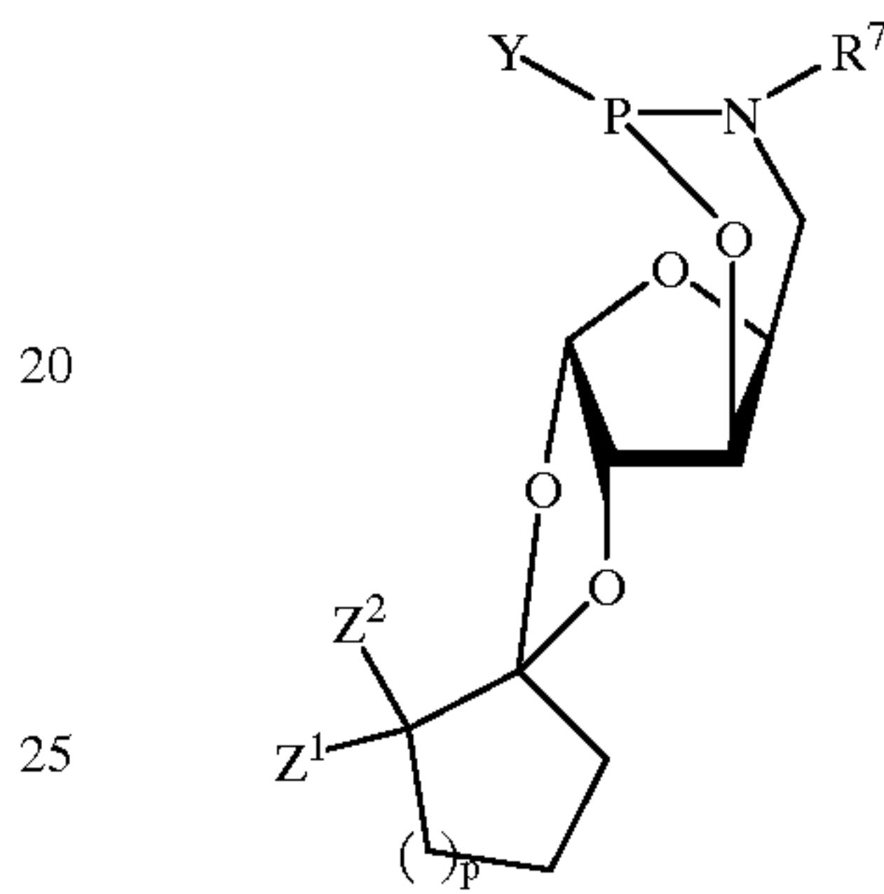
XIIa
