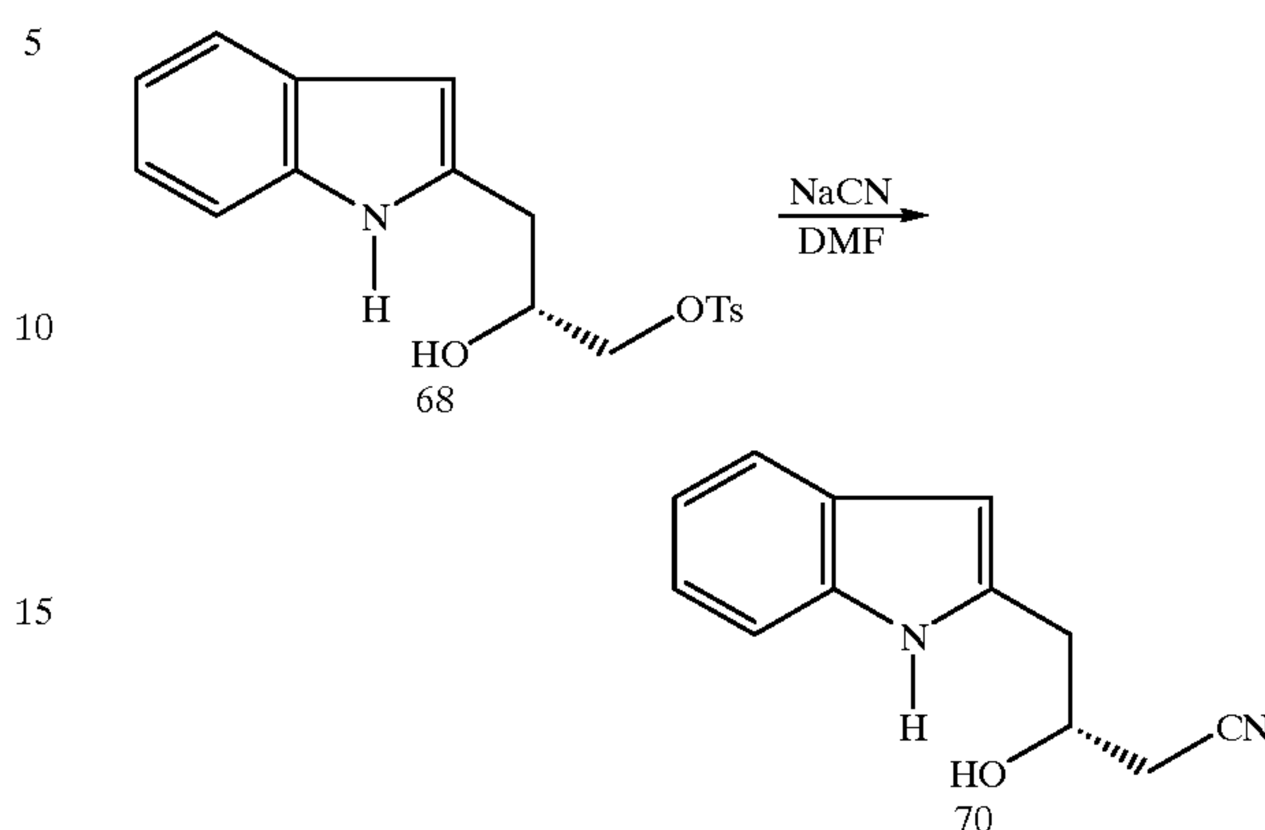
Hydroxycyanopropylindole 70
