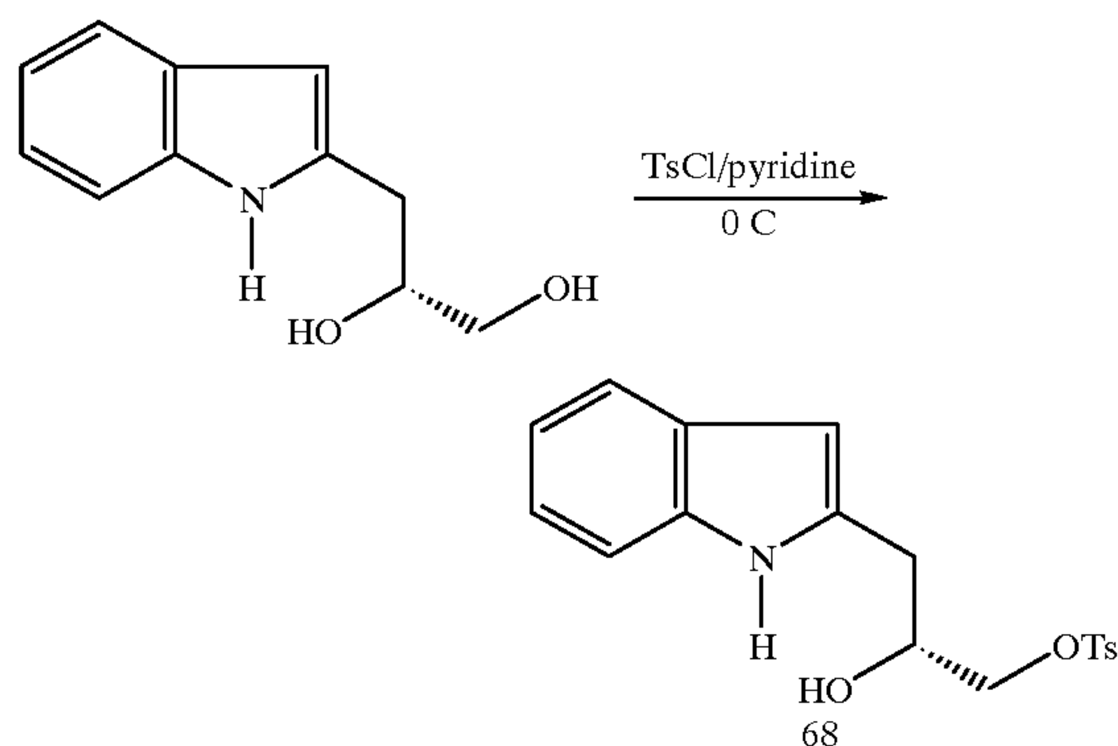
1-p-toluenesulfonic-3-indol-2-yl-propan-2-ol (68)
