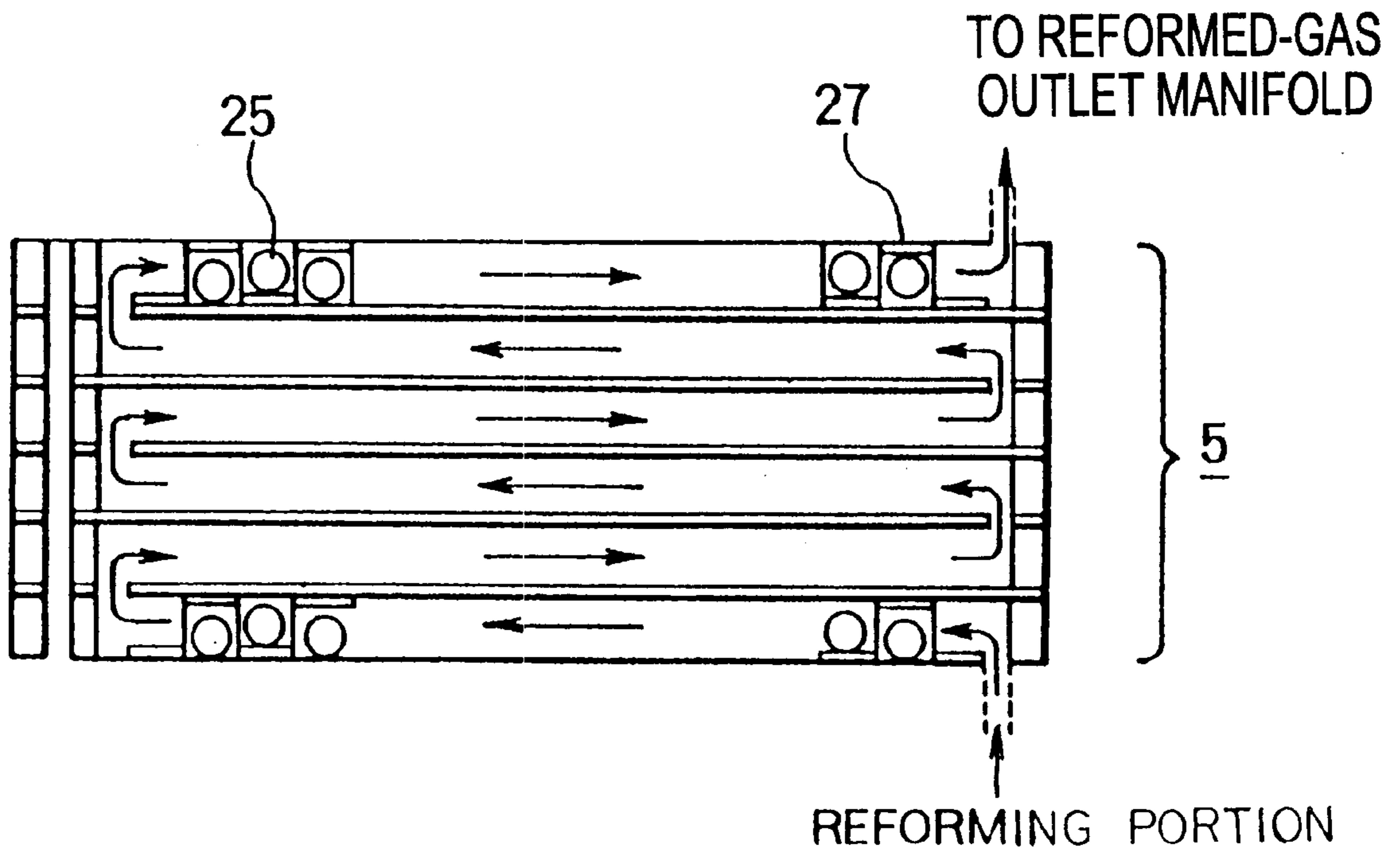
5: MULTILAYER CO OXIDATION PORTION
