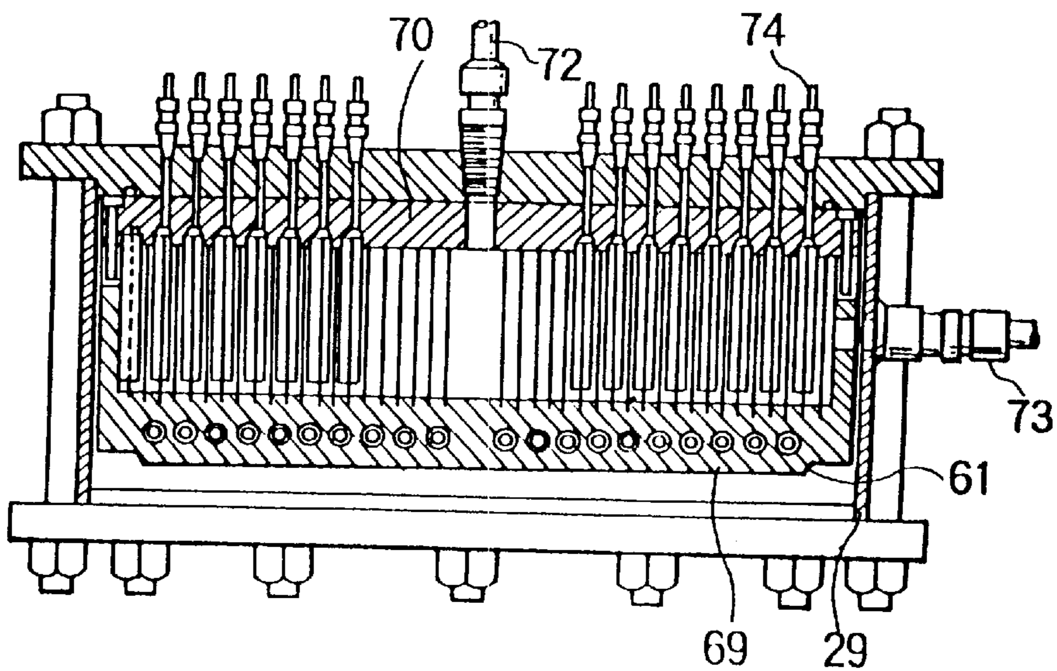
FIG. 24 (PRIOR ART)
