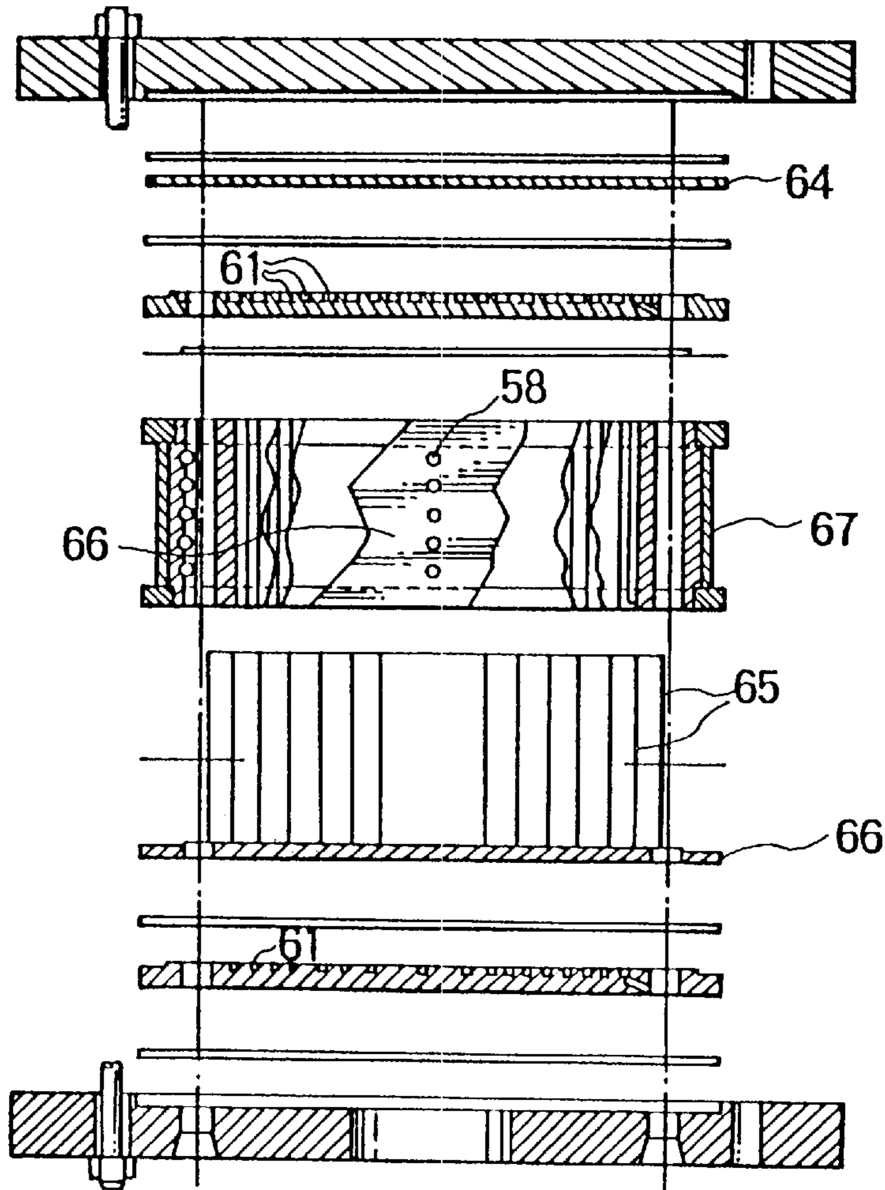
FIG. 23 (PRIOR ART)
