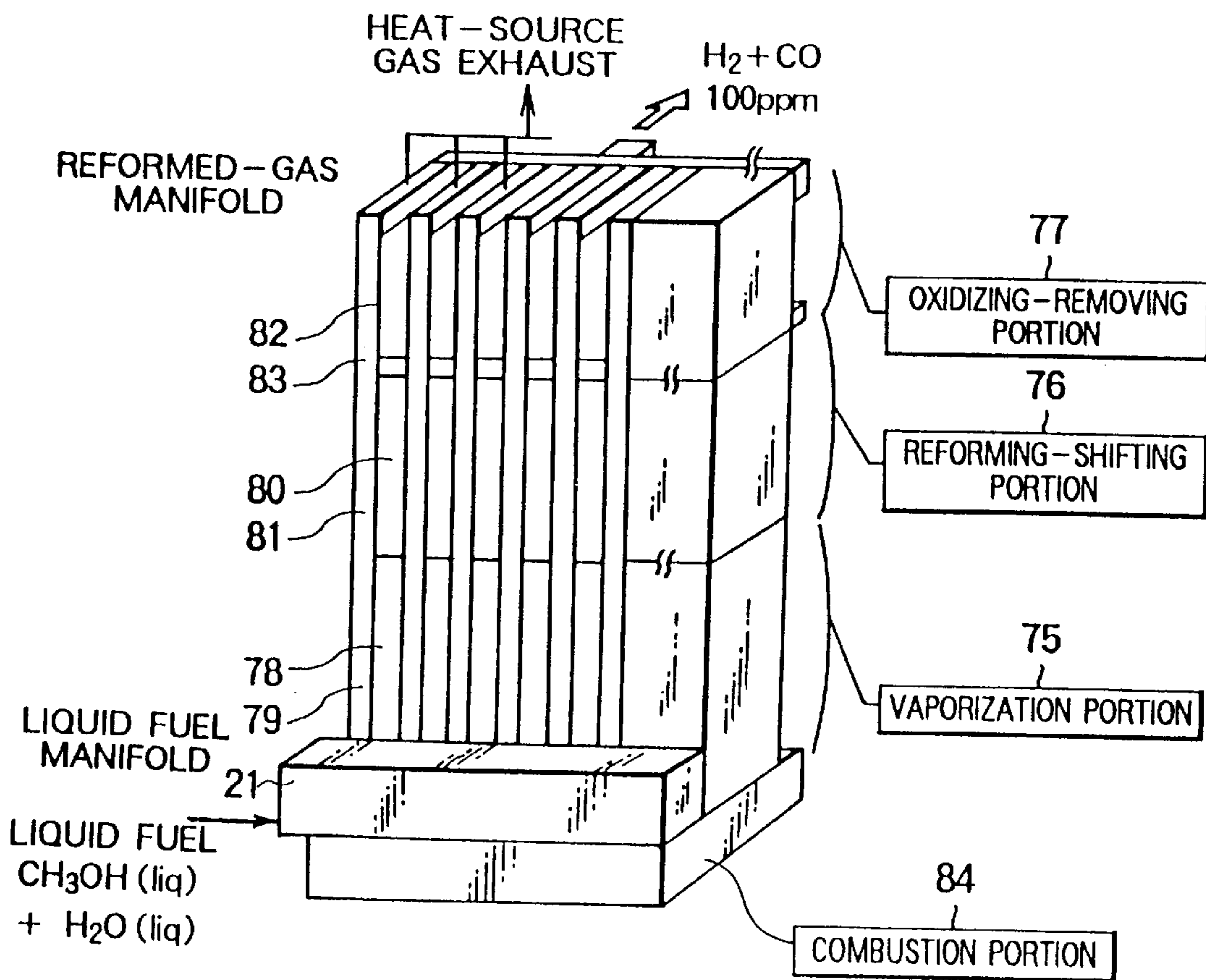
FIG. 26 (PRIOR ART)
