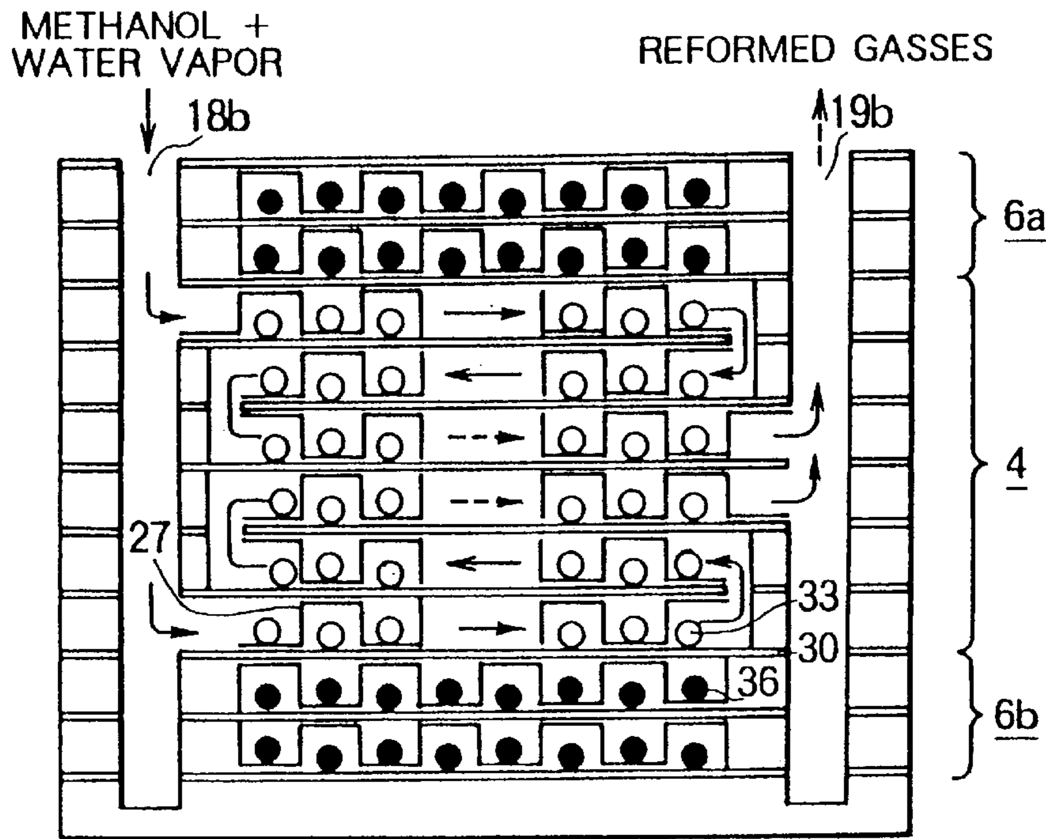
4: MULTILAYER REFORMING PORTION 6a,6b: CATALYTIC COMBUSTION PORTIONS
