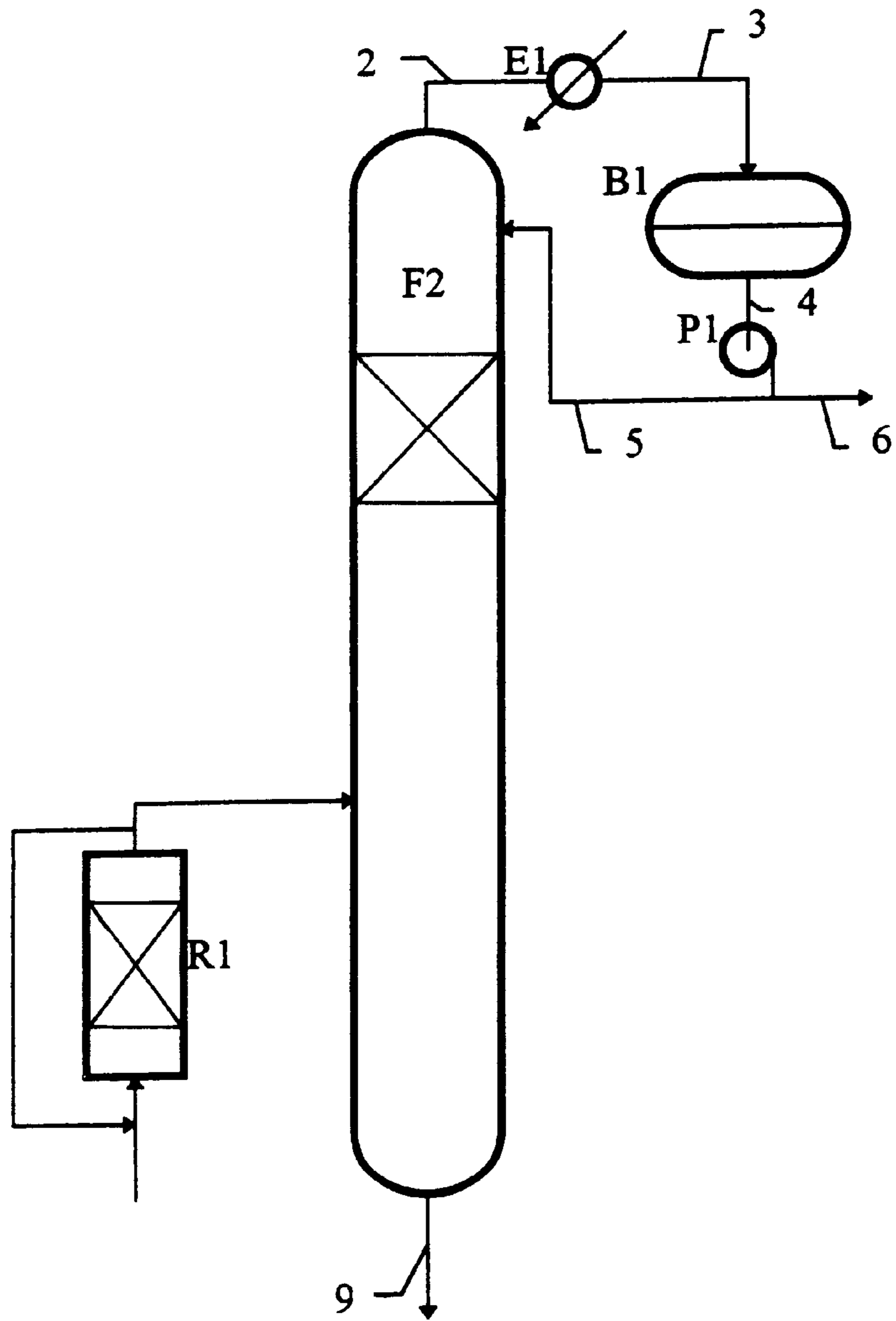
FIG. 3 PRIOR ART
