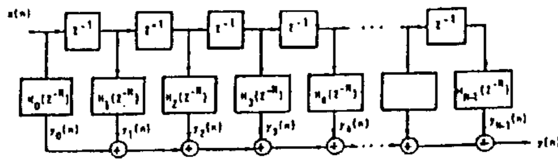
FIGURE 4A. ALL-PASS FILTER STRUCTURE
