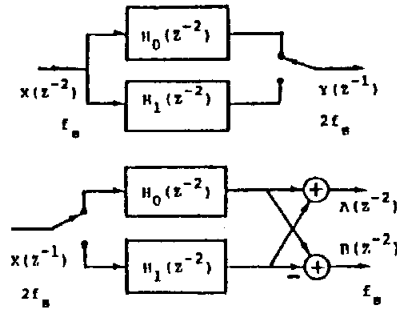
FIGURE 10. RESAMPLING 2-PATH ALL-PASS FILTER
