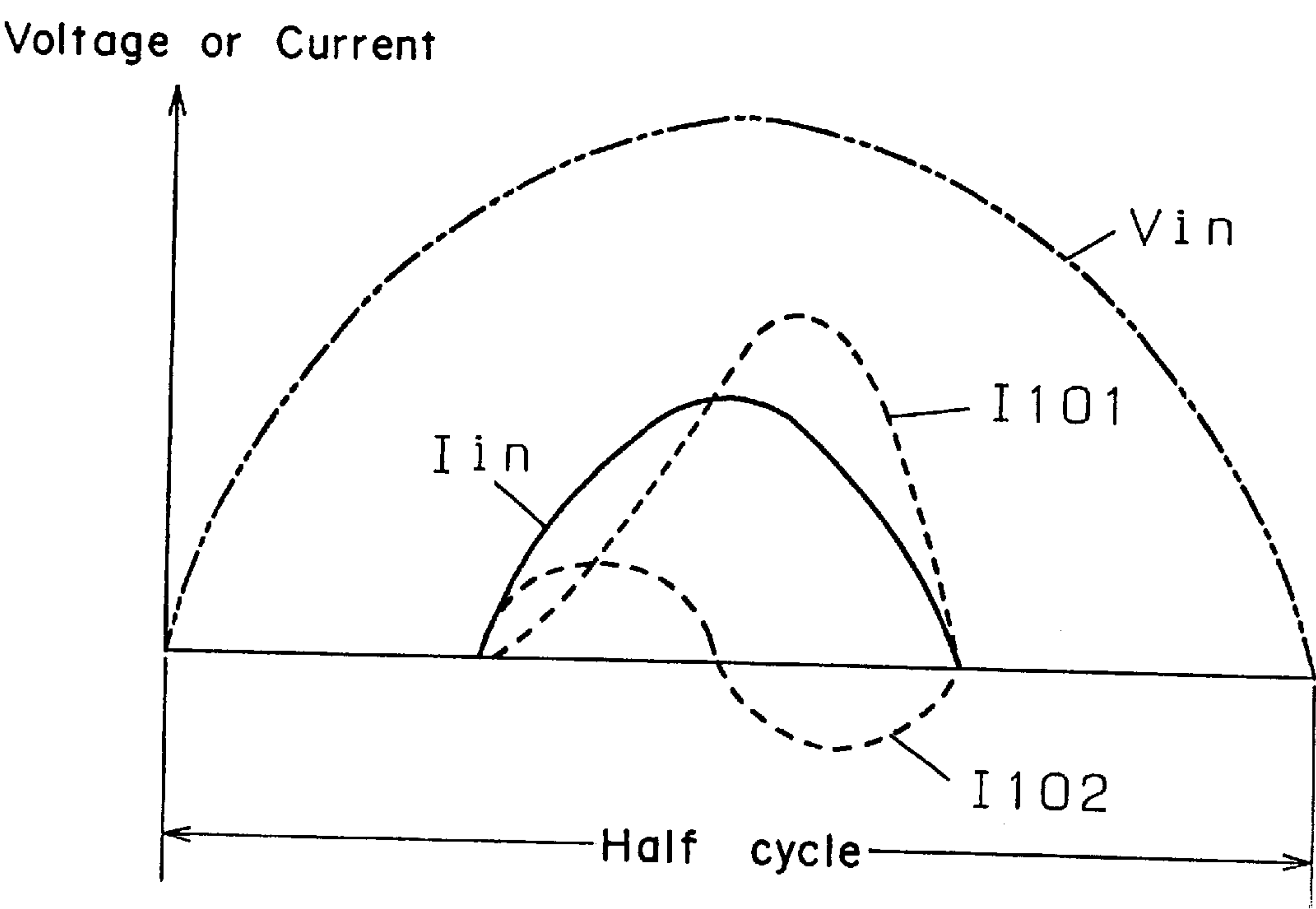
Fig. 20 PRIOR ART
