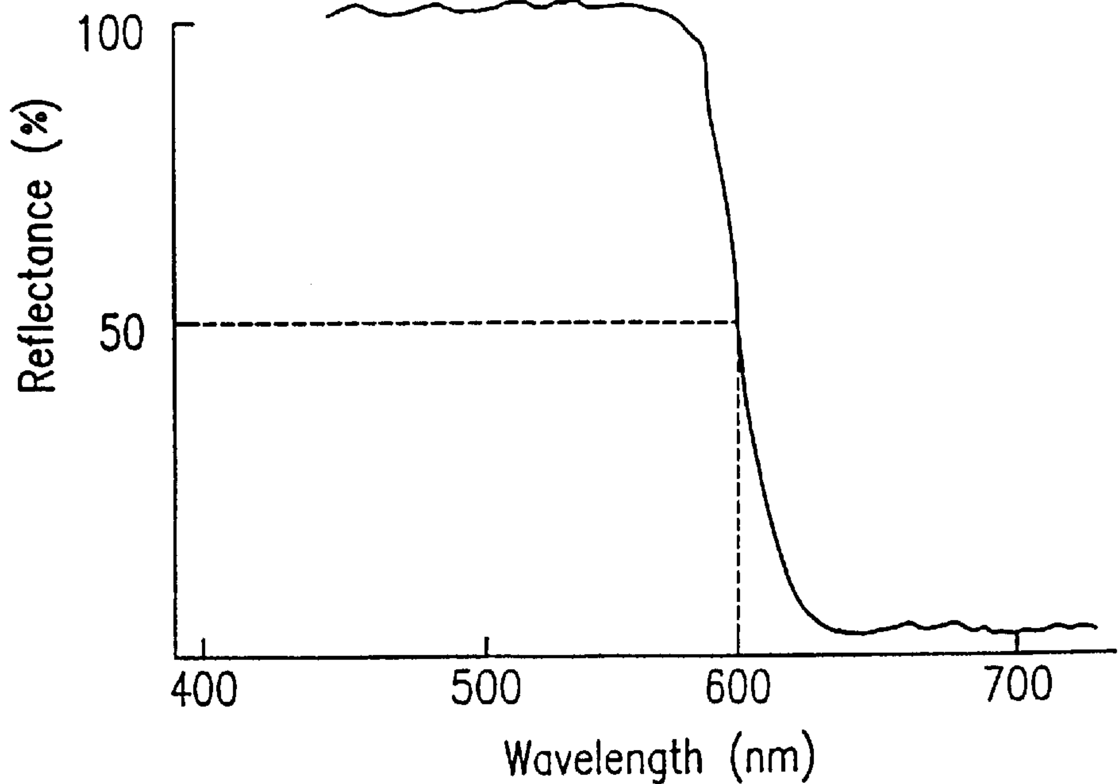
Spectral characteristics of 6-R filter
