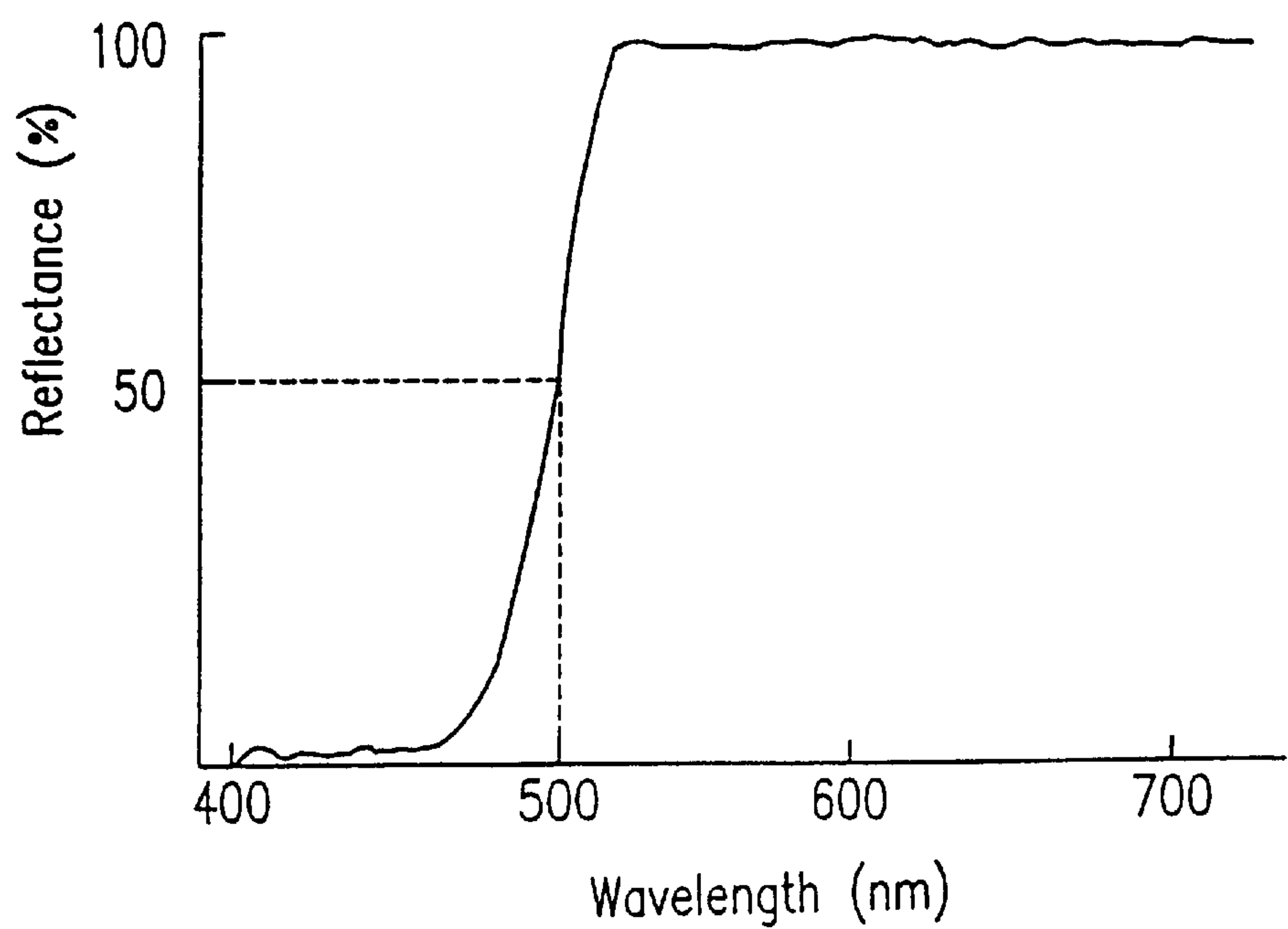
Spectral characteristics of 6-B filter
