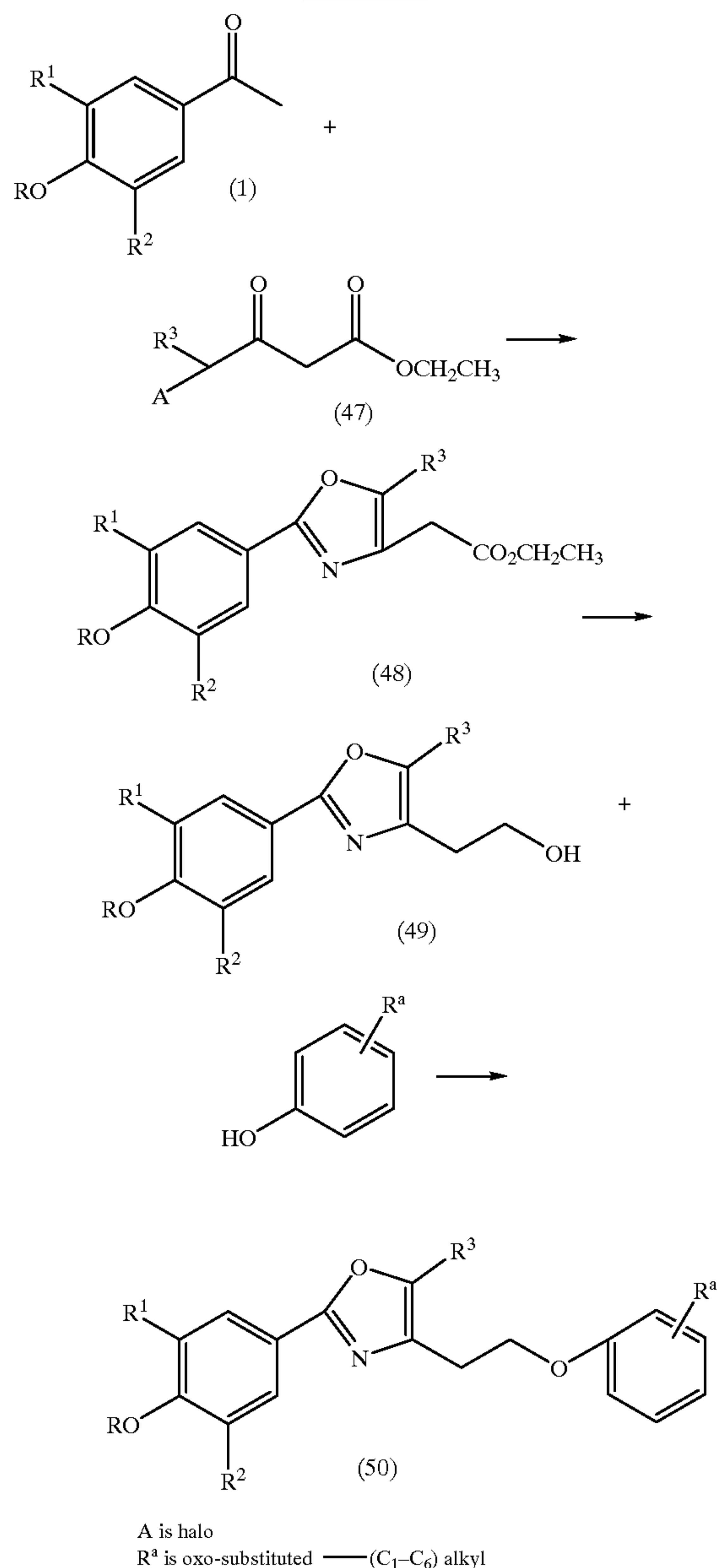
Scheme XII
