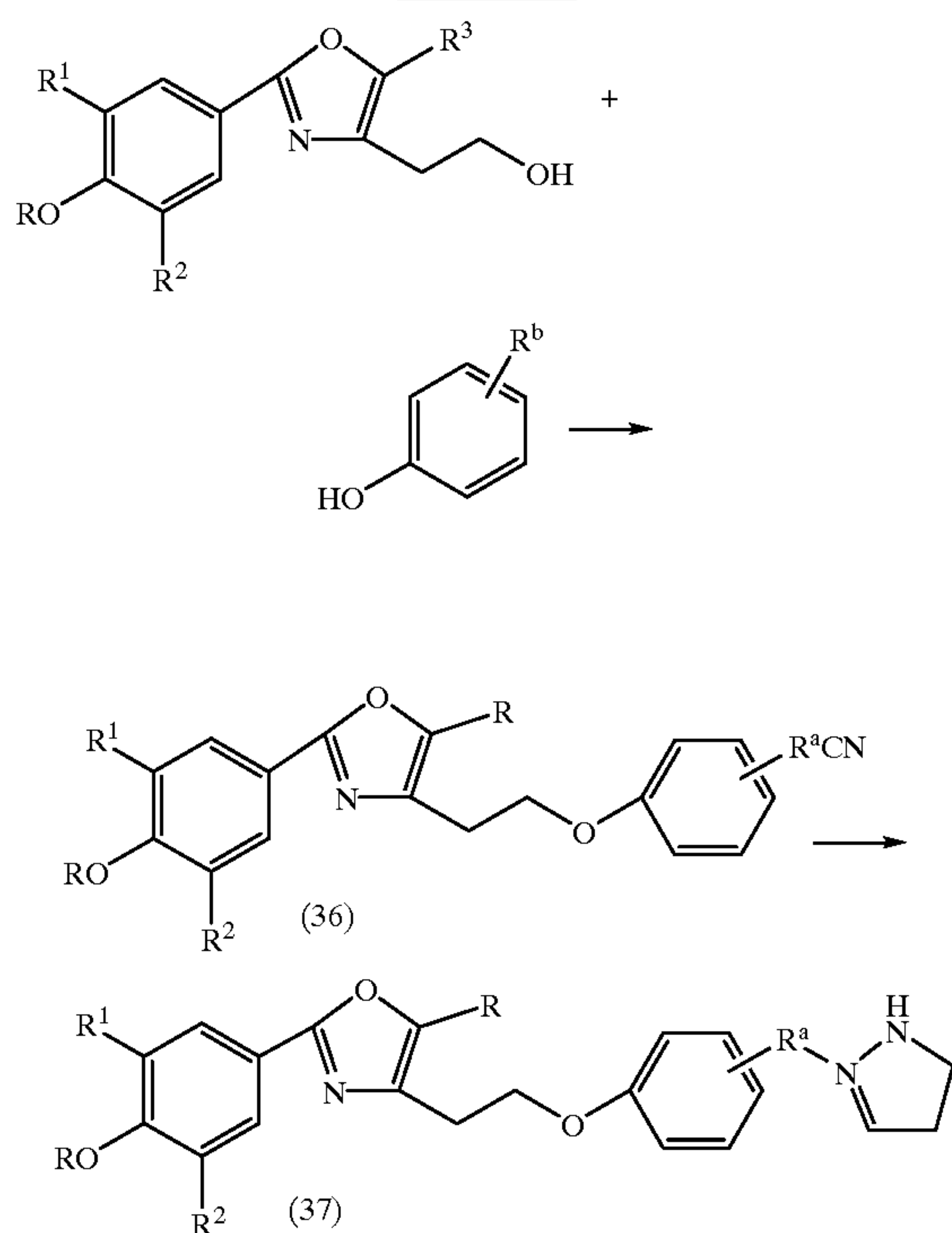
Scheme VIII
