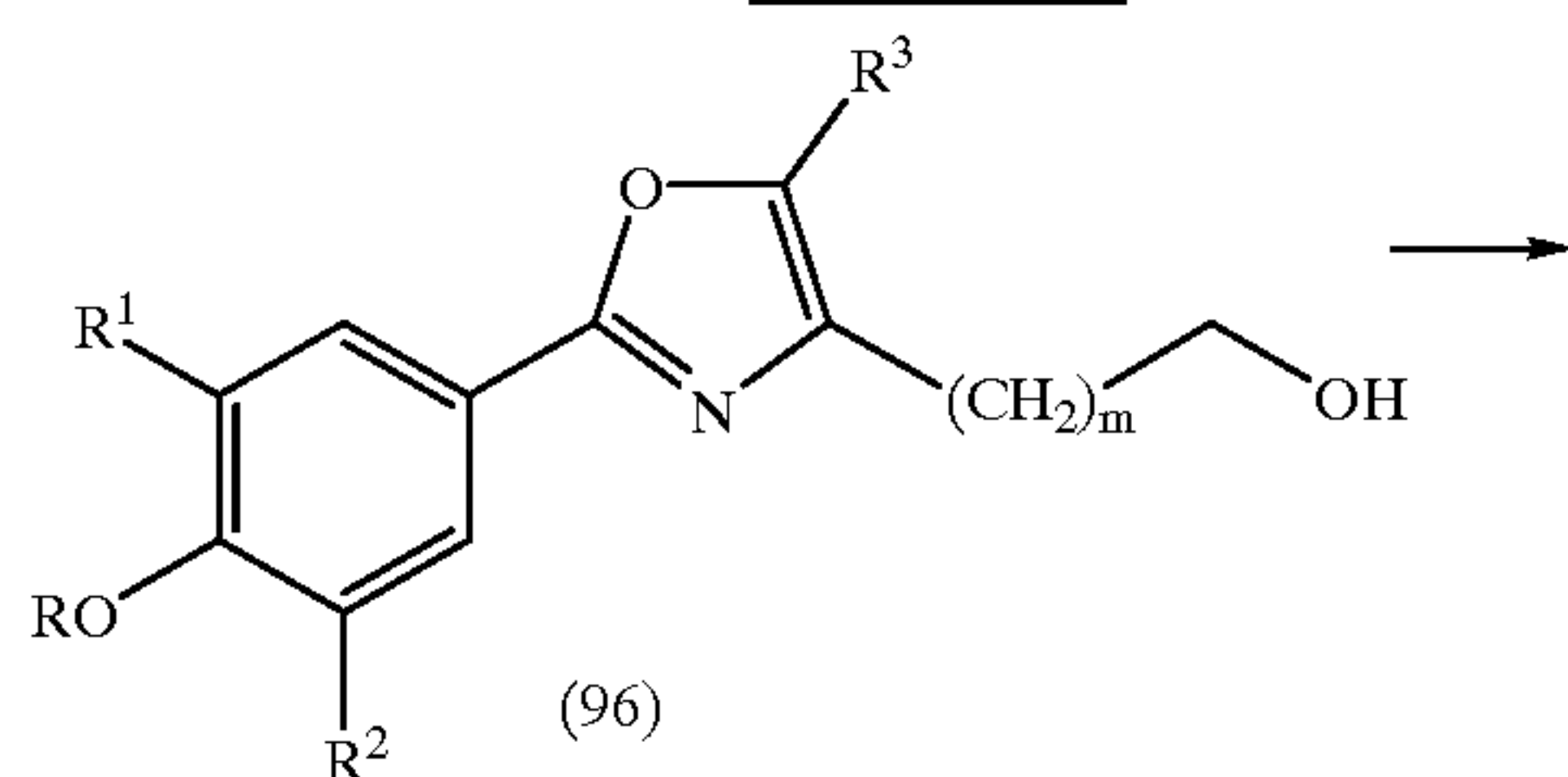
Scheme XXII
