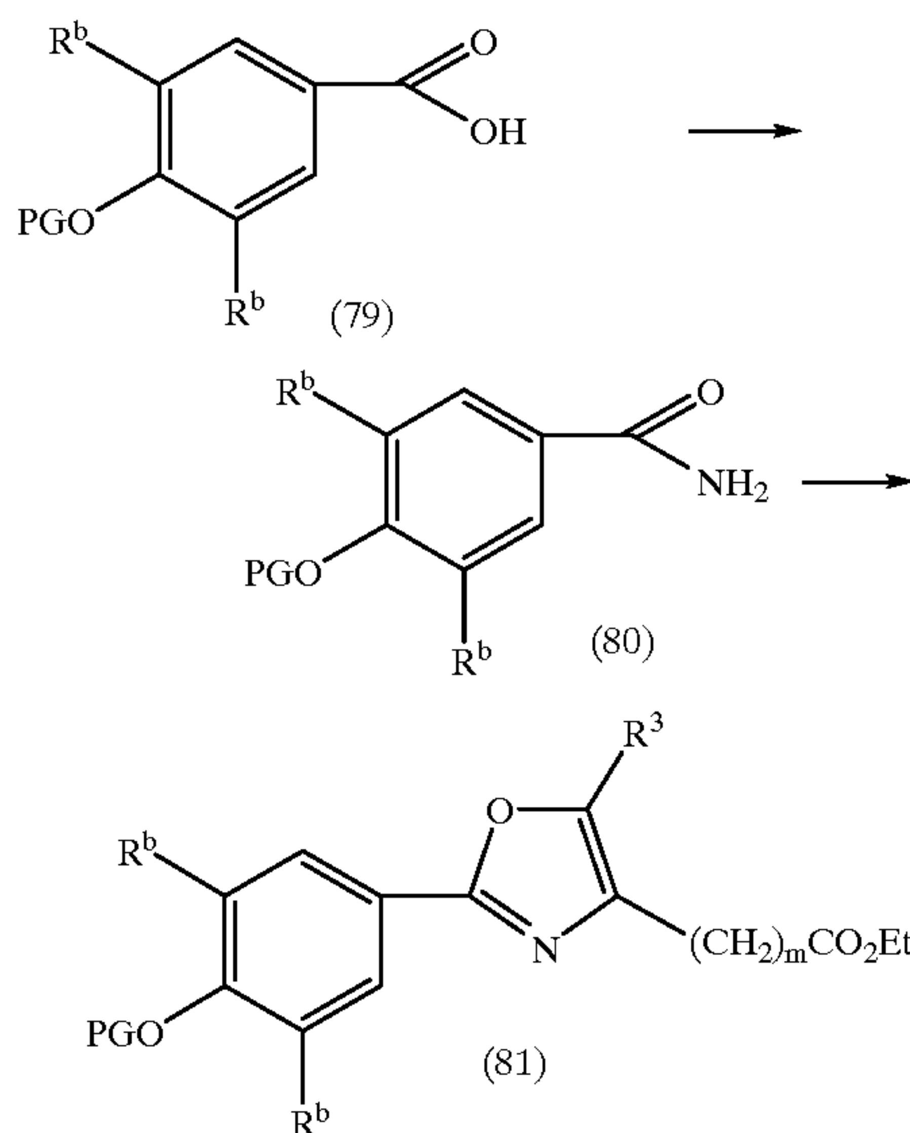
Scheme XVIII
