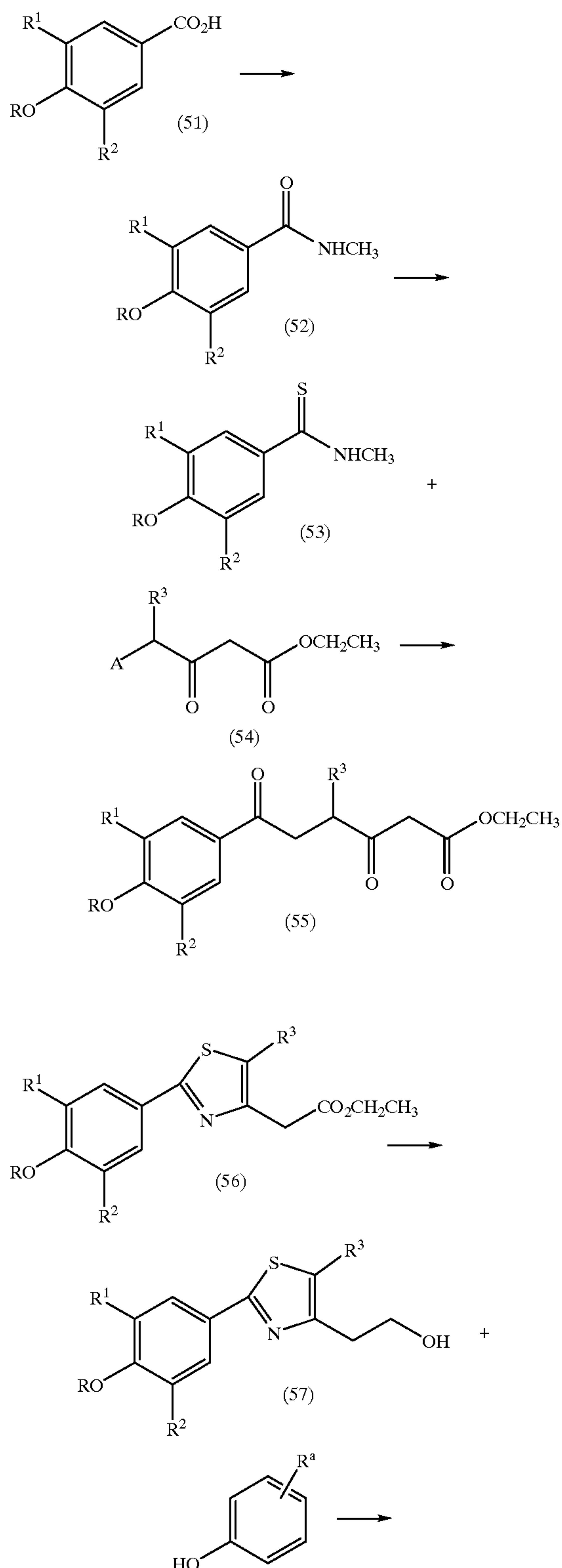
Scheme XIII
