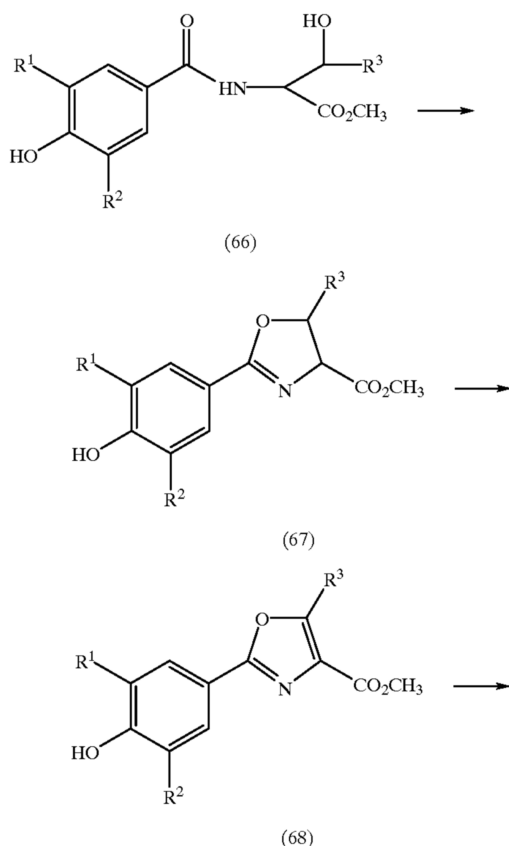
Scheme XV
