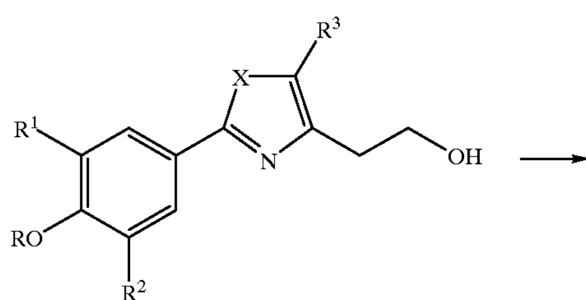
Scheme XIV
