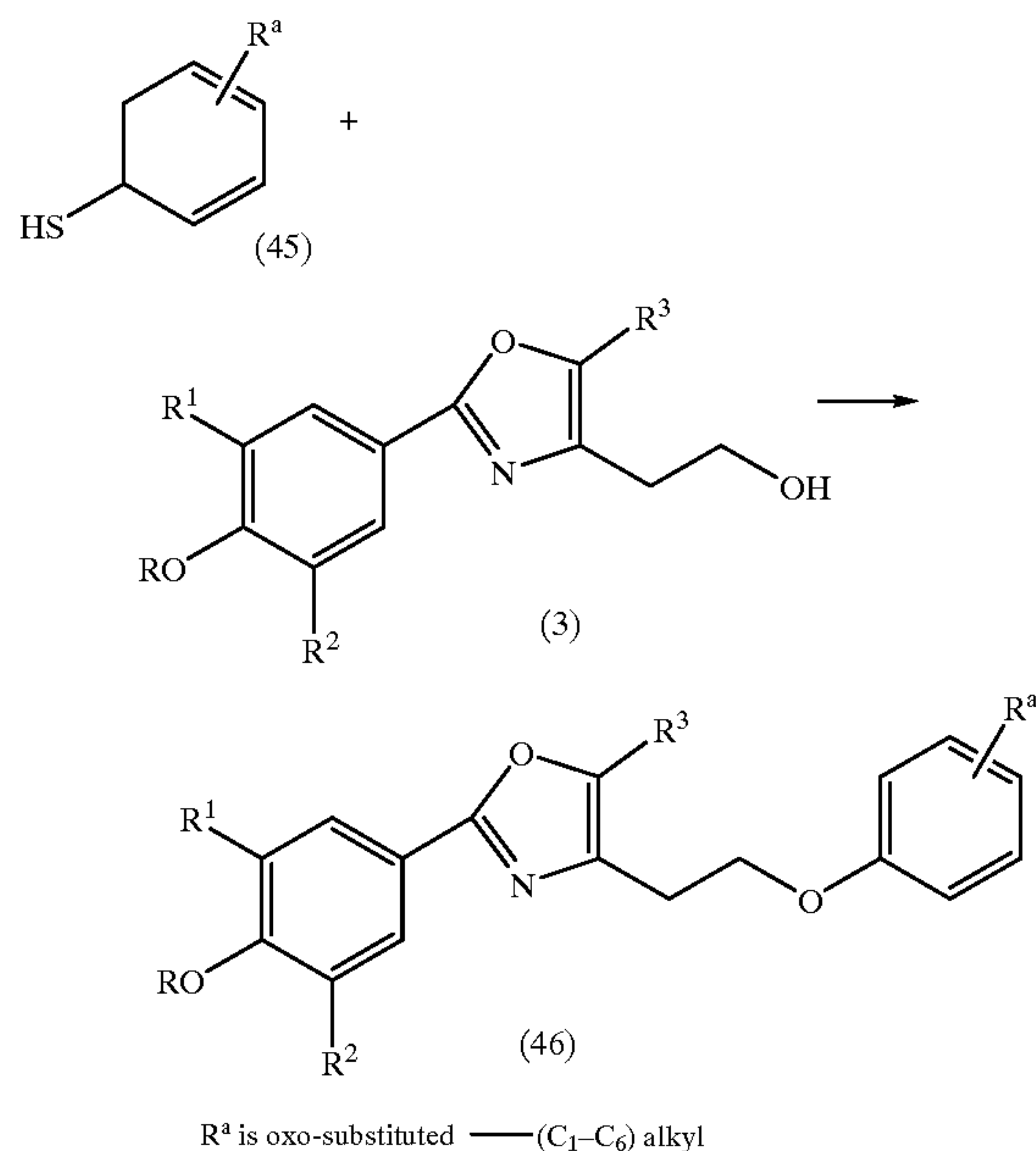
Scheme XI
