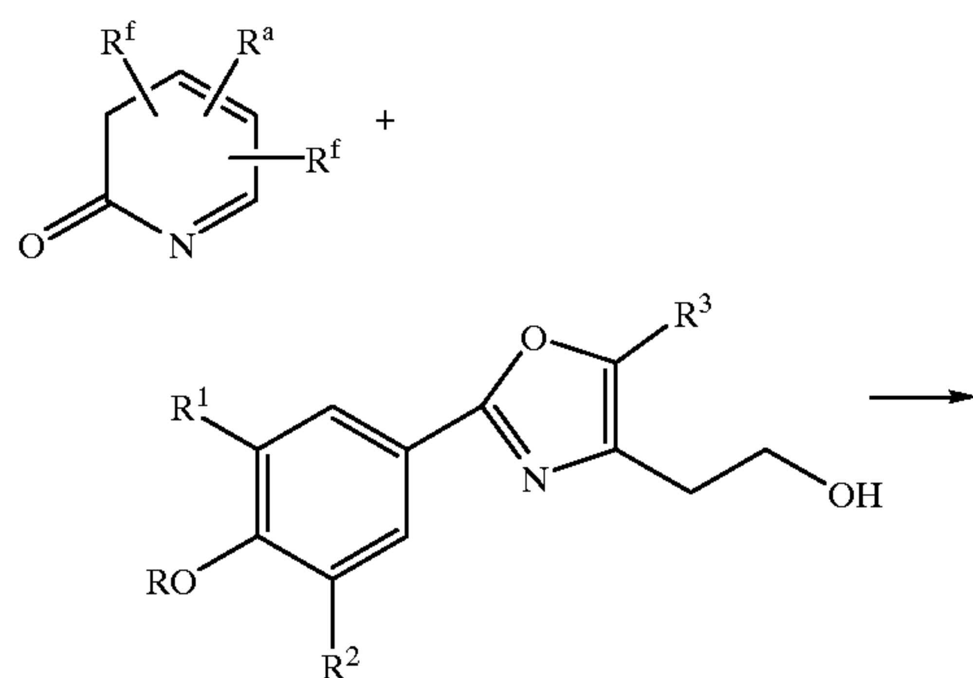
Scheme X
