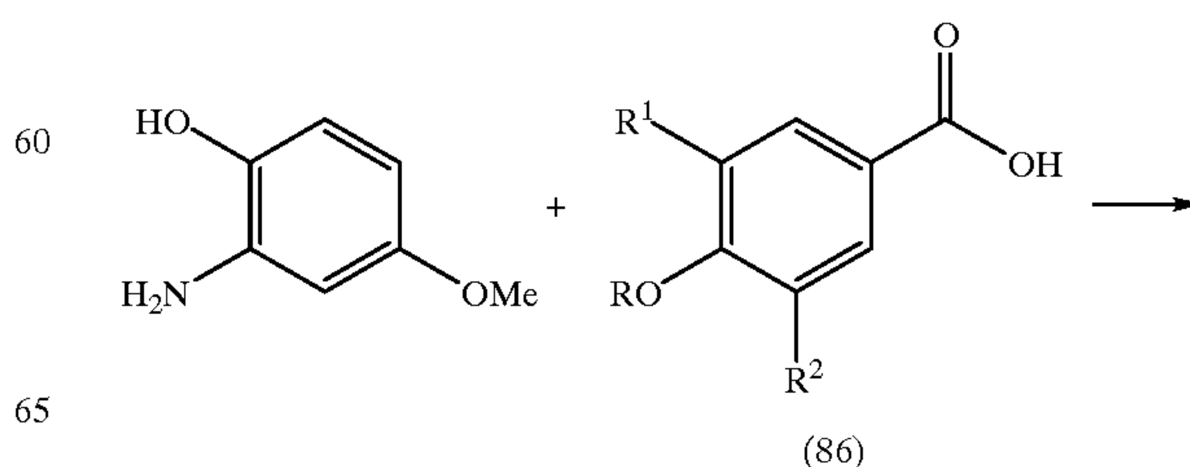
Scheme XIX
