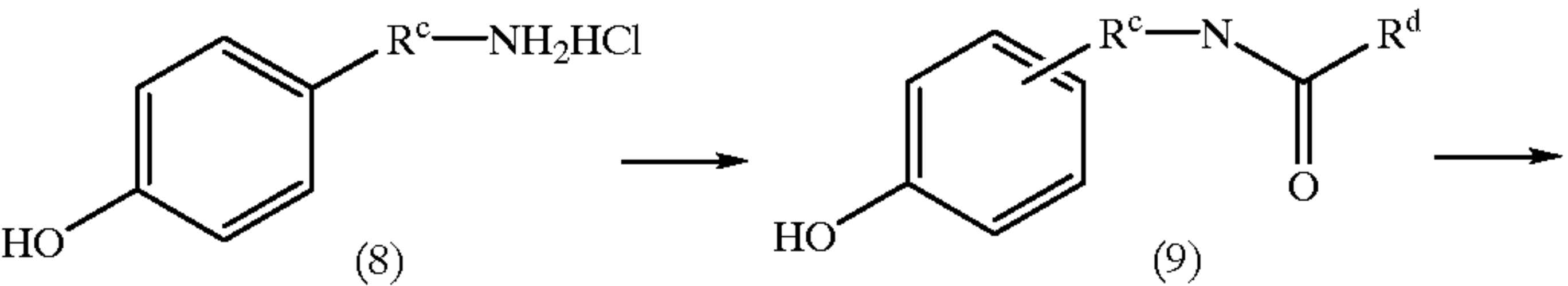
Scheme I (c)
