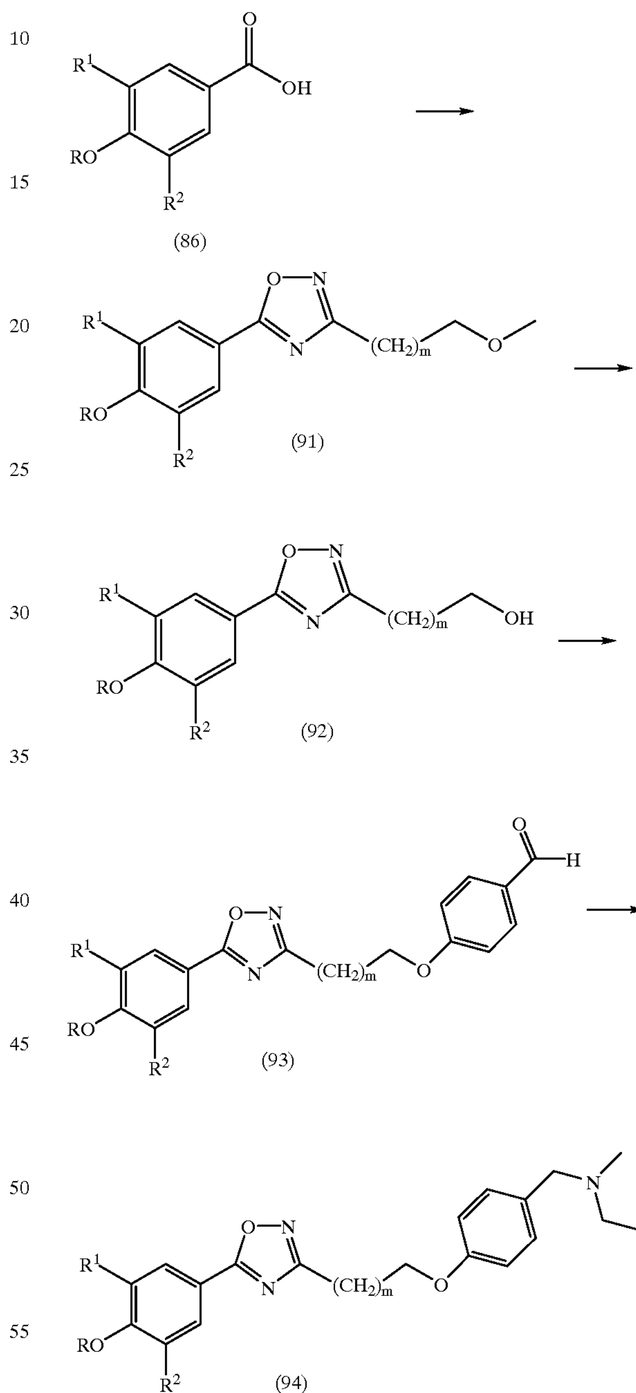
Scheme XX
