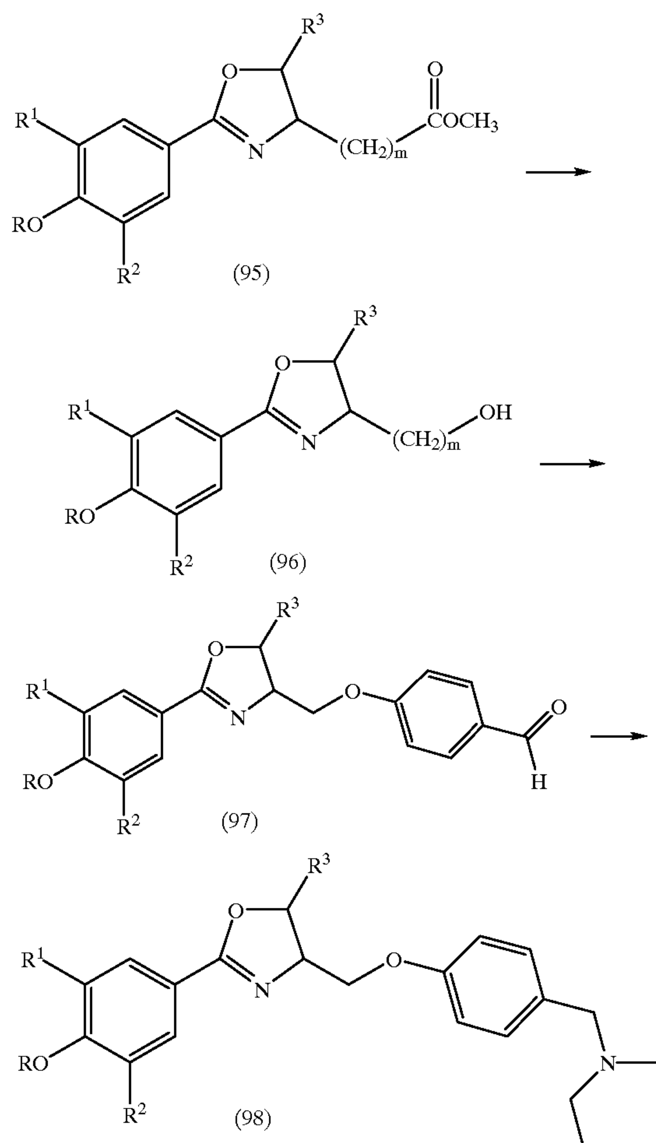
Scheme XXI
