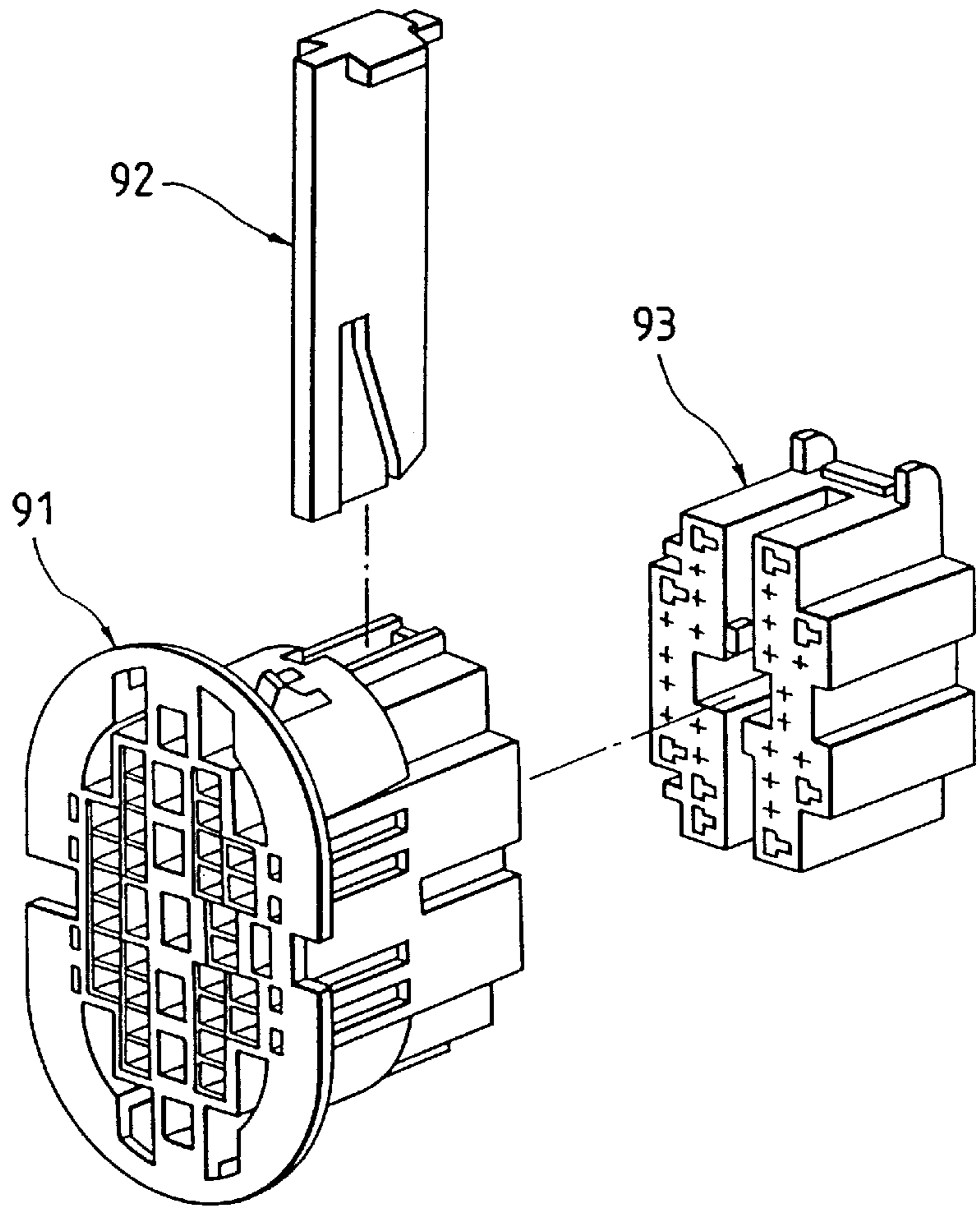
FIG. 17 PRIOR ART
