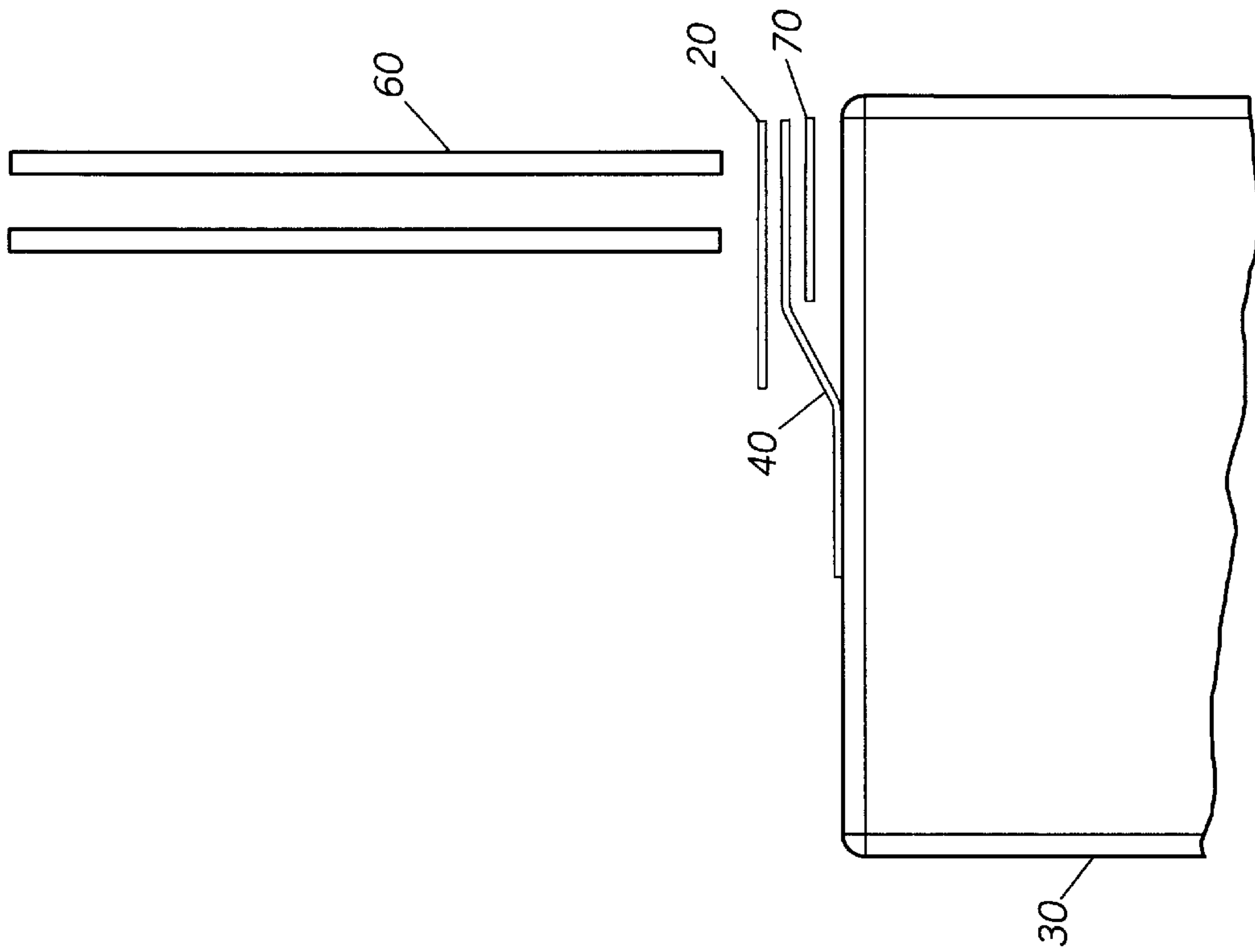
FIG. 3 (PRIOR ART)
