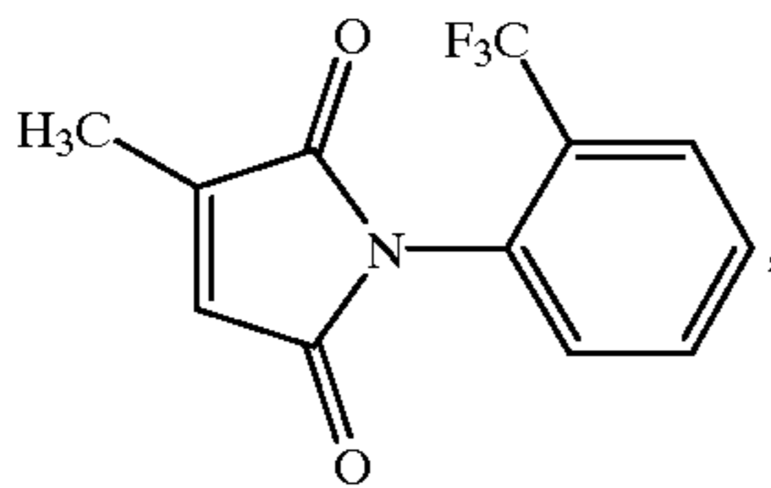
N-(2,4,6-isopropyl-3-maleimide phenyl)maleimide (Id)
