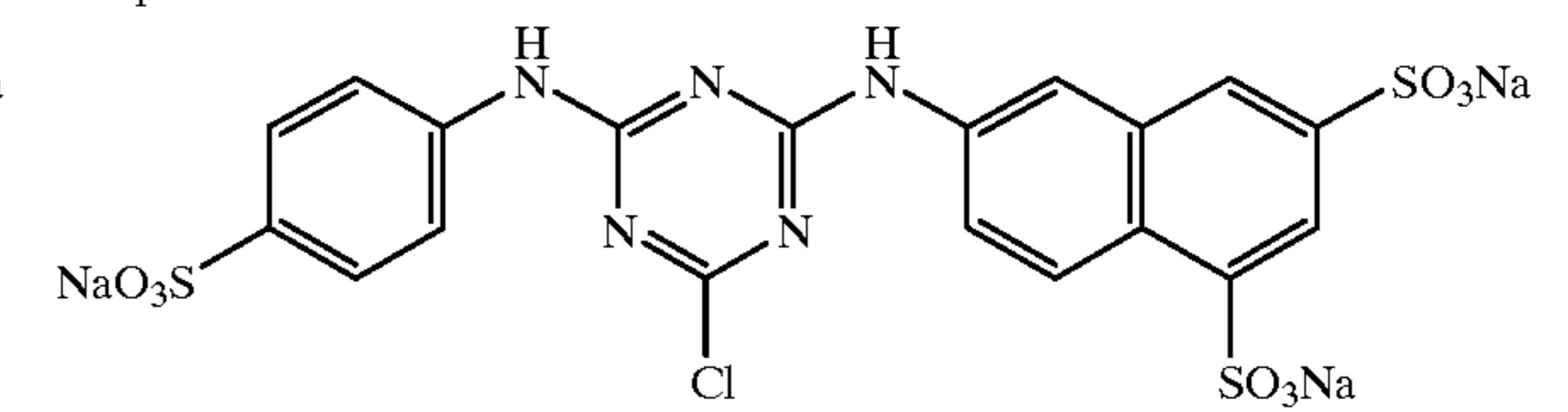
Compound 10:
