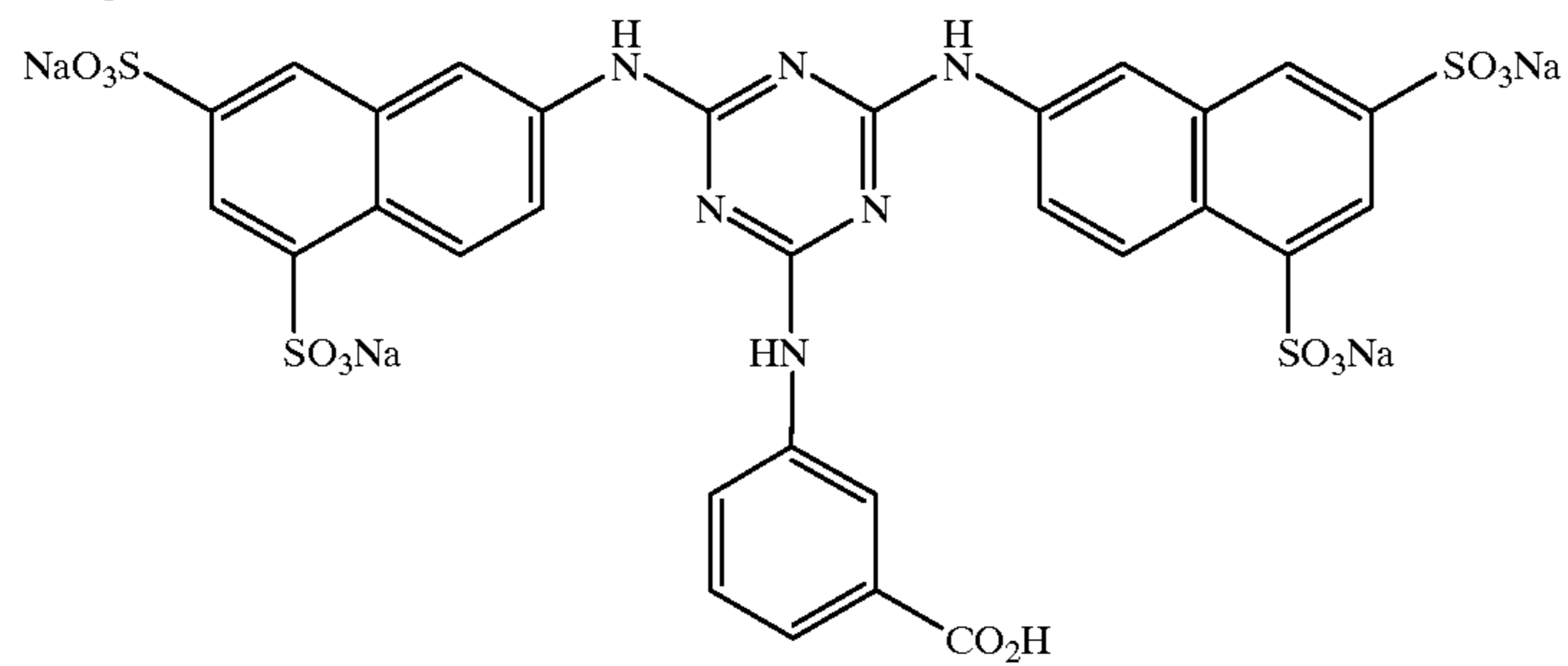
Compound 15:
