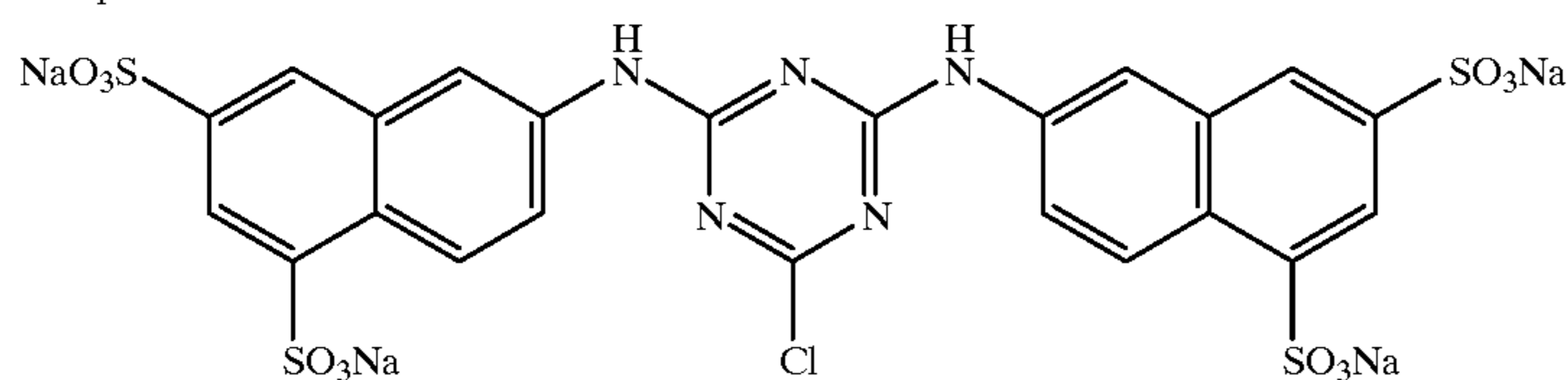
Compound 3:
