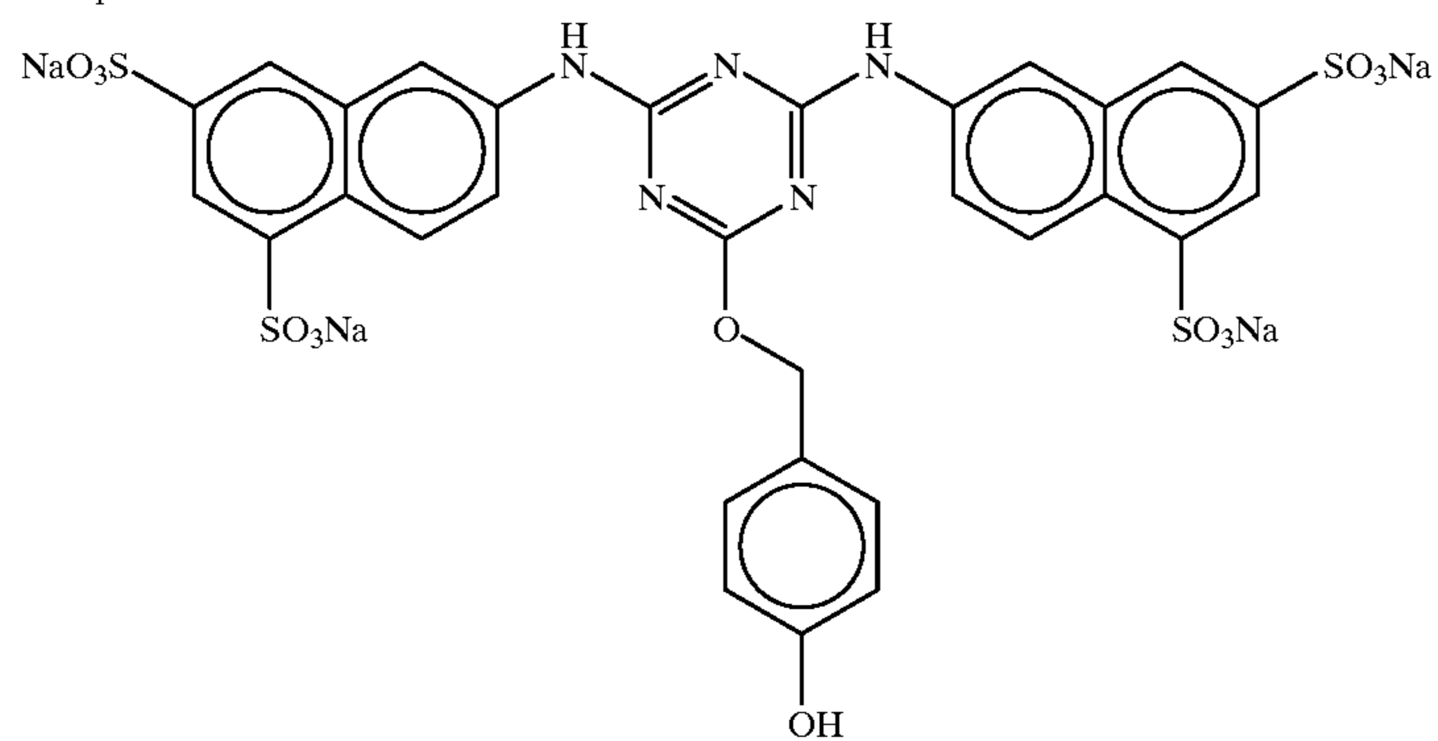
Compound 15:
