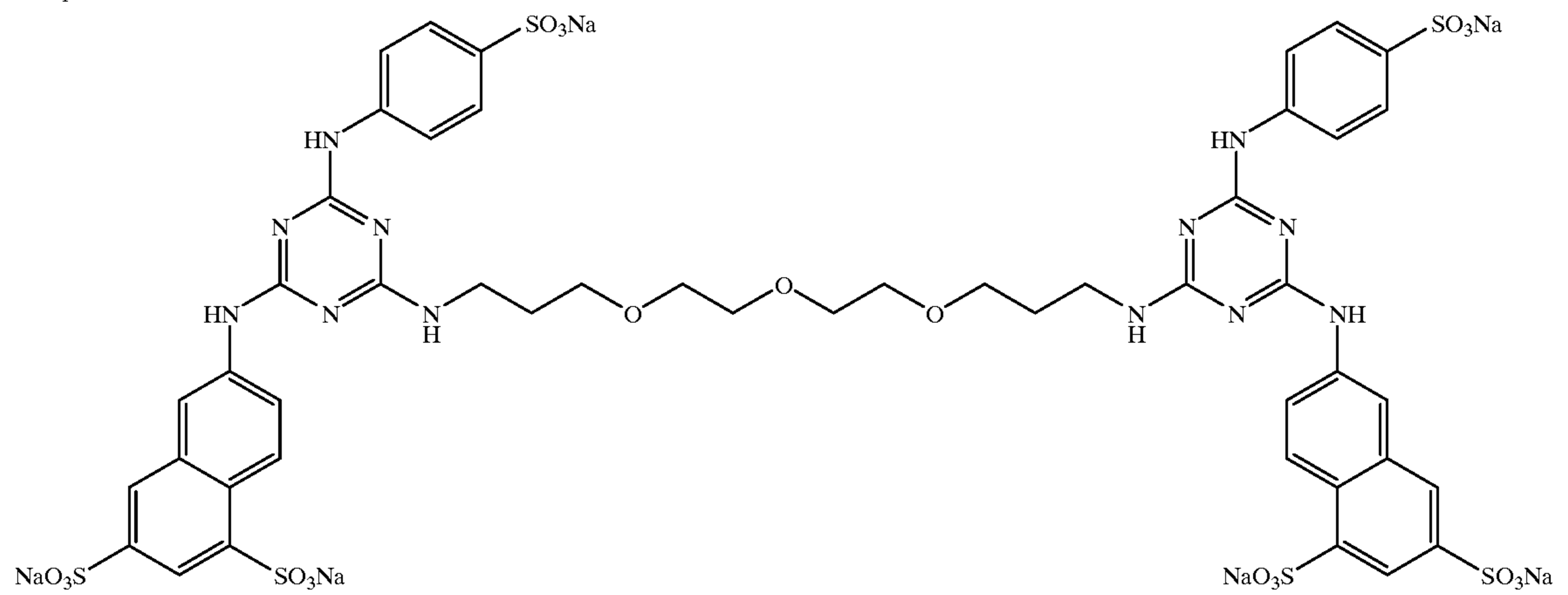
Compound 9:
