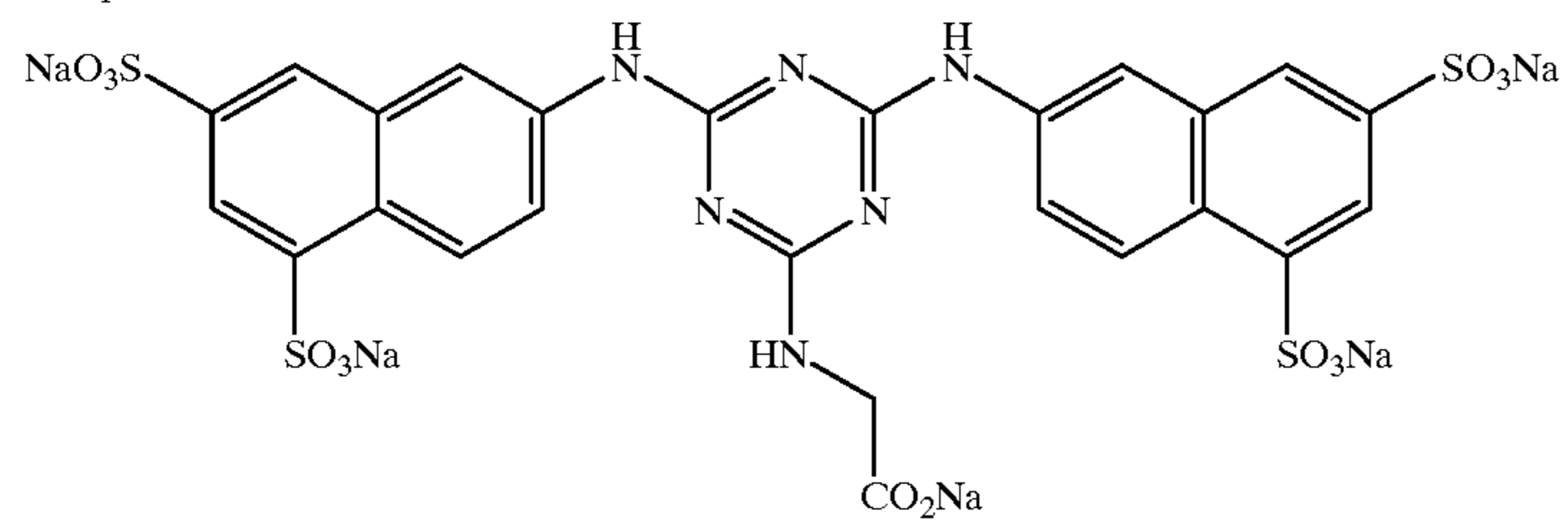
Compound 5:
