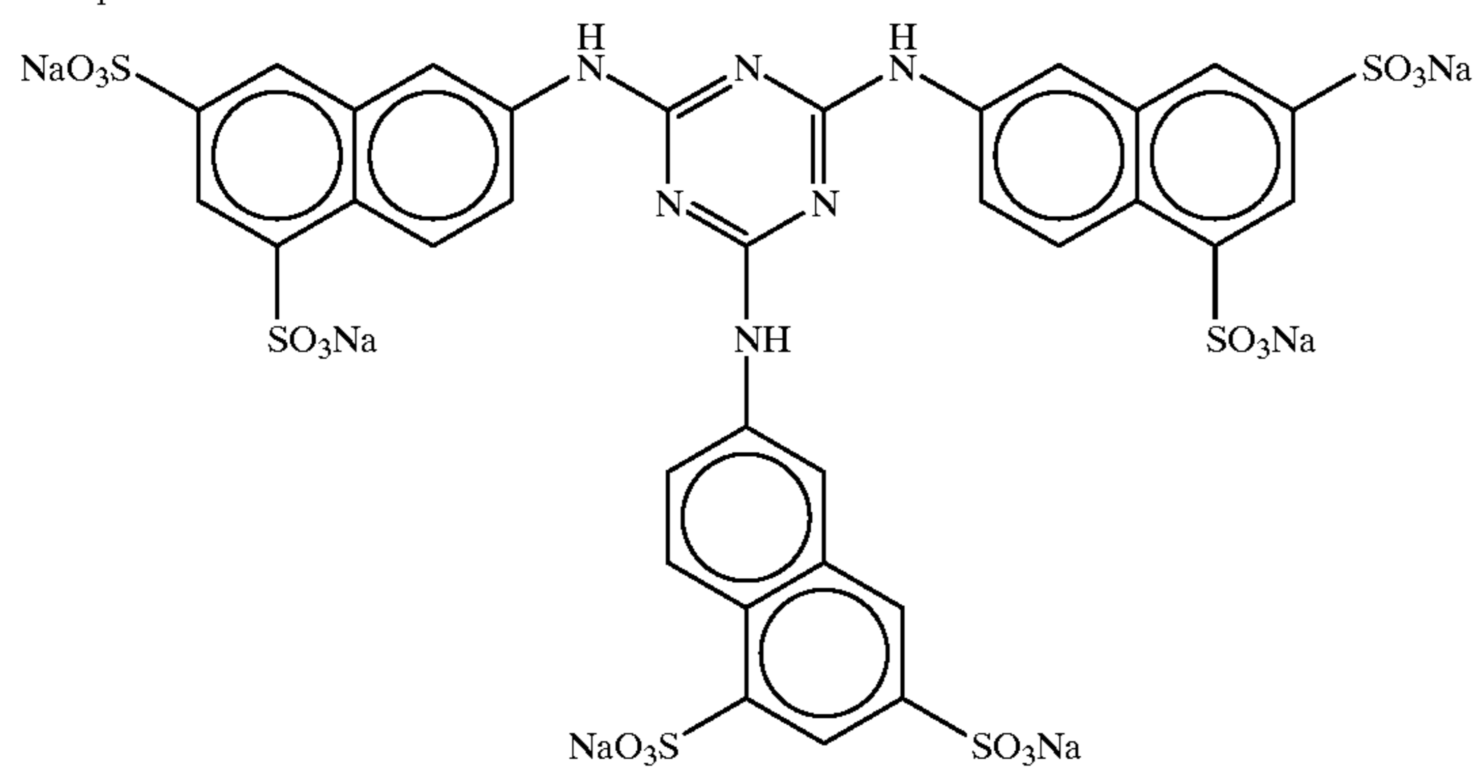
Compound 13:
