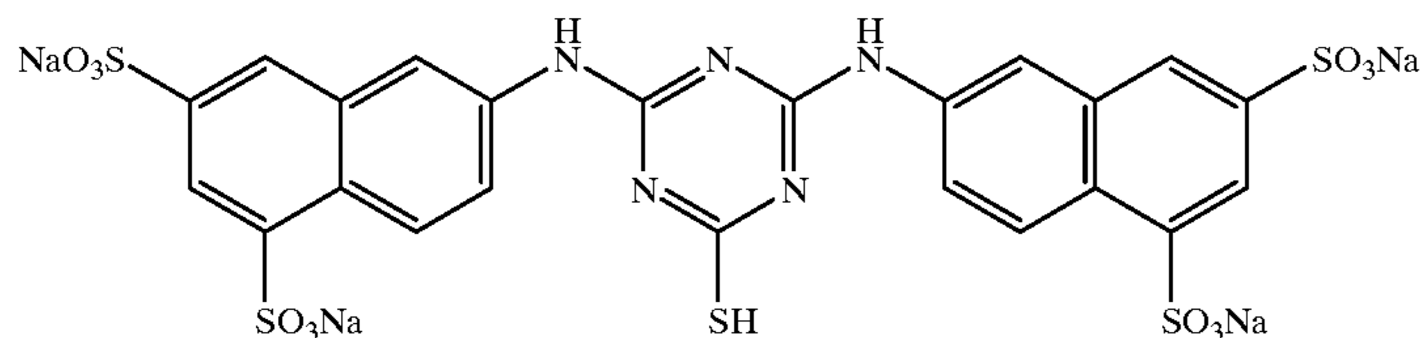
Compound 17:
