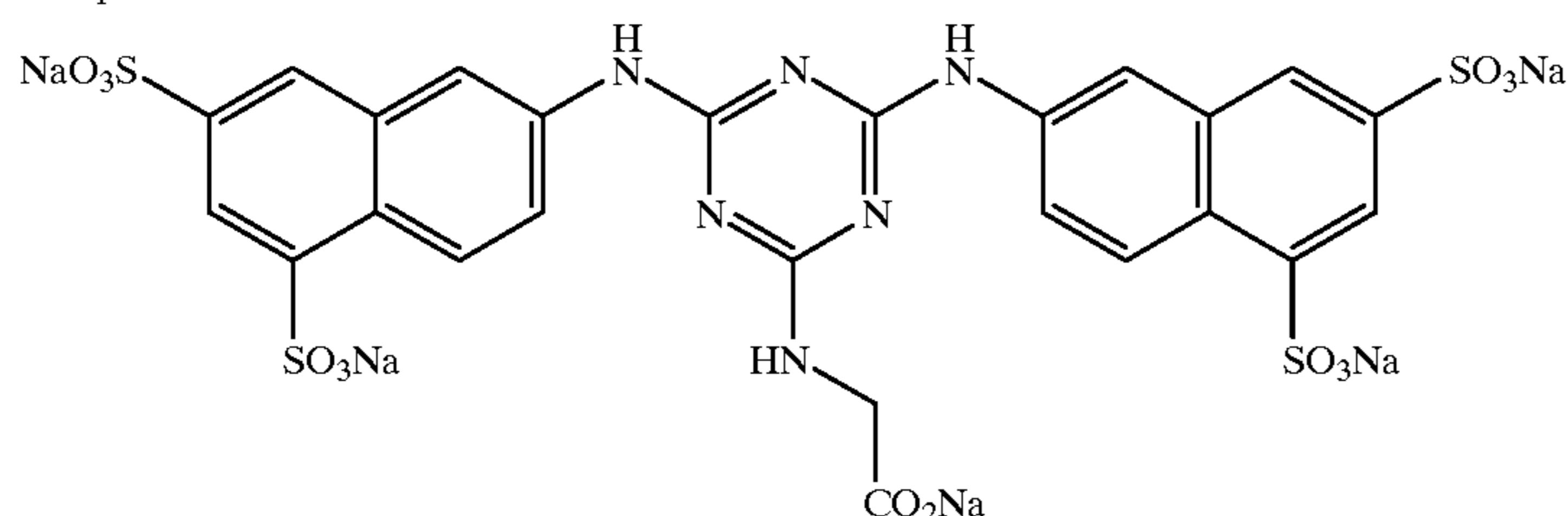
Compound 4:
