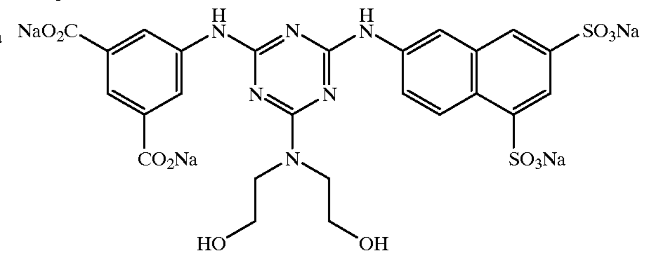
Compound 7:
