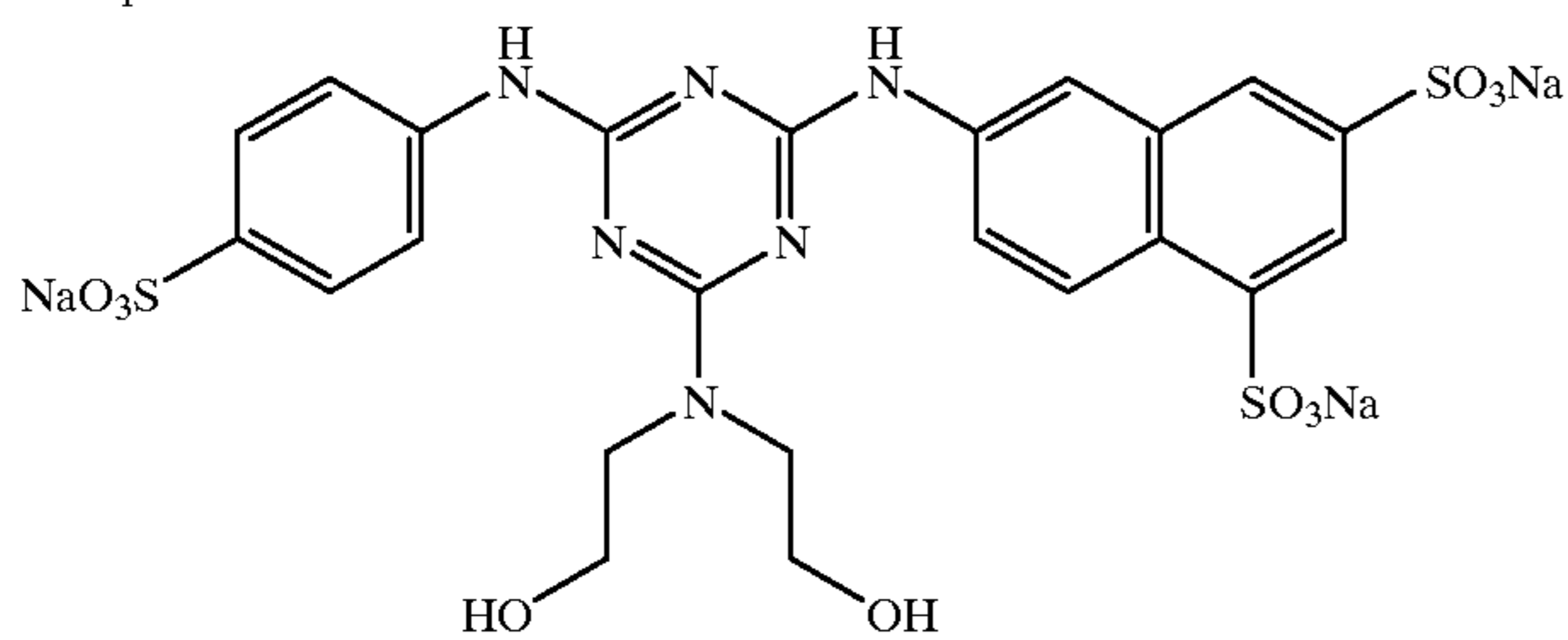
Compound 9:
