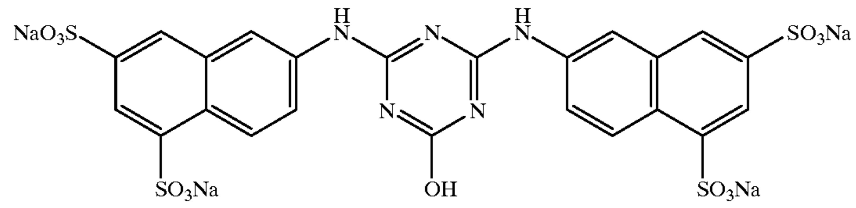
Compound 4:
