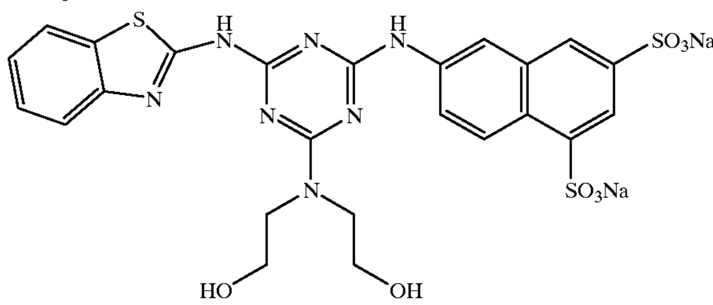
Compound 8:
