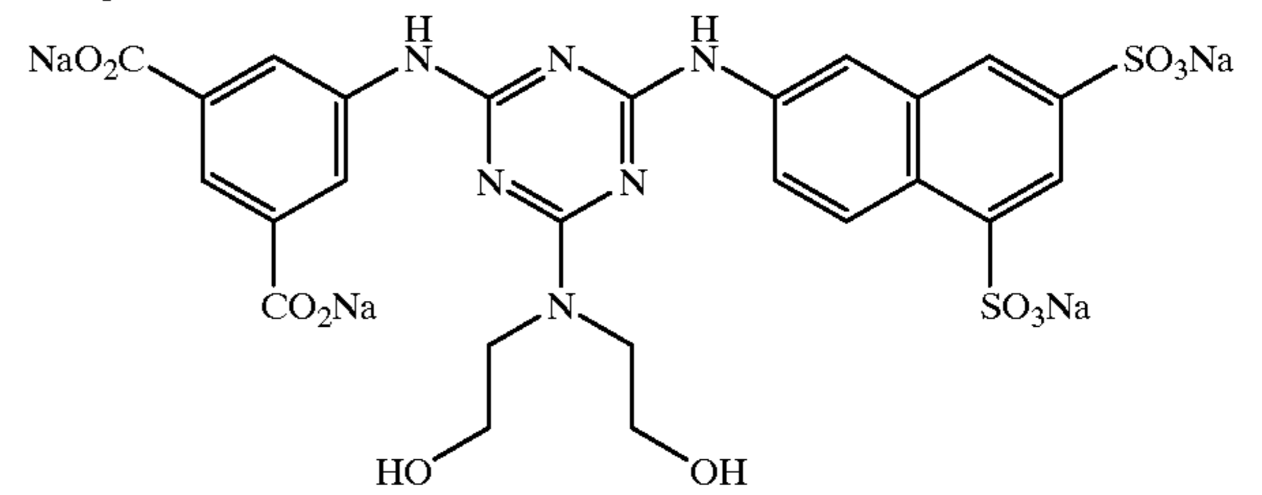
Compound 7:
