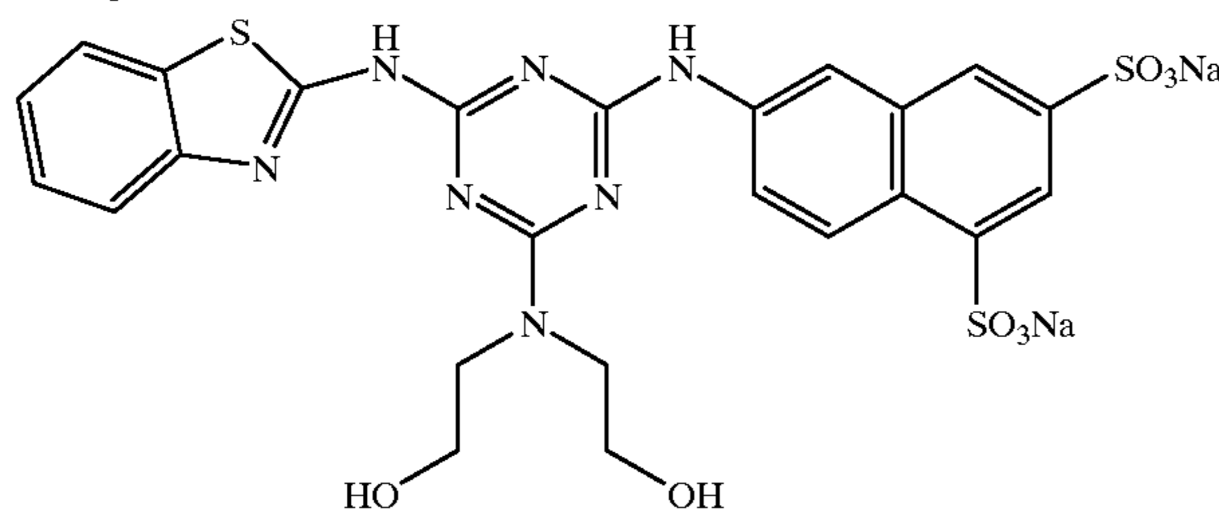
Compound 6:
