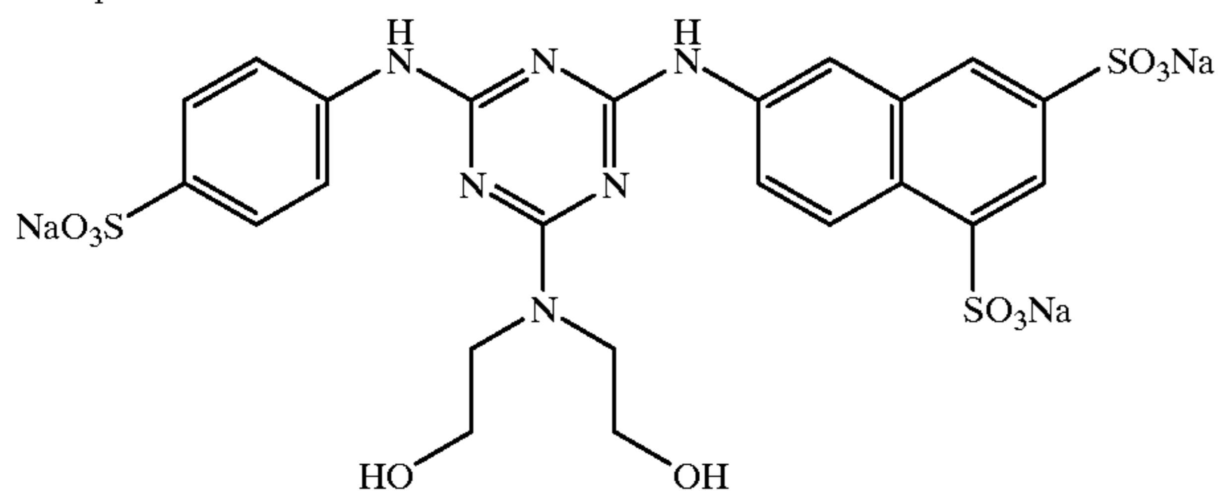
Compound 9:
