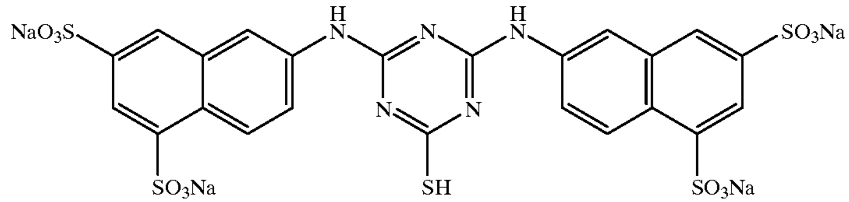
Compound 17:
