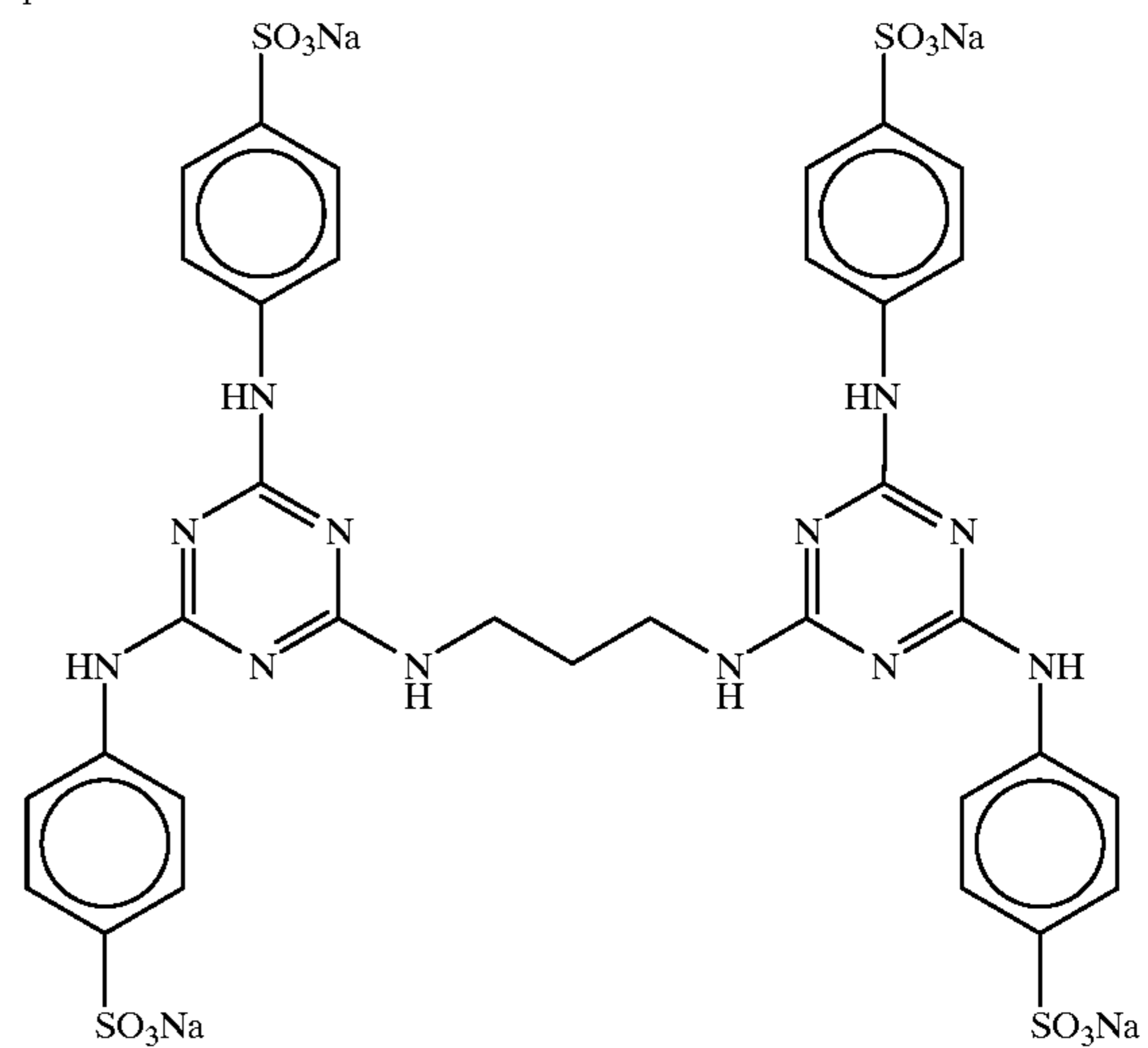
Compound 12:
