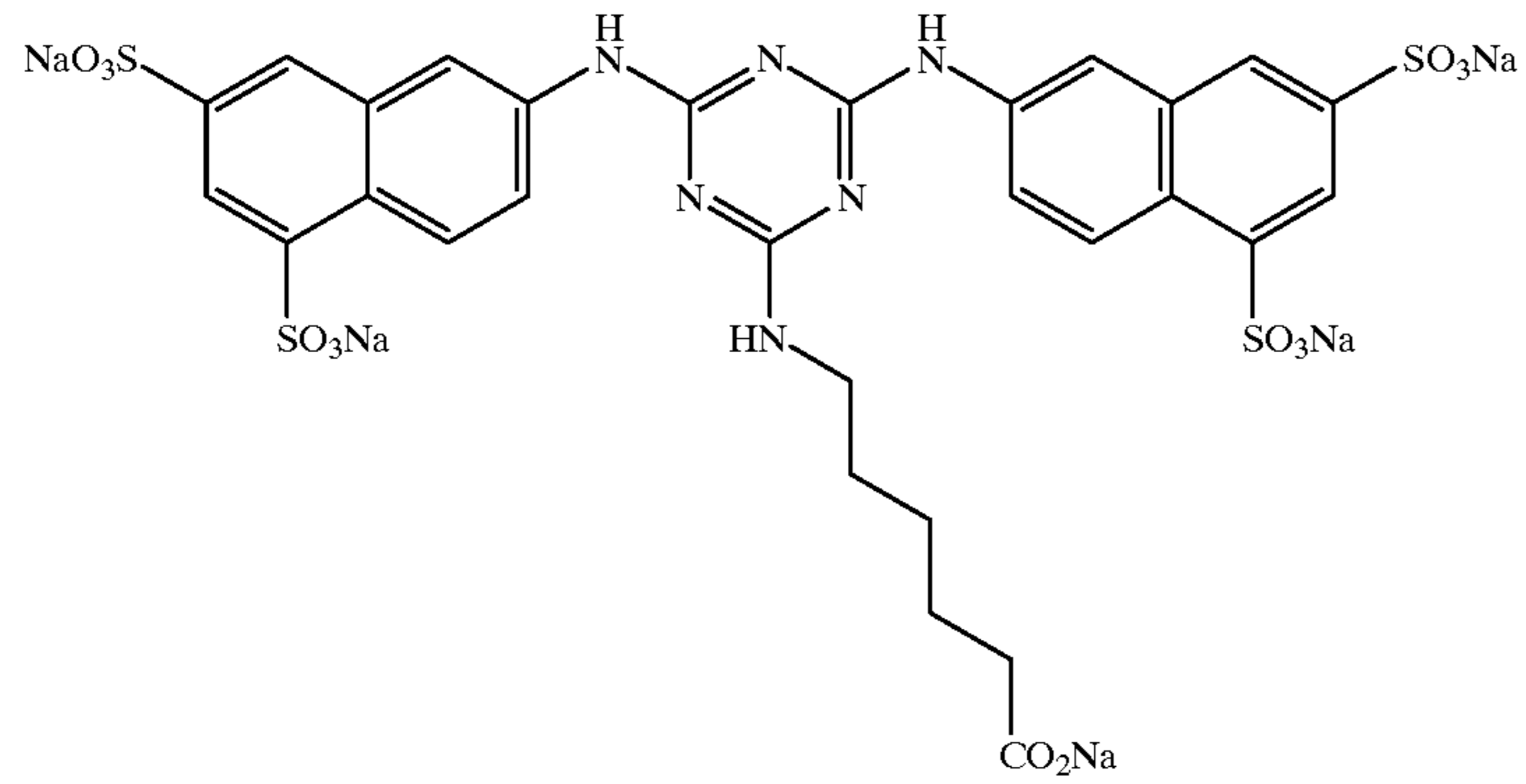
Compound 6:
