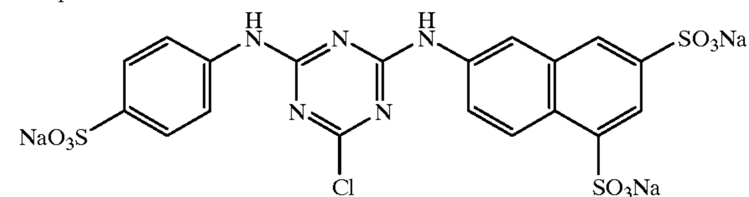
Compound 10:
