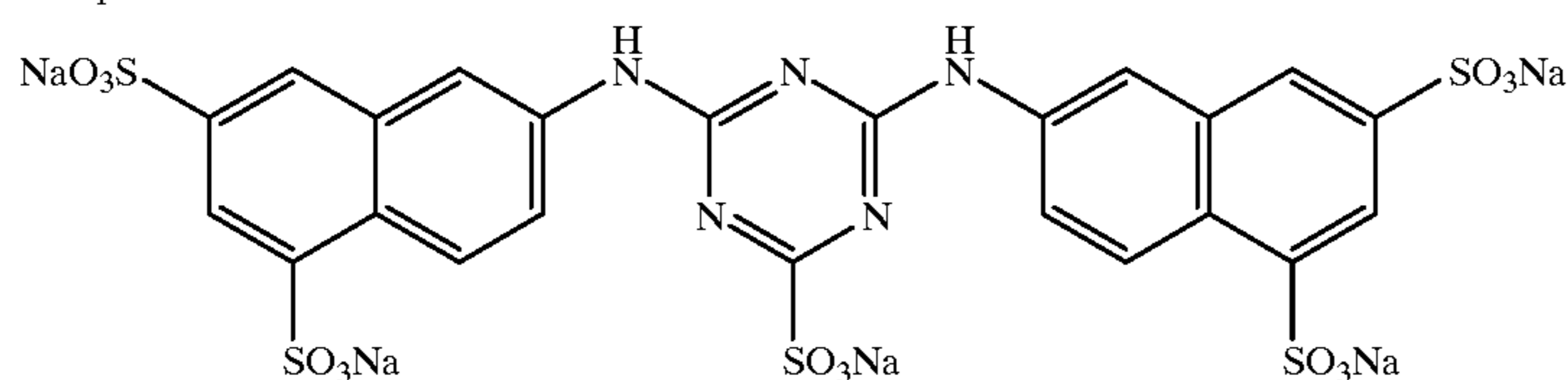
Compound 1:
