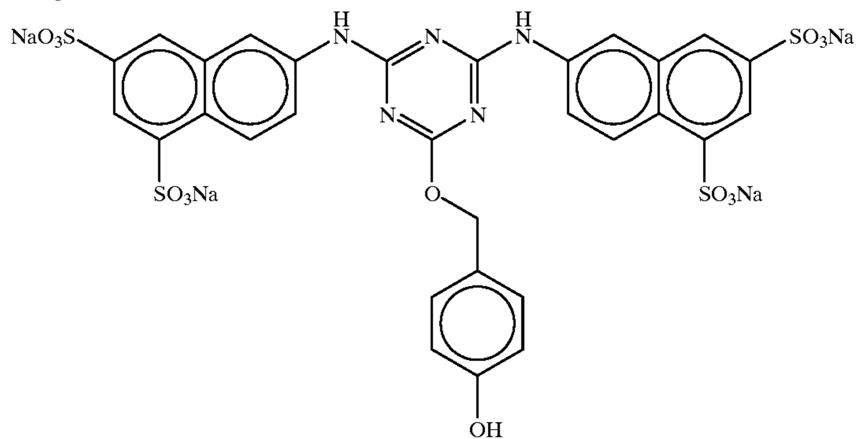
Compound 15:
