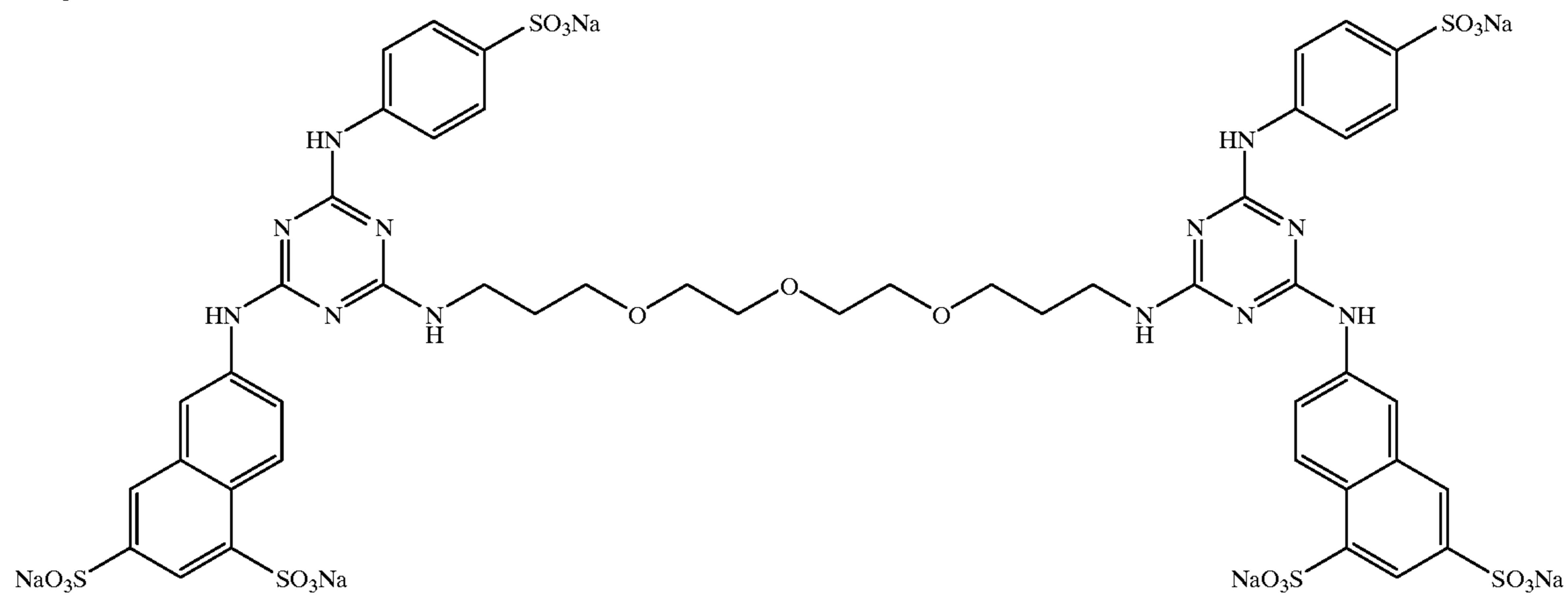
Compound 9:
