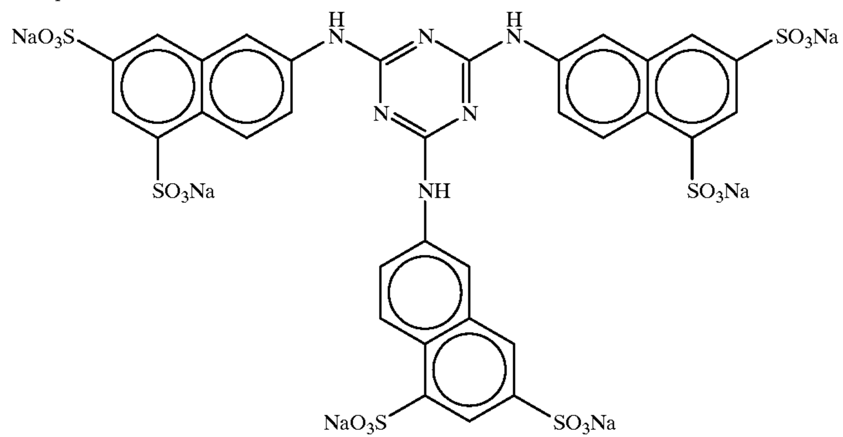
Compound 14:
