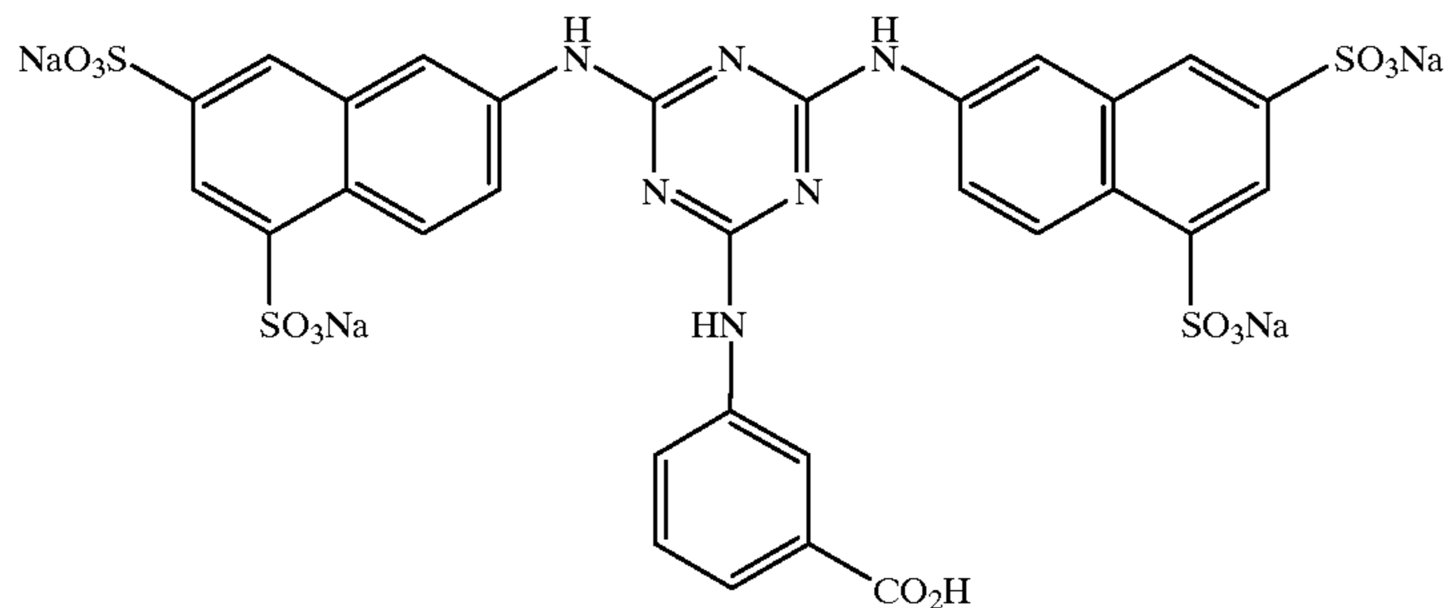
Compound 16:
