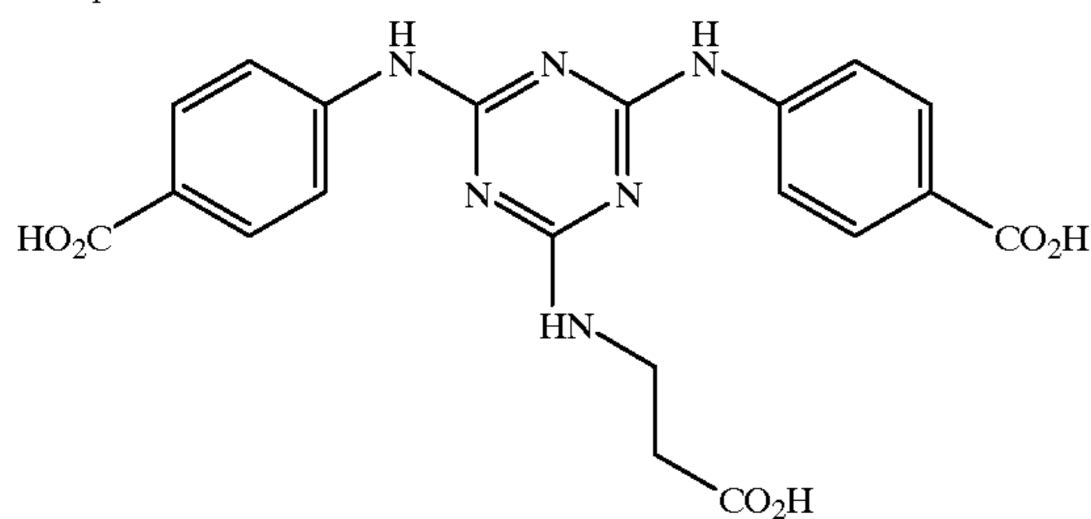
Compound 17:
