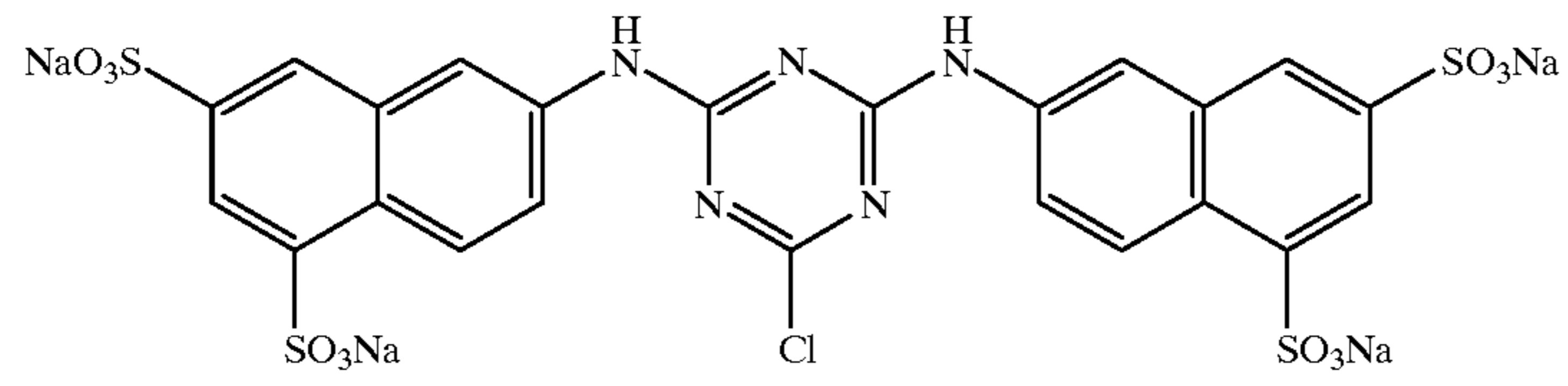
Compound 3:
