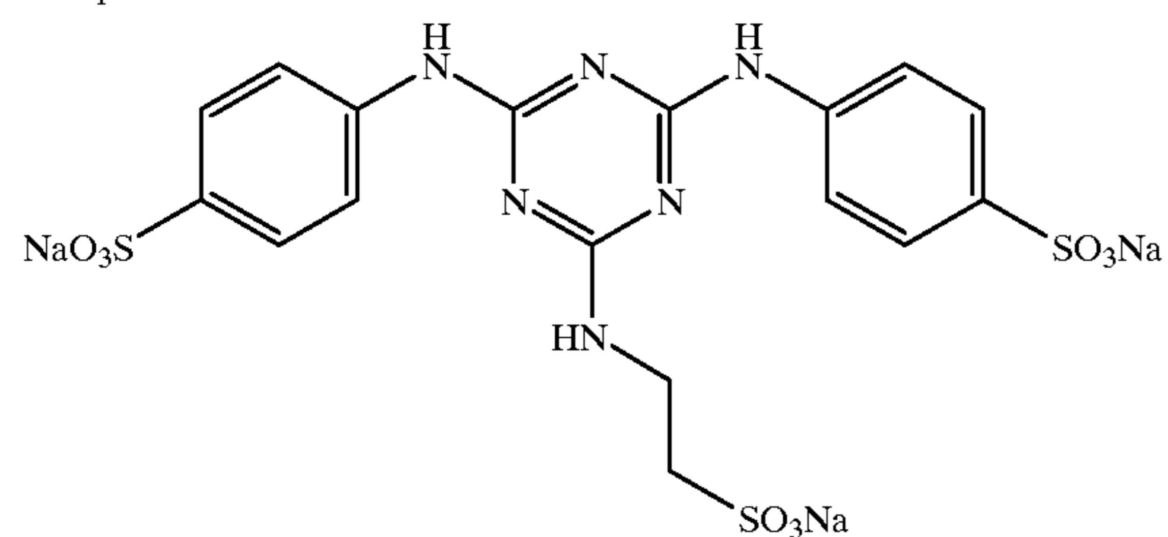
Compound 11:
