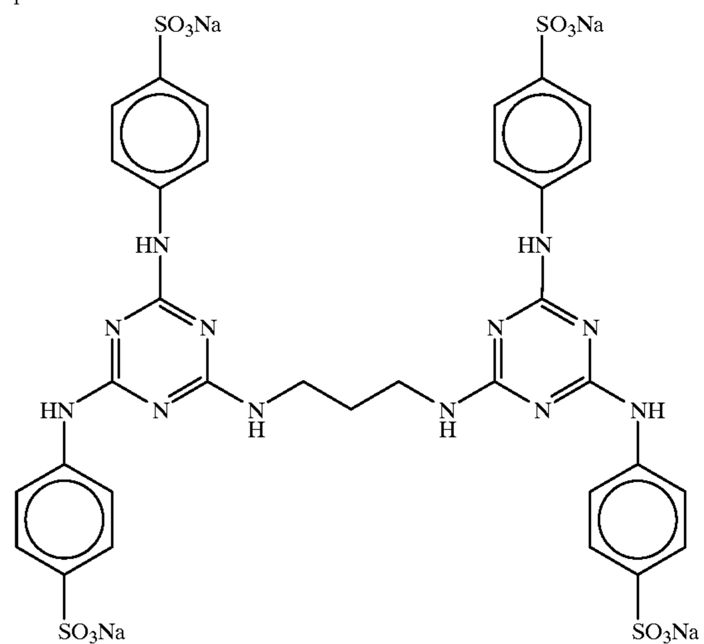
Compound 12:
