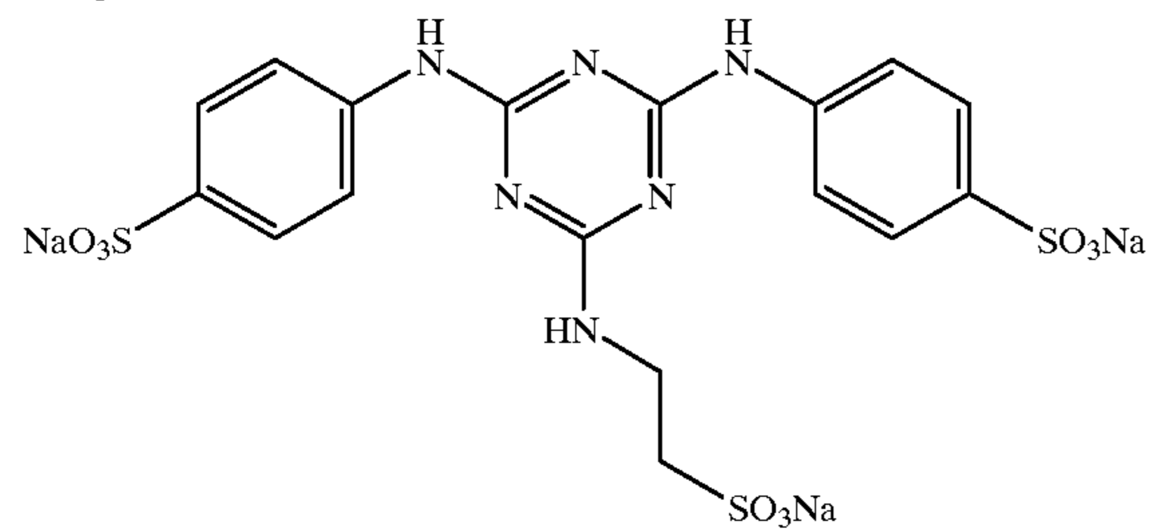
Compound 11:
