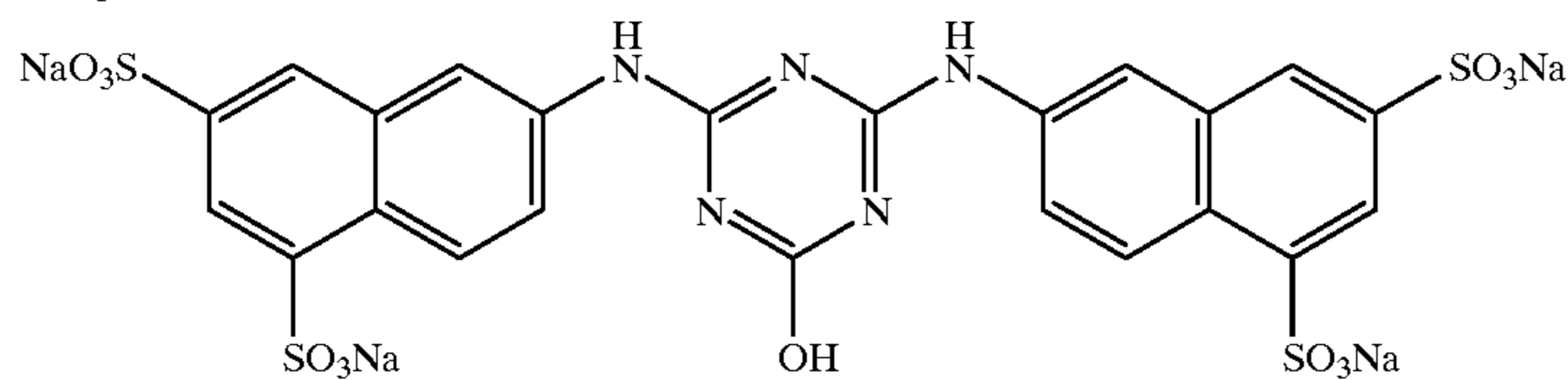
Compound 4:
