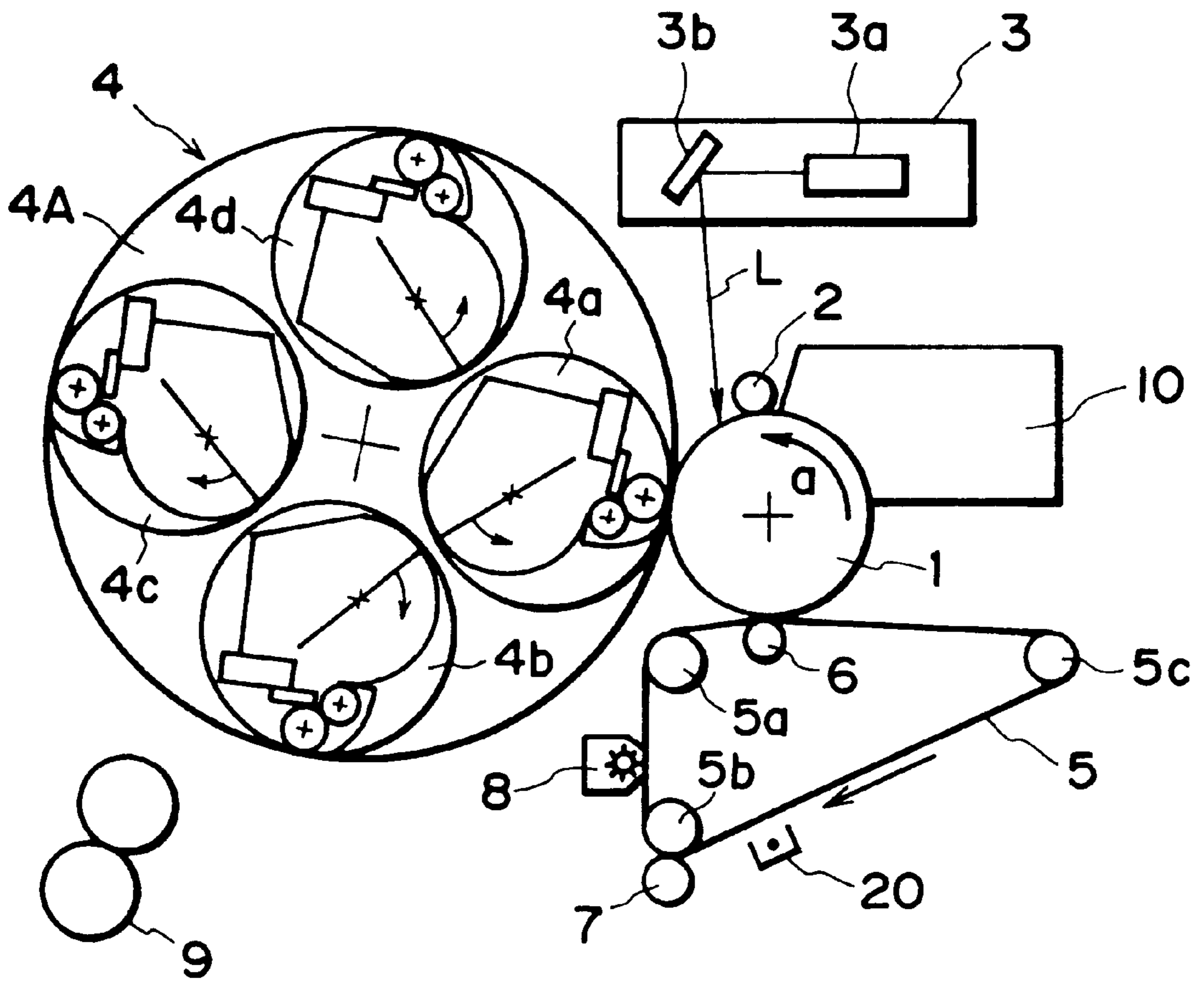
FIG. 8 PRIOR ART
