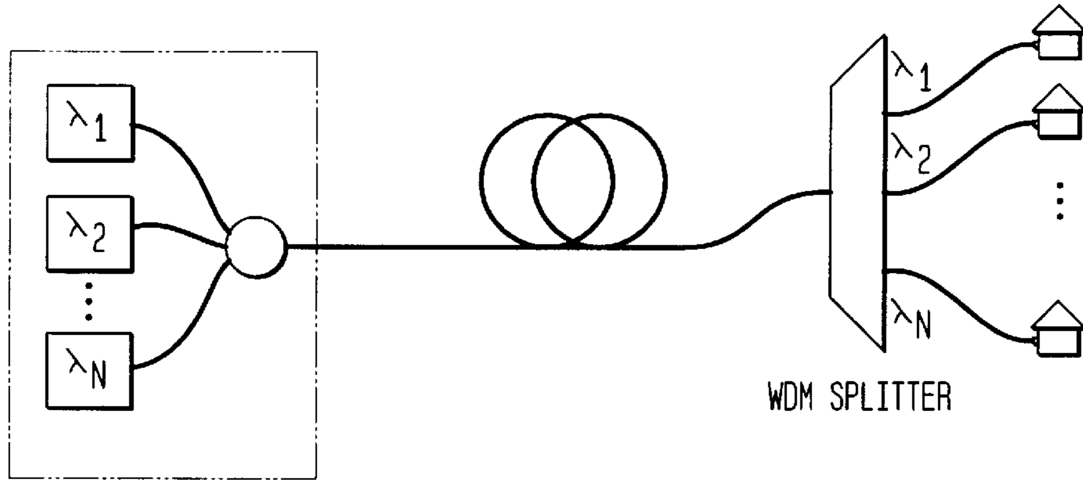
FIG. 9 (PRIOR ART)
