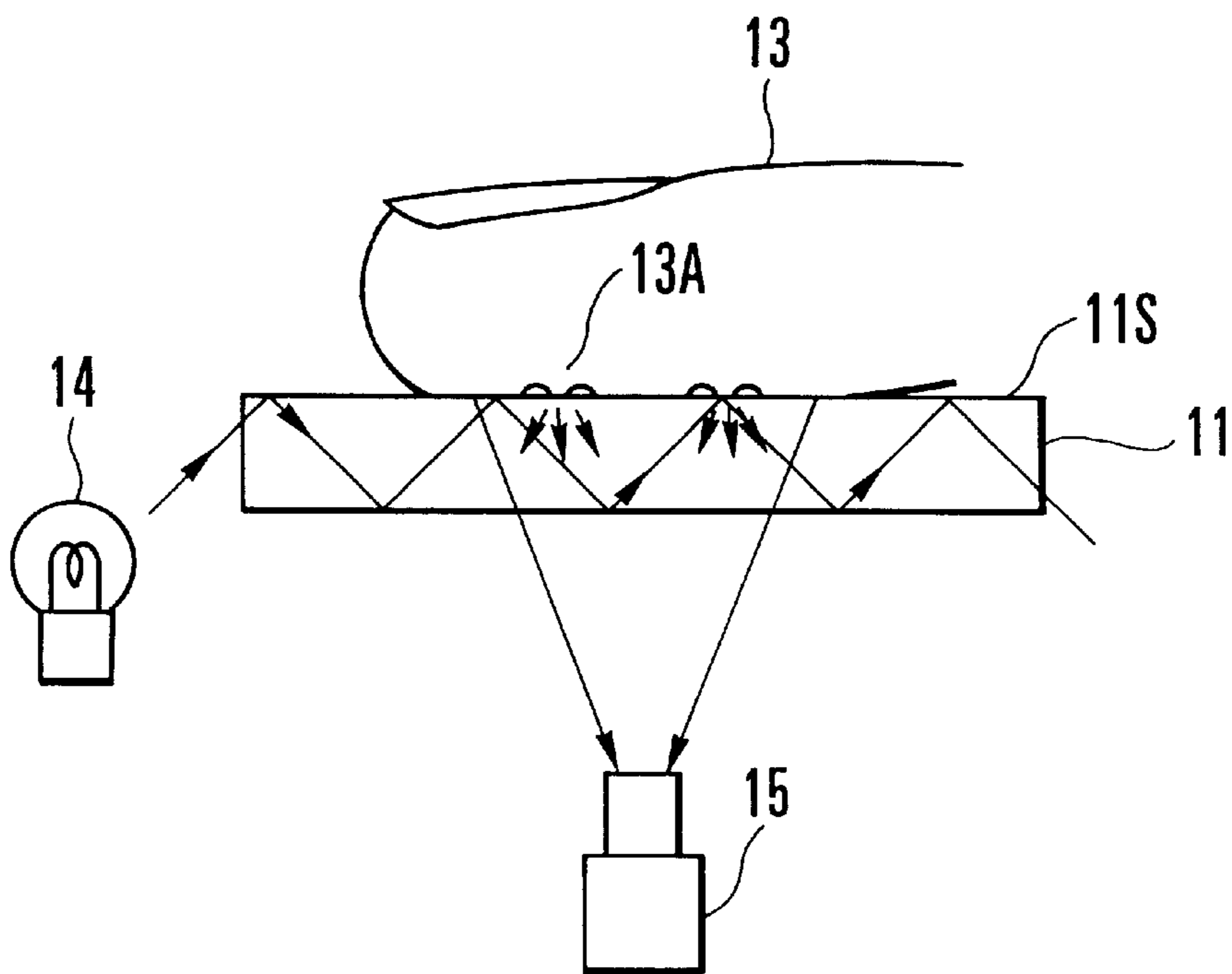
FIG. 4 PRIOR ART
