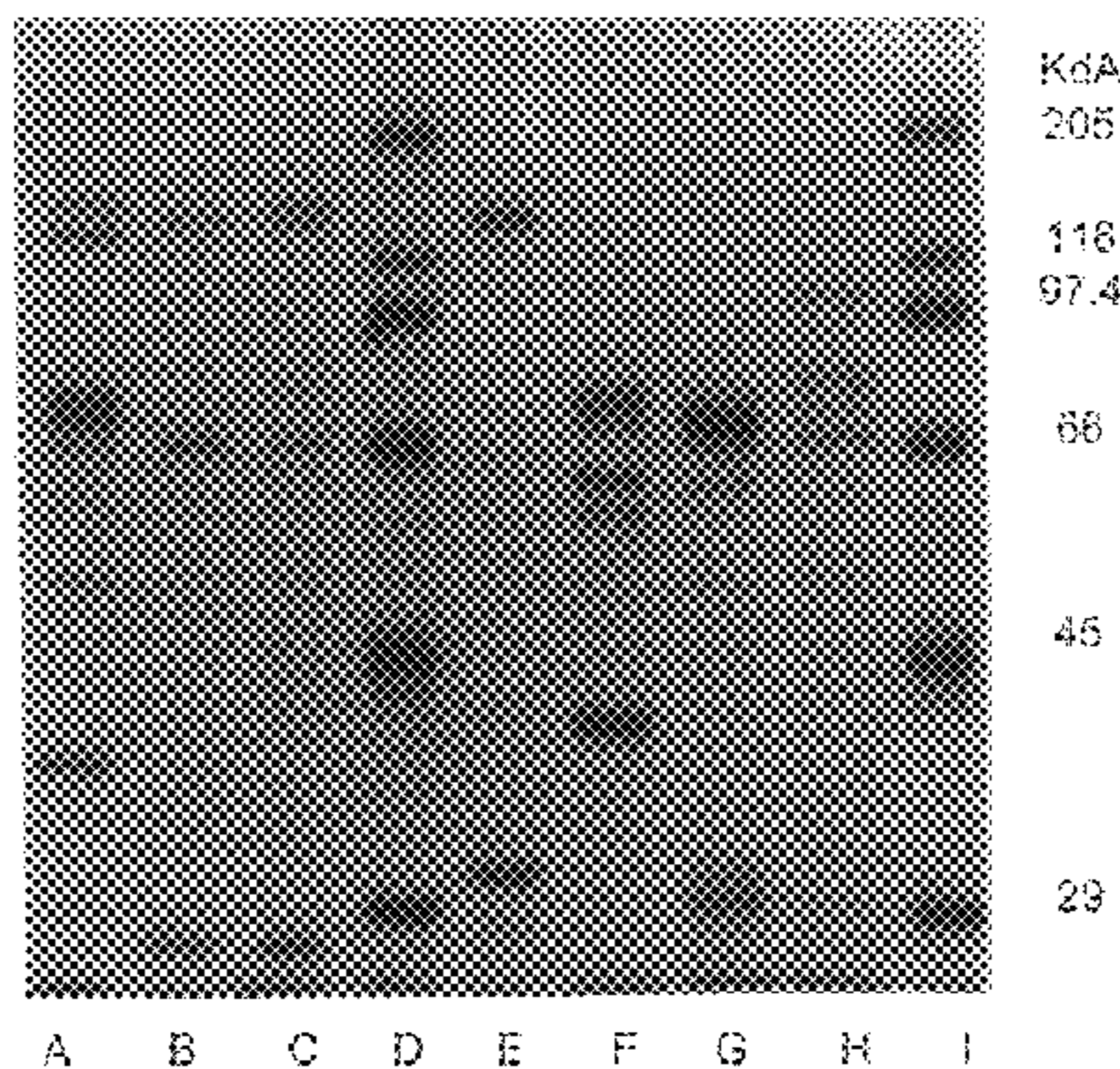
A. Bacillus thuringiensis PS192N1 B. Bacillus thuringiensis PS123D1 C. Bacillus thuringiensis PS71M3 D. Protein Standard E. Bacillus thuringiensis PS201T6 F. Bacillus thuringiensis PS201L1 G. Bacillus thuringiensis PS196S1 H. Bacillus thuringiensis PS92J I. Protein Standard
