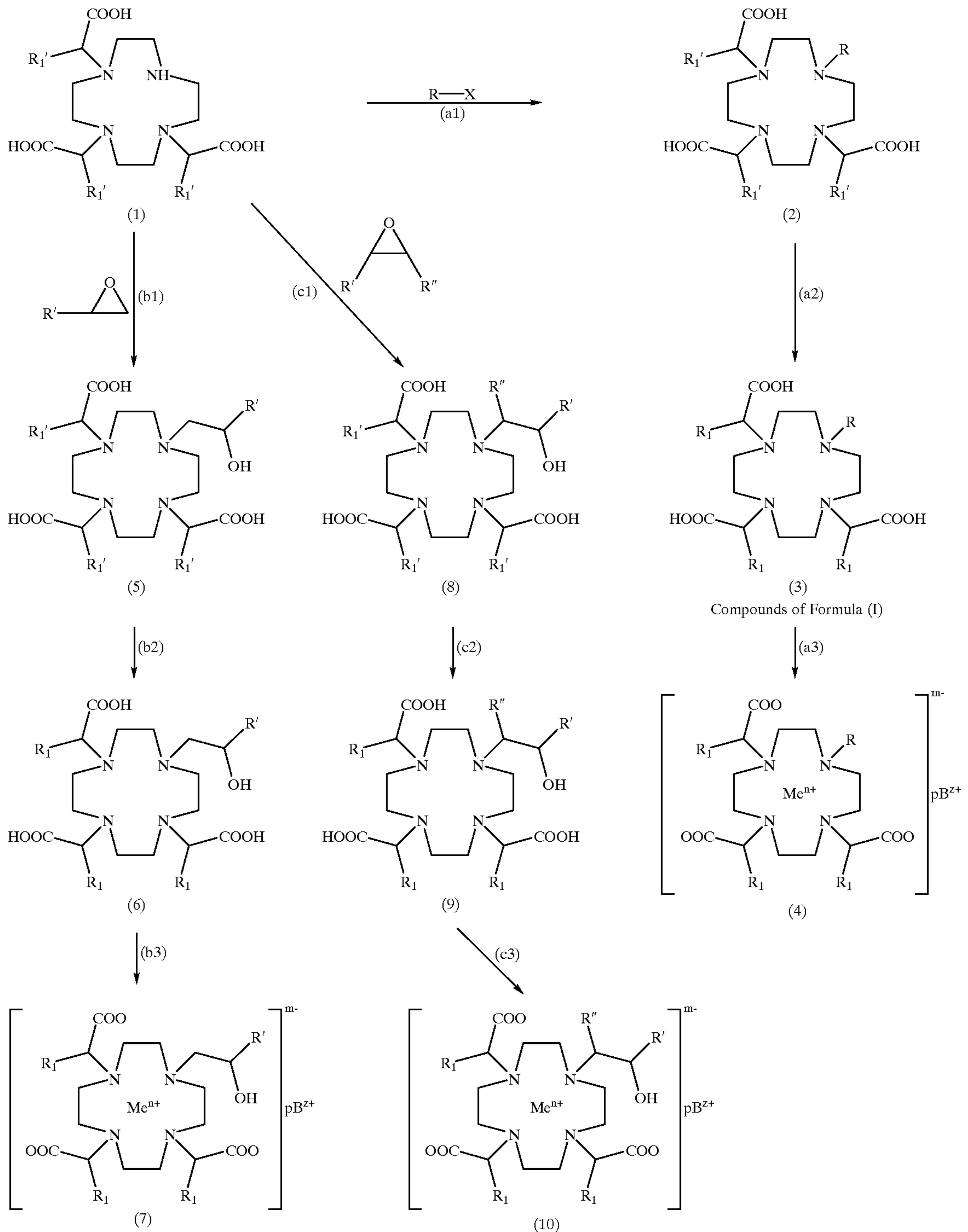
SCHEME 1
