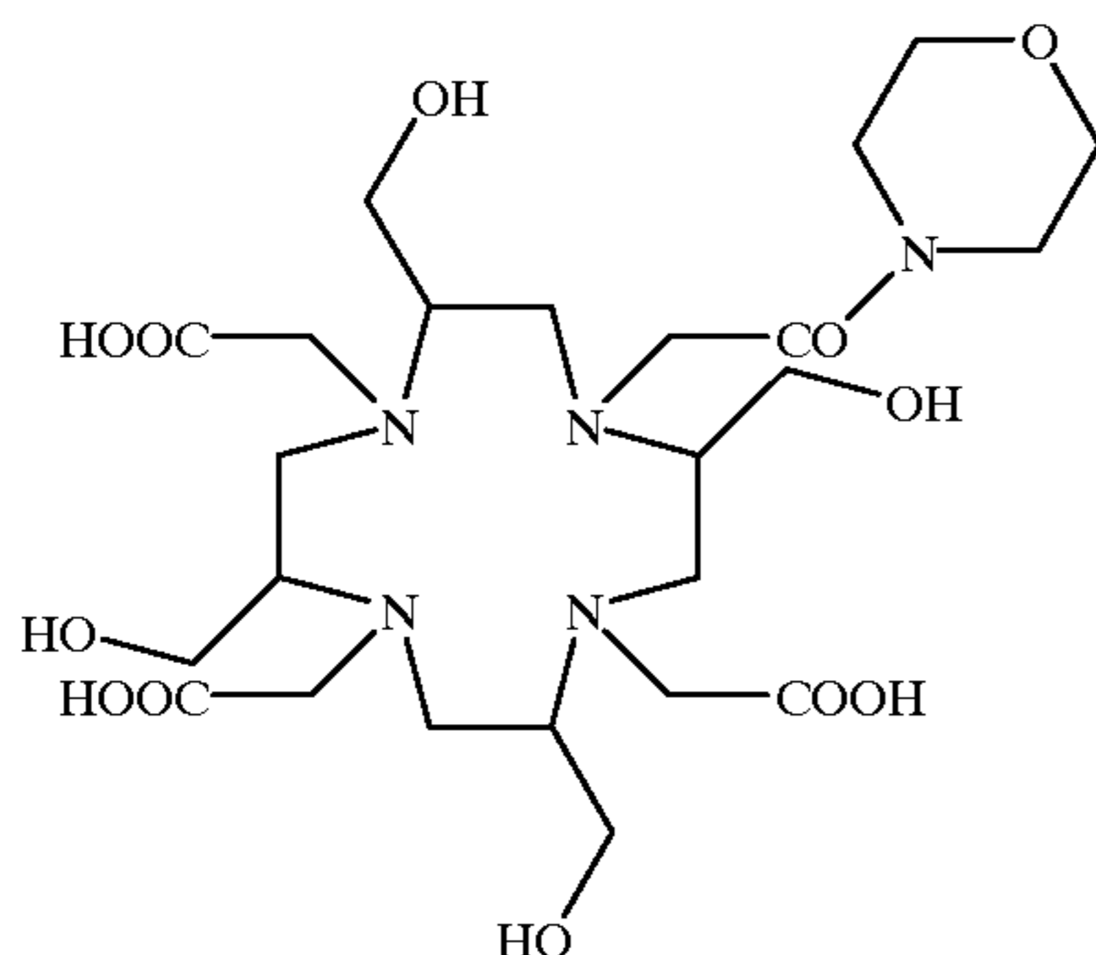
Compound 8 (Example 4)
