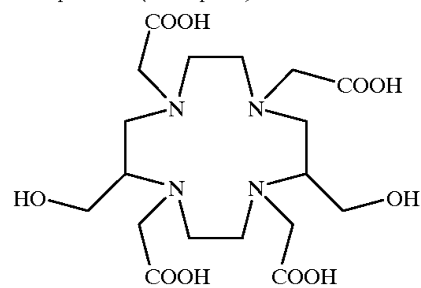
Compound 4 (Example 4)
