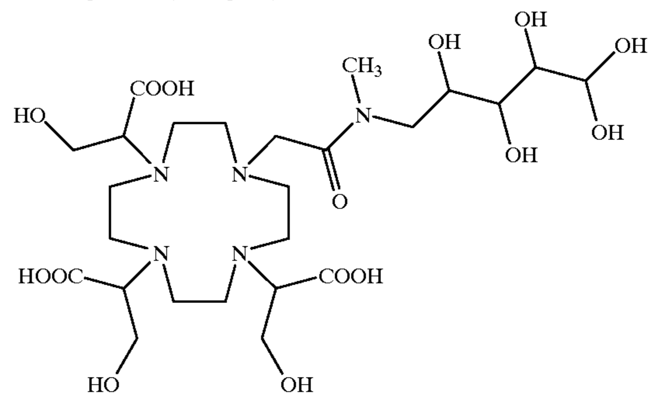
Compound 6 (Example 2)
