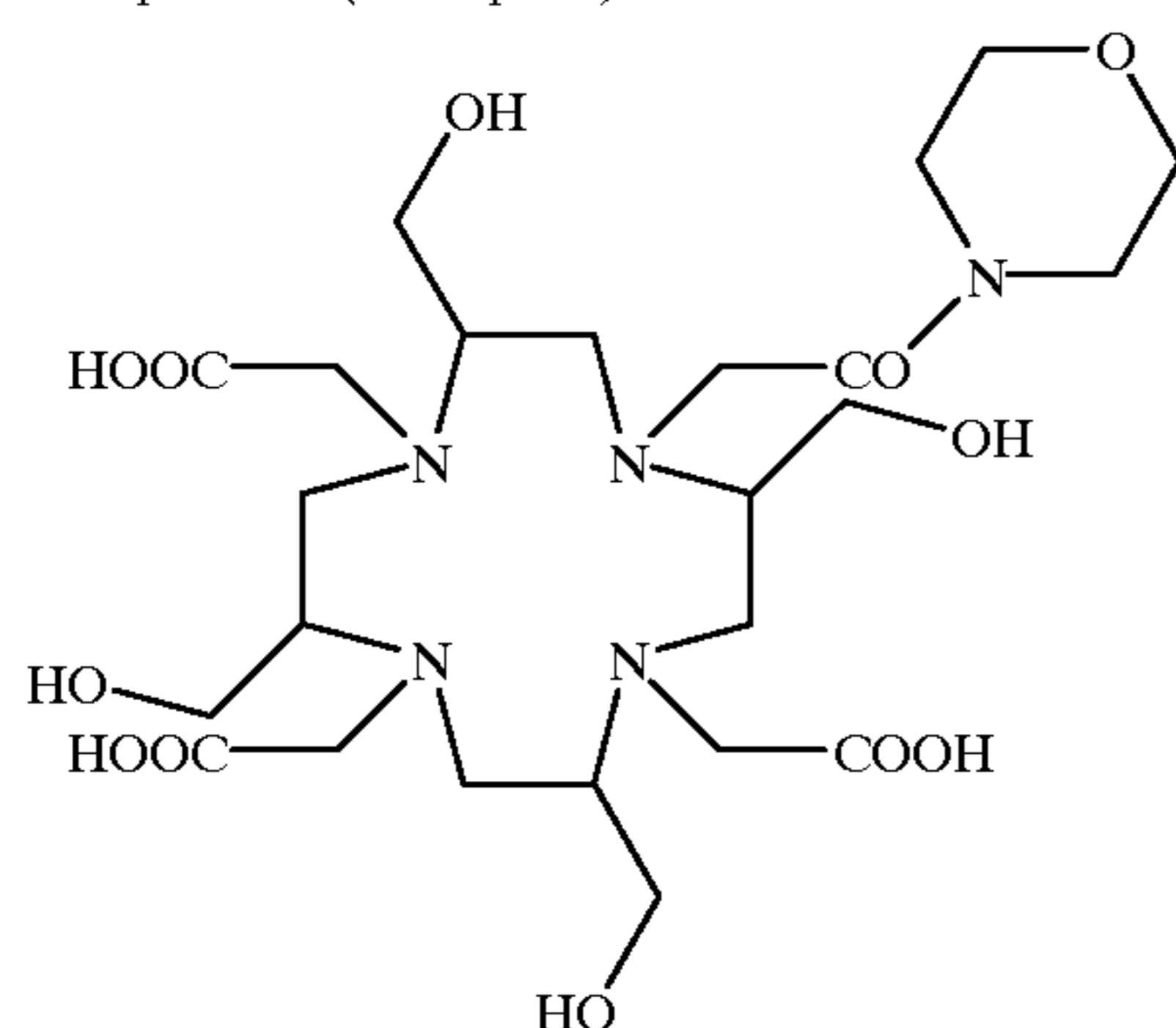
Compound 8 (Example 4)
