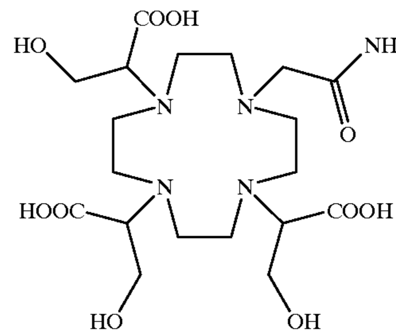
Compound 3 (Example 3)
