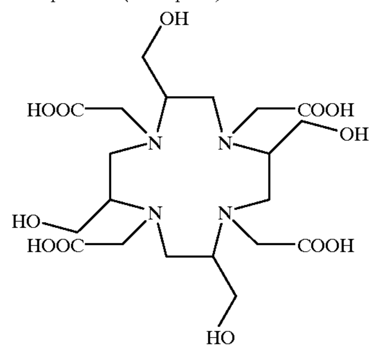
Compound 5 (Example 1)
