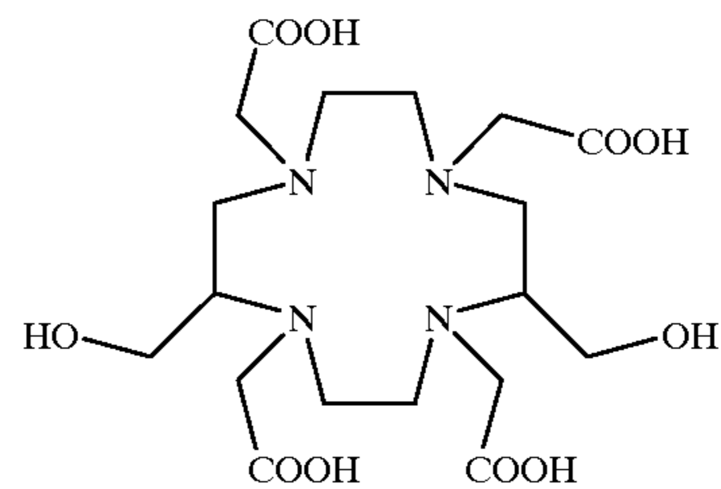
Compound 4 (Example 4)
