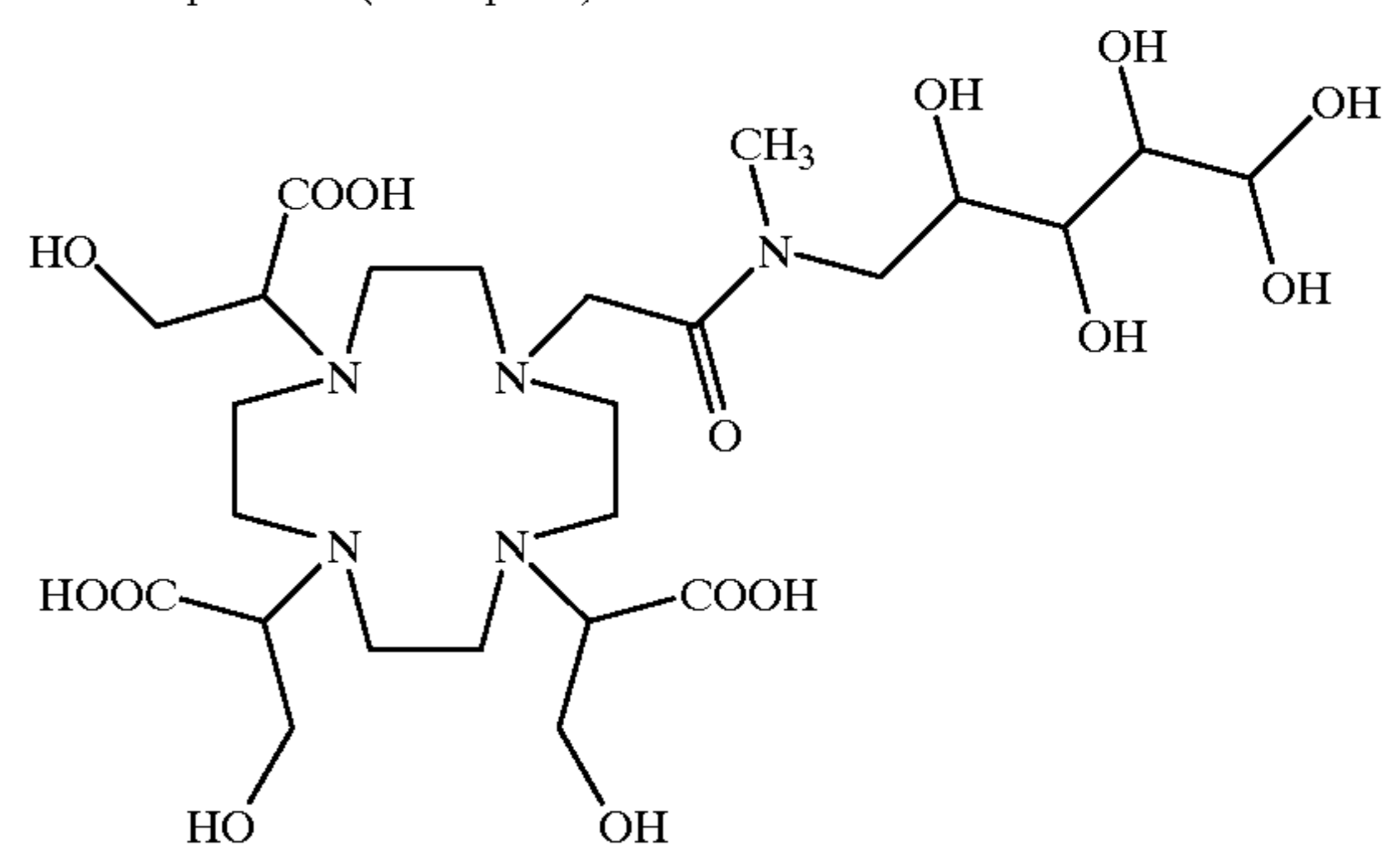
Compound 6 (Example 2)
