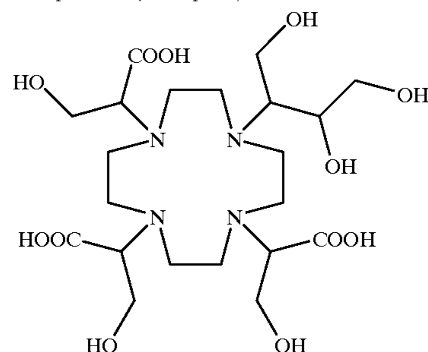
Compound 6 (Example 2)
