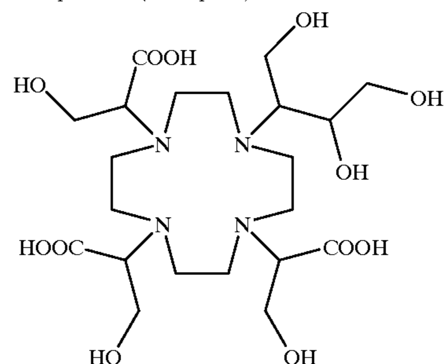
Compound 6 (Example 2)
