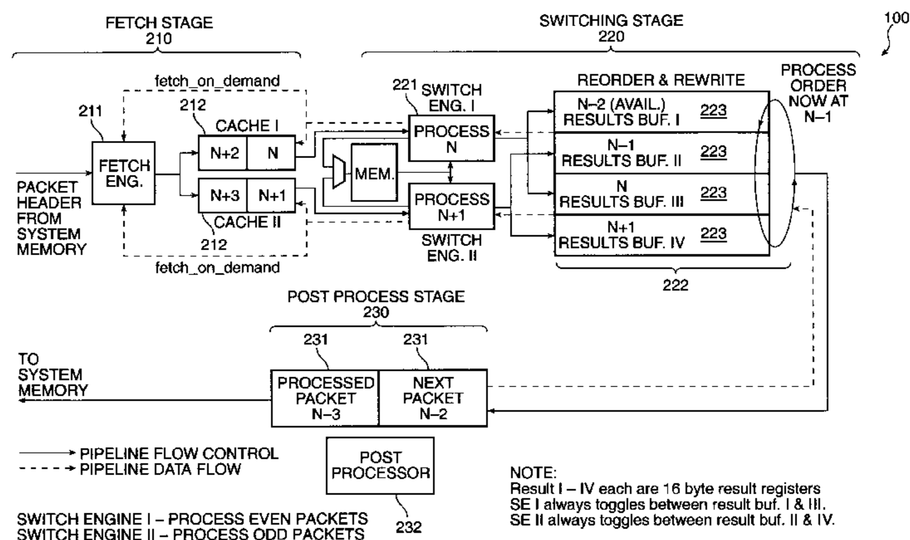
DUAL ISSUE SWITCH: PACKETS AND CONTROL FLOW
