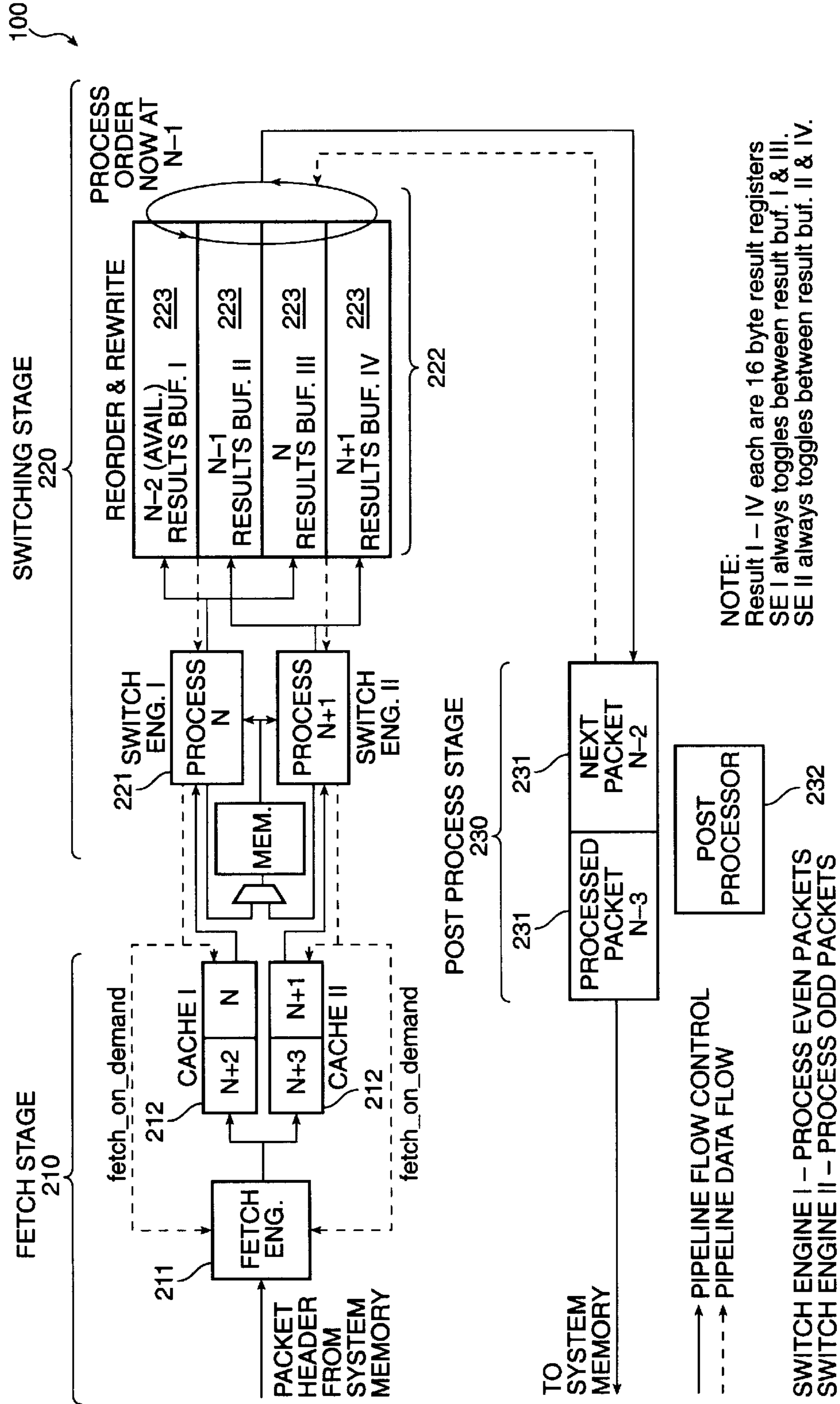
DUAL ISSUE SWITCH: PACKETS AND CONTROL FLOW
